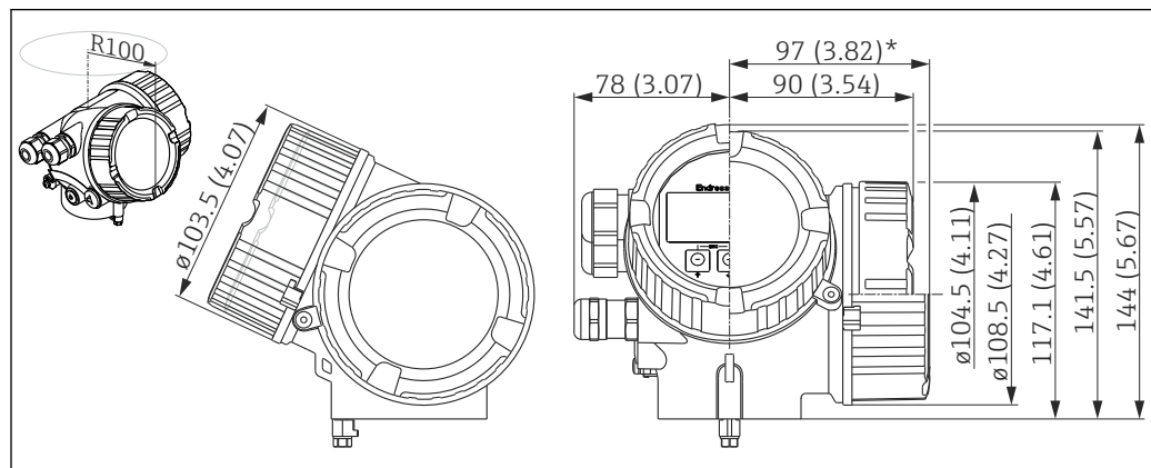
17 Housing GT20 (Alu coated); Dimensions in mm (in)
