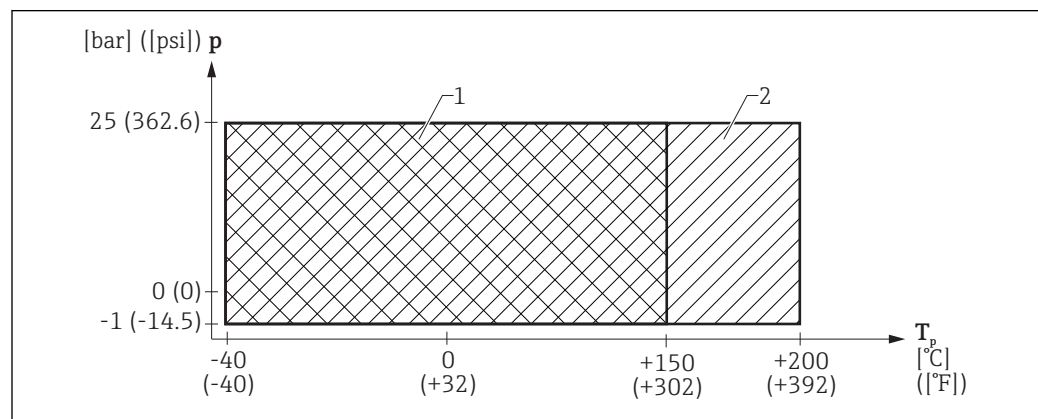
14 FMR62: Permitted range for process temperature and process pressure of version with flush mount PTFE antenna (feature 070)
