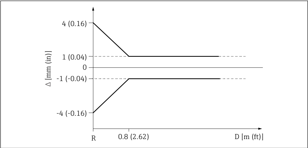
10 Maximum measured error in near-range applications
