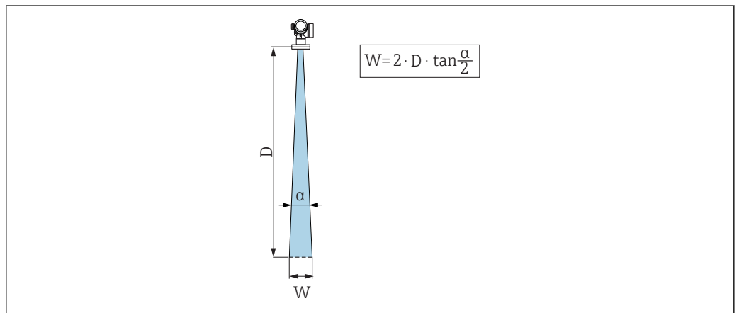
11 Relationship between beam angle \alpha , distance D and beamwidth diameter W
