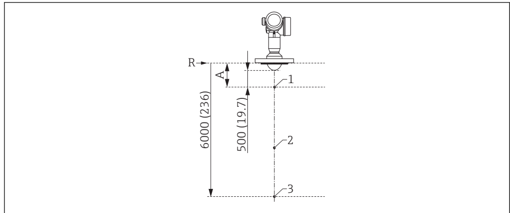
25 Points of the 3-point linearity protocol; engineering unit: mm (in)
