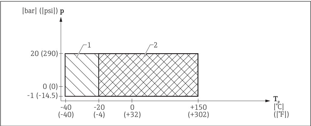
12 FMR62: Permitted range for process temperature and process pressure of version with integrated antenna, PEEK, 150° (feature 070) 1 Feature 90, seal: A5, FKM Viton GLT 2 Feature 90, seal: C1, FFKM Kalrez
