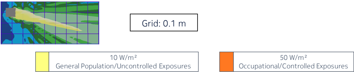
Figure 6 – Side view of the power density for the time-averaged actual maximum transmitted power of 0.178 W and the beam oriented in azimuth = 0° & elevation = +15°
