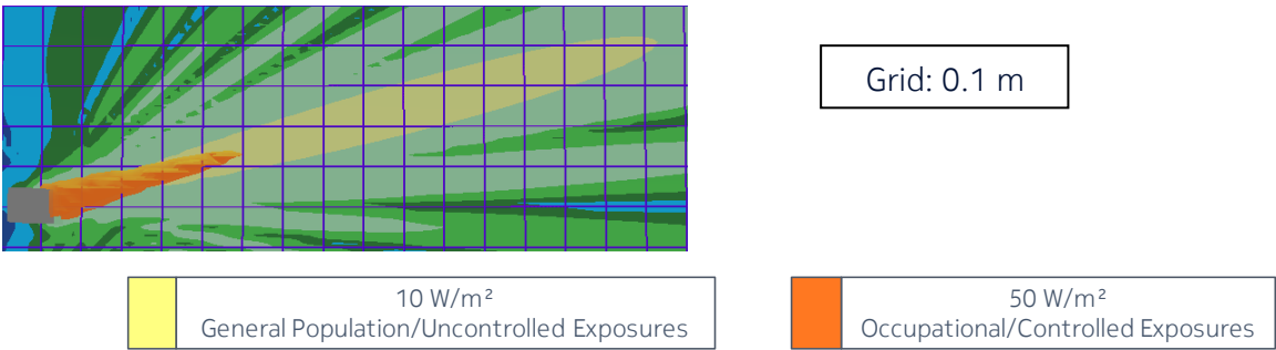
Figure 7 – Side view of the power density for the time-averaged maximum transmitted power of 0.713 W and the beam oriented in azimuth = 0° & elevation = -15°
