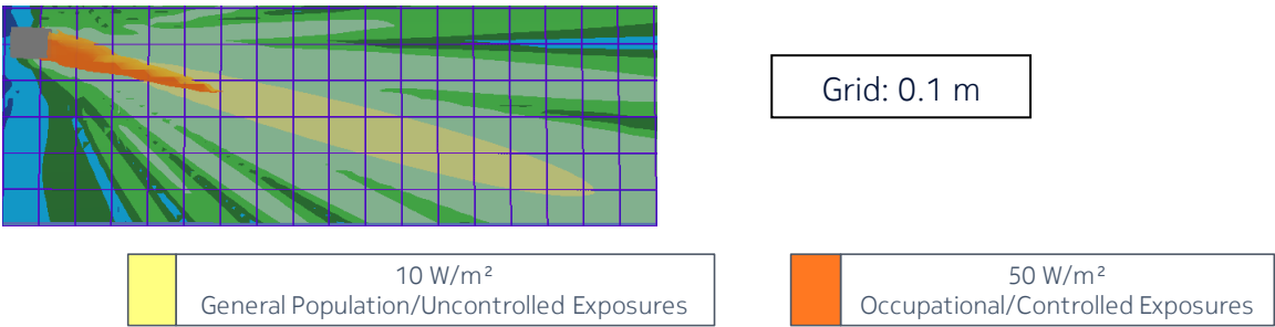
Figure 5 – Side view of the power density for the time-averaged maximum transmitted power of 0.713 W and the beam oriented in azimuth = 0° & elevation = +15°
