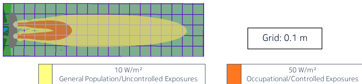
Figure 3 – Top view of the power density for the time-averaged maximum transmitted power of 0.713 W and the beam oriented in azimuth = 0° & elevation = 0°
