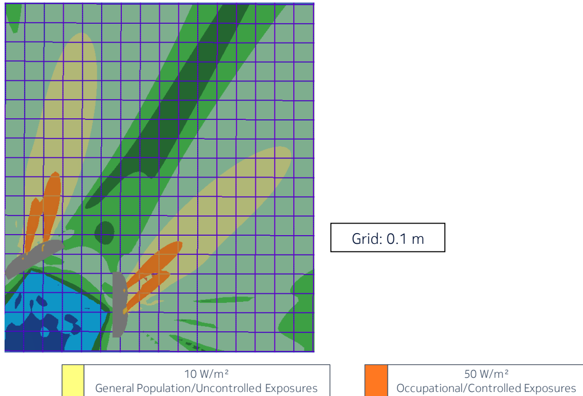
Figure 9 – Top view of the power density for the time-averaged maximum transmitted power of 0.713 W and the beam oriented in azimuth = -45°/+45° & elevation = 0°
