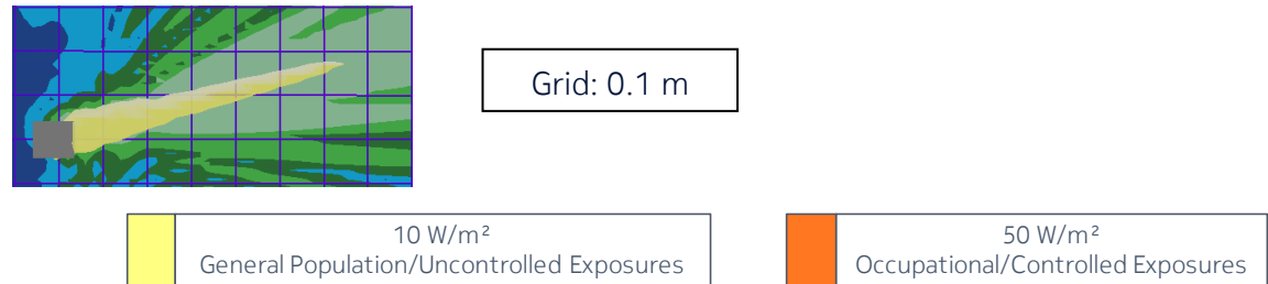
Figure 8 – Side view of the power density for the time-averaged actual maximum transmitted power of 0.178 W and the beam oriented in azimuth = 0° & elevation = -15°
