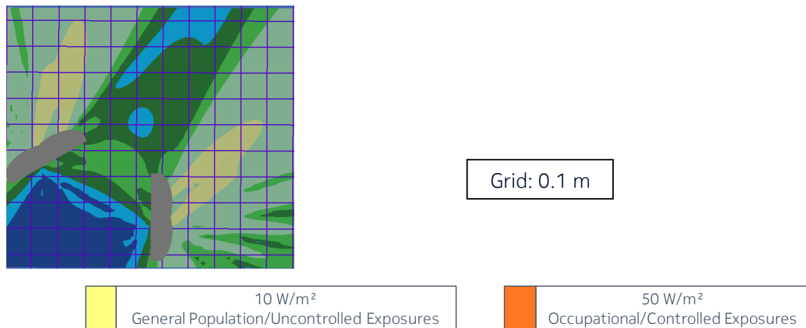
Figure 10 – Top view of the power density for the time-averaged actual maximum transmitted power of 0.178 W and the beam oriented in azimuth = -45°/+45° & elevation = 0°
