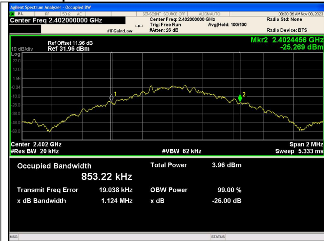
GFSK DH5 Channel 0
