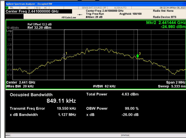
GFSK DH5 Channel 39
