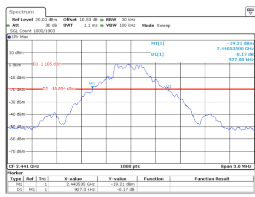
GFSK_Middle 0.927 MHz
