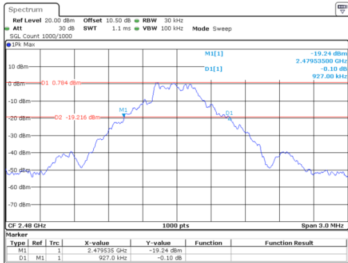
GFSK_High 0.927 MHz
