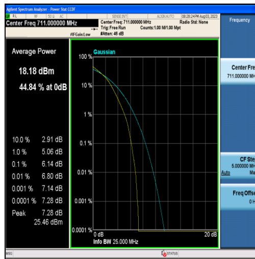
Band12-10MHz-16QAM-23130-50RB#0
