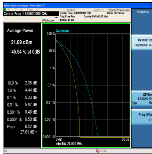
Band25-20MHz-QPSK-26140-100RB#0
