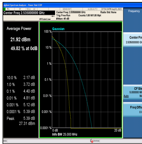
Band7-20MHz-QPSK-21100-100RB#0
