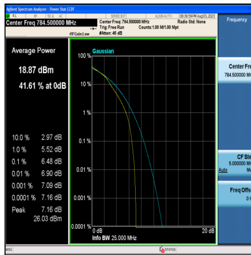
Band13-5MHz-16QAM-23255-25RB#0
