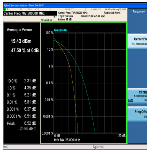
Band12-10MHz-QPSK-23095-50RB#0
