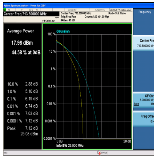
Band12-5MHz-16QAM-23155-25RB#0
