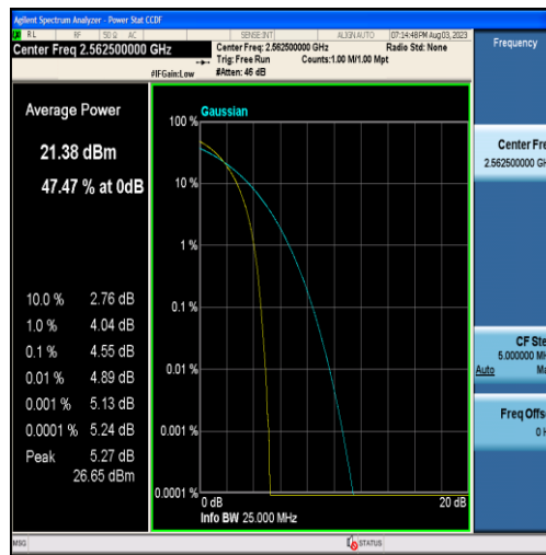
Band7-15MHz-16QAM-21375-75RB#0
