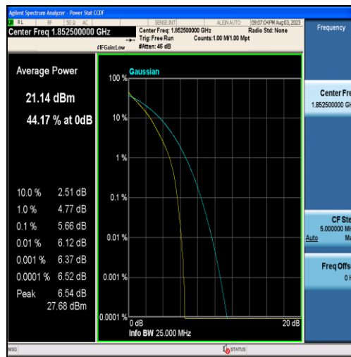
Band25-5MHz-QPSK-26065-25RB#0
