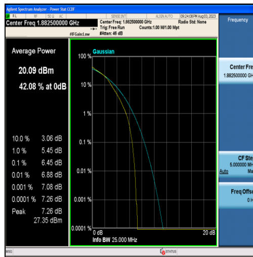
Band25-15MHz-16QAM-26365-75RB#0
