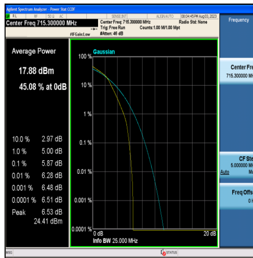
Band12-1.4MHz-16QAM-23173-6RB#0
