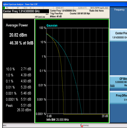
Band25-1.4MHz-QPSK-26683-6RB#0
