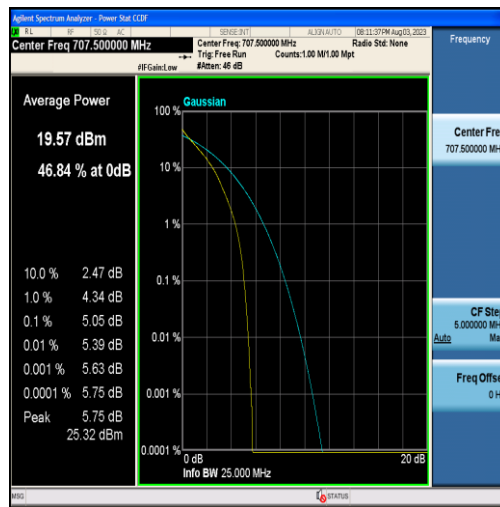
Band12-3MHz-QPSK-23095-15RB#0
