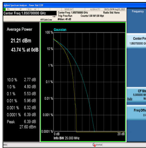
Band25-1.4MHz-QPSK-26047-6RB#0
