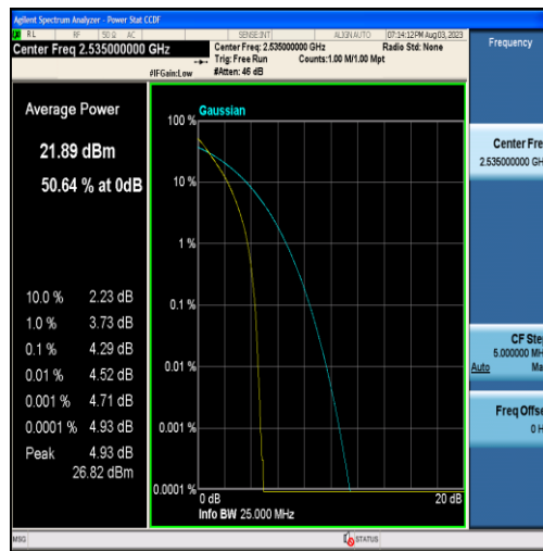
Band7-15MHz-QPSK-21100-75RB#0
