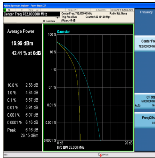
Band13-5MHz-QPSK-23230-25RB#0
