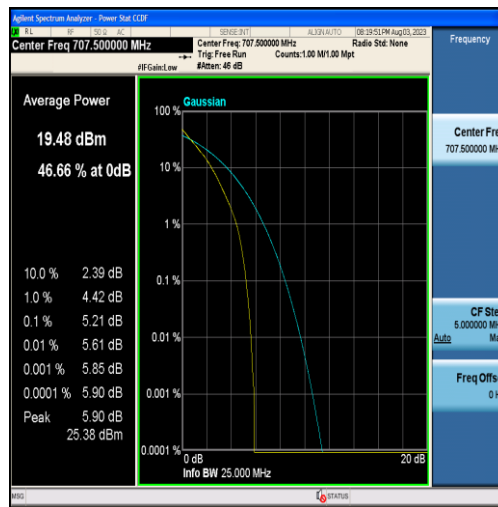
Band12-5MHz-QPSK-23095-25RB#0
