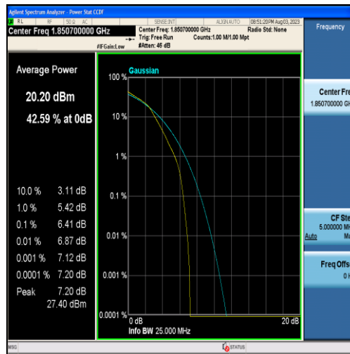
Band25-1.4MHz-16QAM-26047-6RB#0
