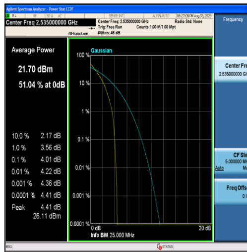
Band7-5MHz-QPSK-21100-25RB#0
