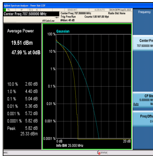
Band12-1.4MHz-QPSK-23095-6RB#0
