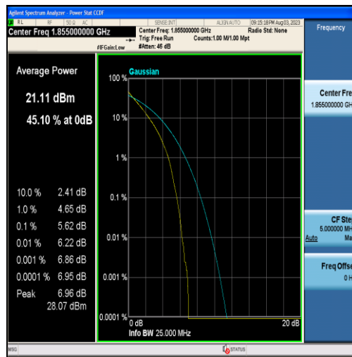
Band25-10MHz-QPSK-26090-50RB#0
