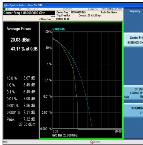
Band25-1.4MHz-16QAM-26365-6RB#0
