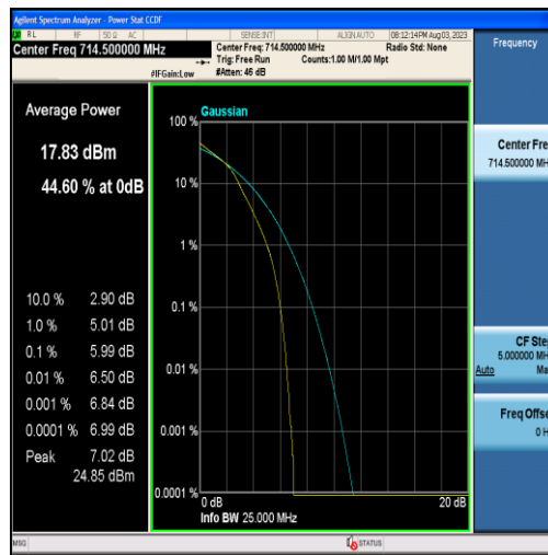
Band12-3MHz-16QAM-23165-15RB#0
