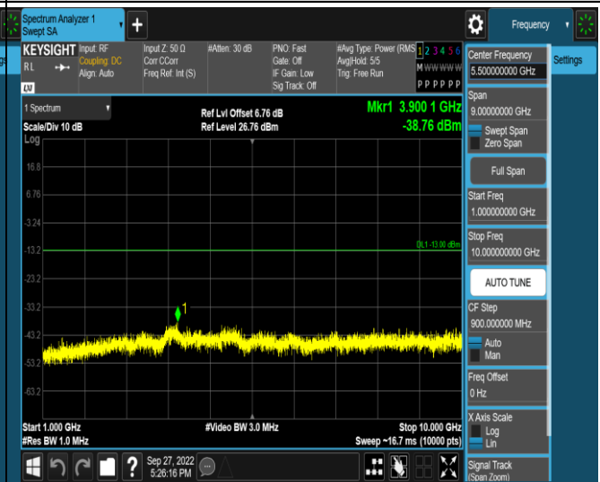
Band17-10MHz-16QAM-23800-1RB#0-Range2:1000~ 10000MHz
