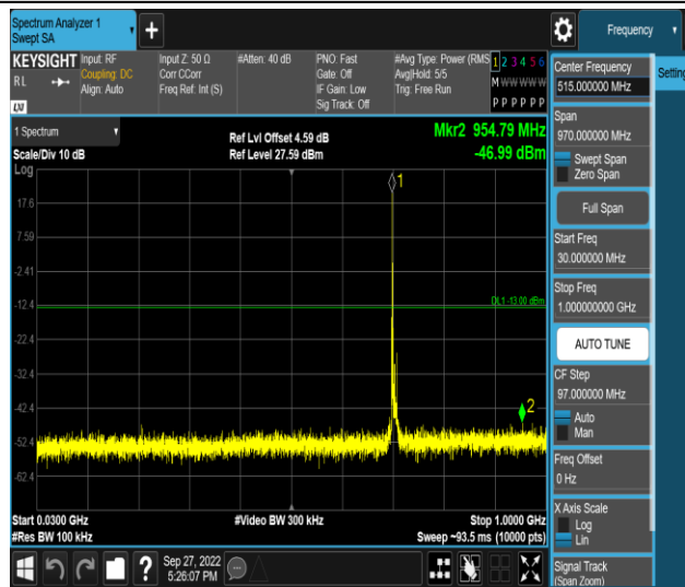
Band17-10MHz-16QAM-23800-1RB#0-Range1:30 ~1000MHz
