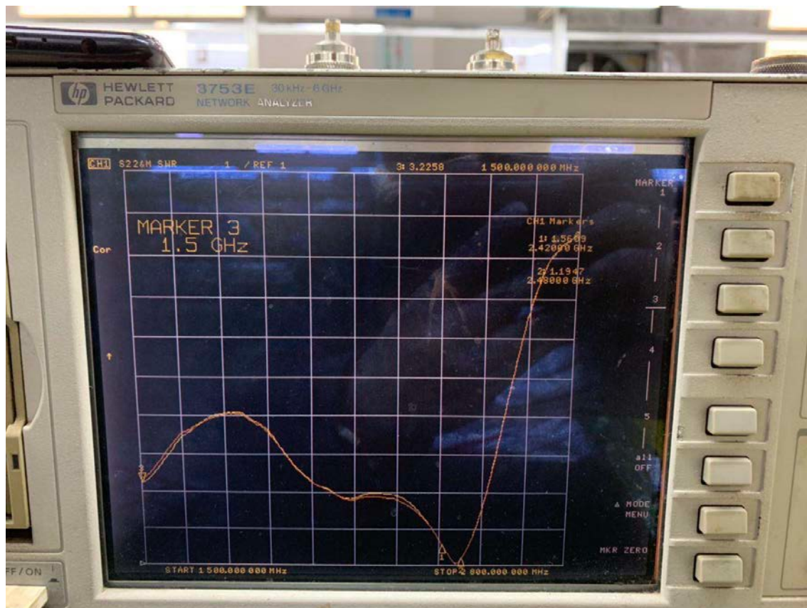
BT antenna VSWR graph
