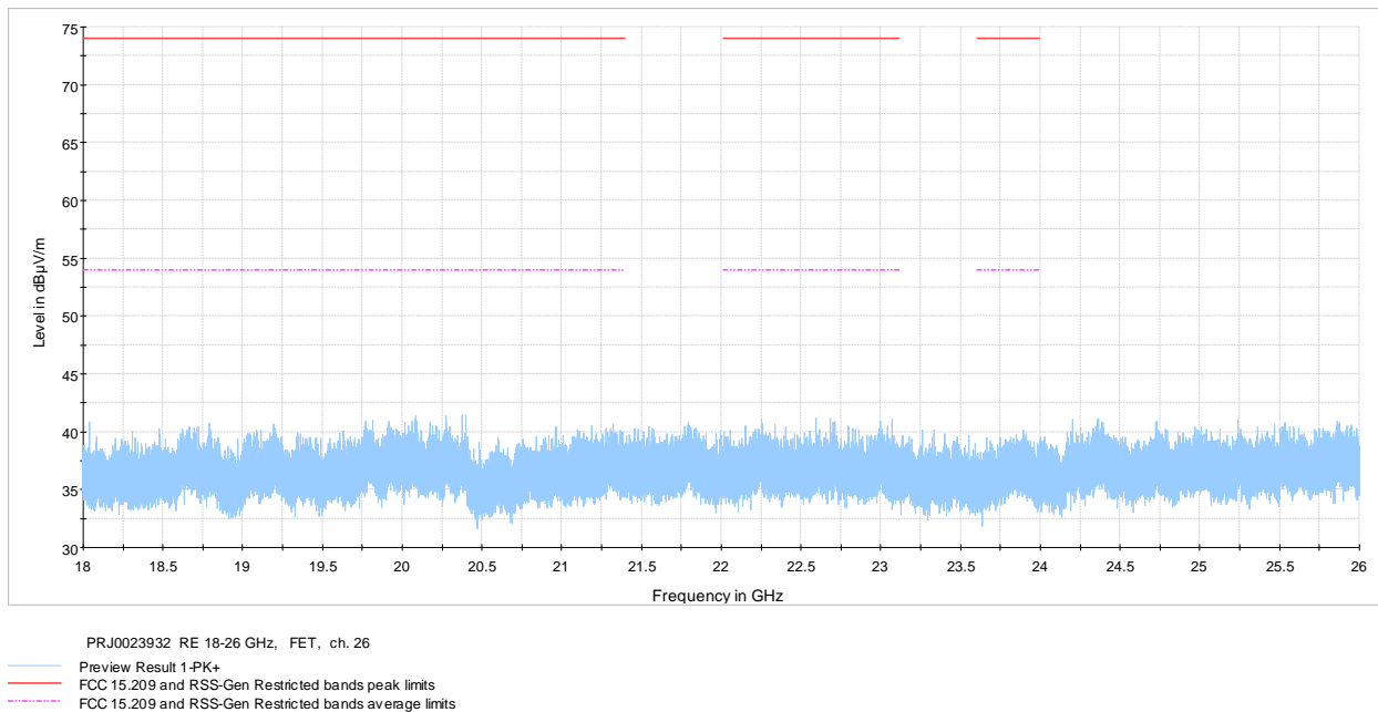
Figure 8.7-9: Radiated spurious emissions 18-26 GHz high ch.
