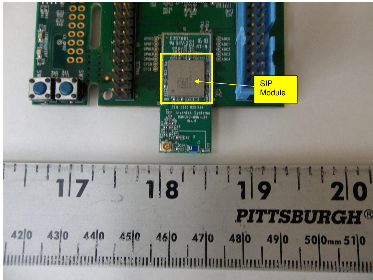
Figure 2. Close Up of ISM4343-WBM-L151 module
