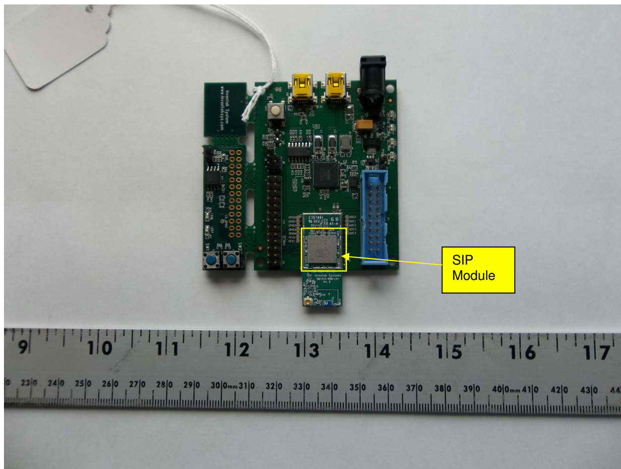
Figure 1. Front of Evaluation Board with ISM4343-WBM-L151 module (Yellow)
