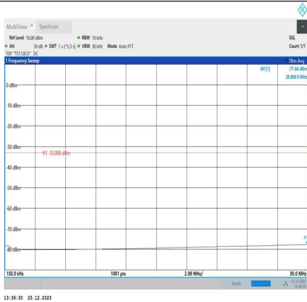
66-66-10MHz-10MHz-16QAM-16QAM-132523-132622-1RB#0-1RB#49-0.15~30MHz-PASS
