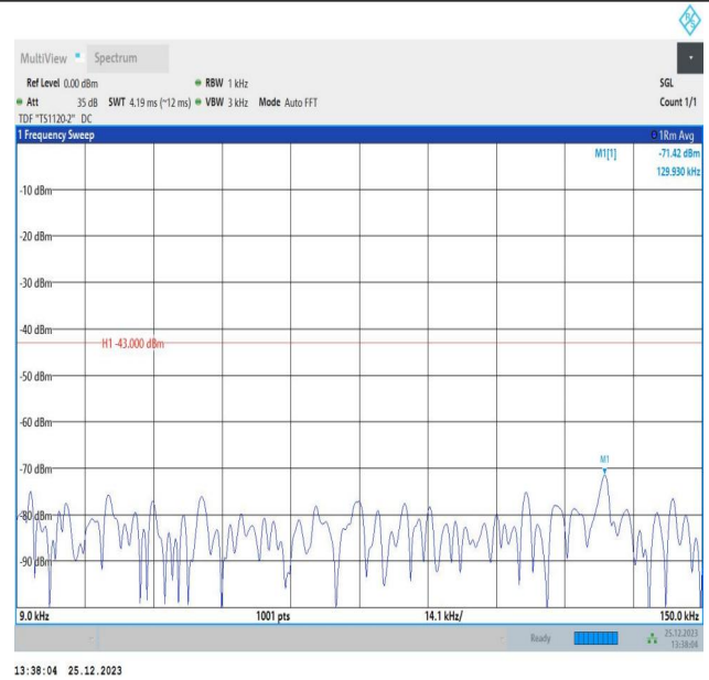
66-66-10MHz-10MHz-16QAM-16QAM-132523-132622-50RB#0-50RB#0-0.009~0.15MHz-PASS
