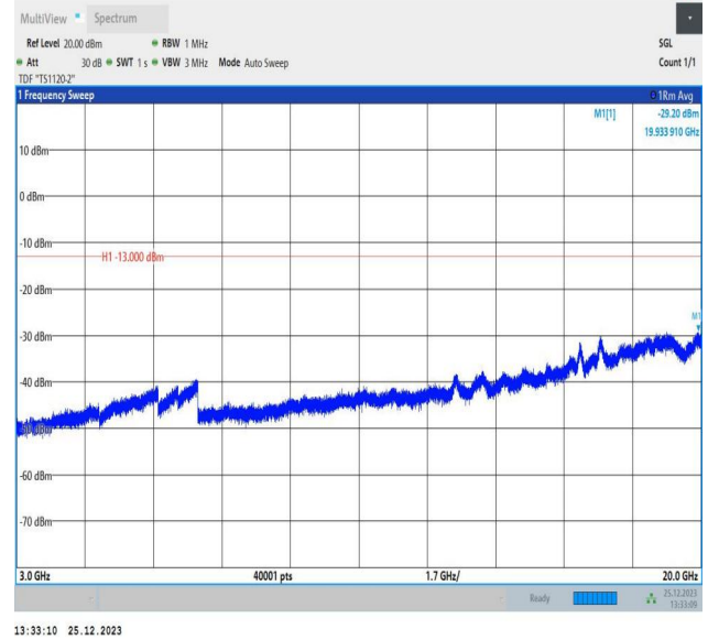
66-66-10MHz-10MHz-16QAM-16QAM-132523-132622-1RB# 0-ORB#0-3000~20000MHz-PASS
