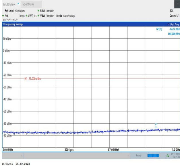
66-66-5MHz-15MHz-QPSK-QPSK-132002-132095-1RB#24- ORB#0-30~1000MHz-PASS
