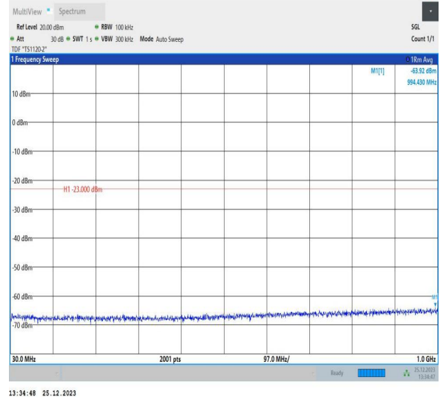
66-66-10MHz-10MHz-16QAM-16QAM-132523-132622-1RB# 49-ORB#0-30~1000MHz-PASS
