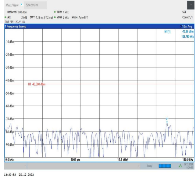
66-66-10MHz-10MHz-16QAM-16QAM-132022-132121-1RB#0-1RB#49-0.009~0.15MHz-PASS
