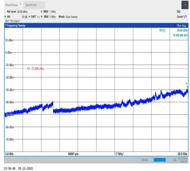
66-66-10MHz-10MHz-16QAM-16QAM-132523-132622-1RB# 0-1RB#49-3000~20000MHz-PASS
