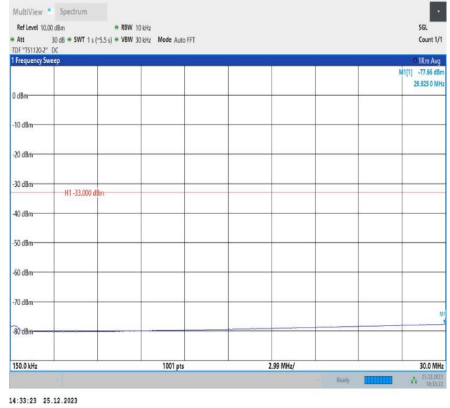
66-66-5MHz-15MHz-QPSK-QPSK-132002-132095-1RB#0-0R B#0-0.15~30MHz-PASS
