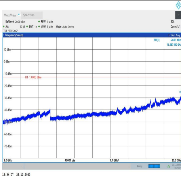
66-66-10MHz-10MHz-QPSK-QPSK-132523-132622-1RB#49 -ORB#0-3000~20000MHz-PASS
