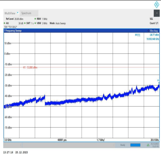
66-66-10MHz-10MHz-16QAM-16QAM-132373-132472-1RB# 49-ORB#0-3000~20000MHz-PASS
