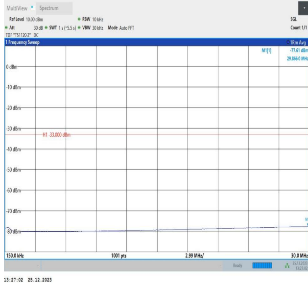
66-66-10MHz-10MHz-16QAM-16QAM-132373-132472-1RB# 49-ORB#0-0.15~30MHz-PASS
