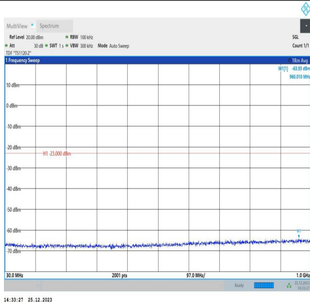
66-66-5MHz-15MHz-QPSK-QPSK-132002-132095-1RB#0-0 RB#0-30~1000MHz-PASS
