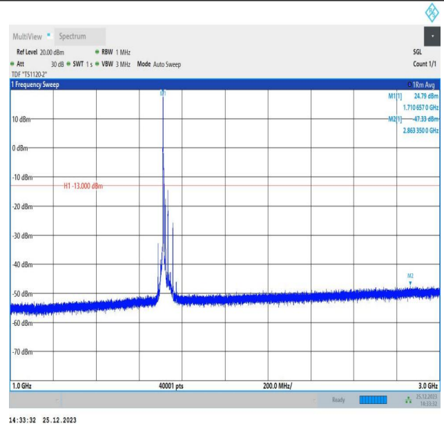
66-66-5MHz-15MHz-QPSK-QPSK-132002-132095-1RB#0-0R B#0-1000~3000MHz-PASS
