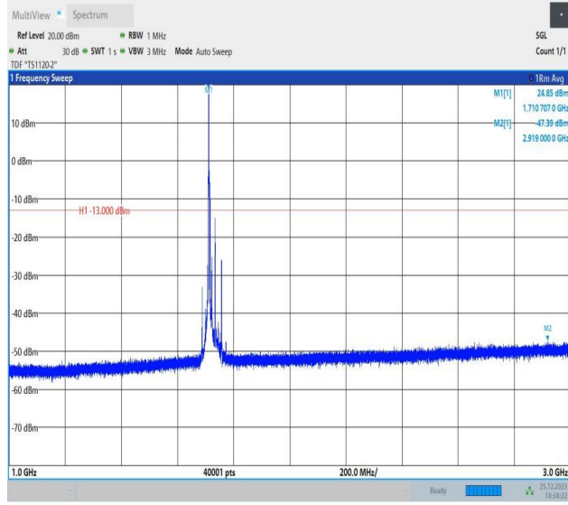
66-66-5MHz-15MHz-16QAM-16QAM-132002-132095-1RB#0-0RB#0-1000~3000MHz-PASS
