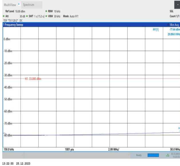
66-66-10MHz-10MHz-16QAM-16QAM-132022-132121-50RB #0-50RB#0-0.15~30MHz-PASS
