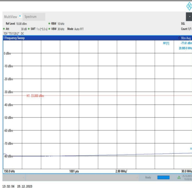
66-66-10MHz-10MHz-16QAM-16QAM-132523-132622-1RB#0-ORB#0-0.15~30MHz-PASS
