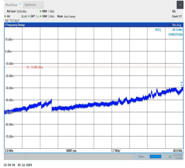
66-66-10MHz-10MHz-16QAM-16QAM-132373-132472-1RB# 0-1RB#49-3000~20000MHz-PASS
