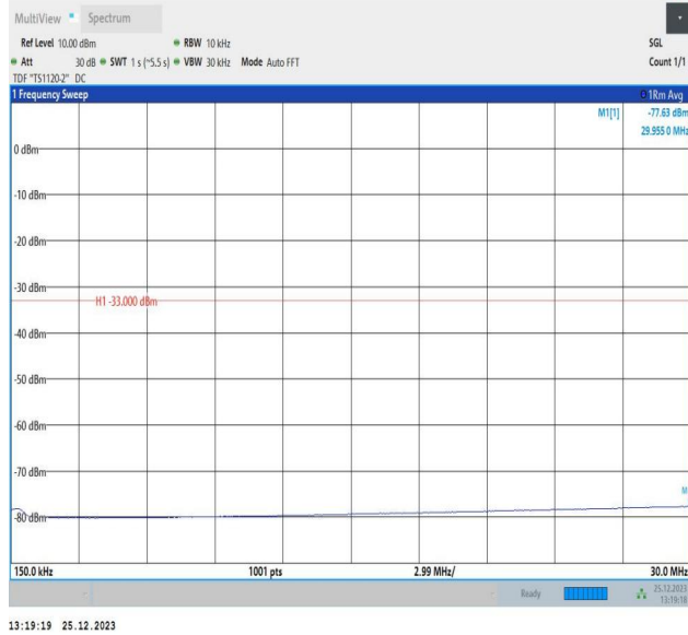
66-66-10MHz-10MHz-16QAM-16QAM-132022-132121-1RB# 49-ORB#0-0.15~30MHz-PASS
