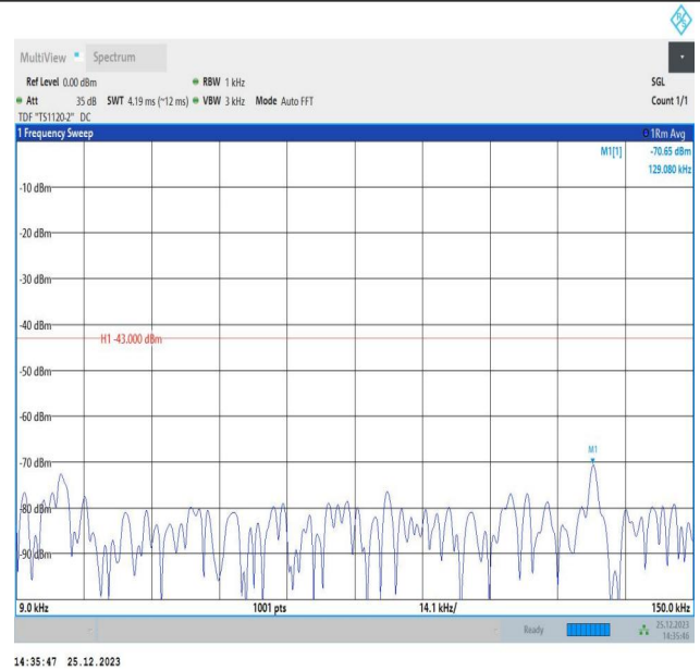
66-66-5MHz-15MHz-16QAM-16QAM-132002-132095-1RB#2 4-ORB#0-0.009~0.15MHz-PASS
