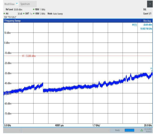
66-66-5MHz-15MHz-16QAM-16QAM-132002-132095-1RB#0-0RB#0-3000~20000MHz-PASS
