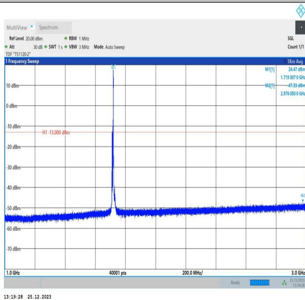
66-66-10MHz-10MHz-16QAM-16QAM-132022-132121-1RB# 49-ORB#0-1000~3000MHz-PASS
