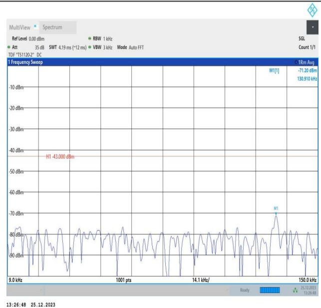
66-66-10MHz-10MHz-16QAM-16QAM-132373-132472-1RB# 49-ORB#0-0.009~0.15MHz-PASS
