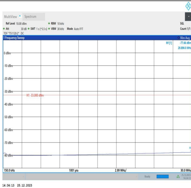
66-66-5MHz-15MHz-16QAM-16QAM-132002-132095-1RB#0 -ORB#0-0.15~30MHz-PASS
