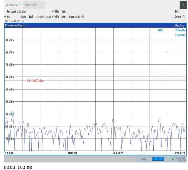
66-66-10MHz-10MHz-16QAM-16QAM-132523-132622-1RB#0-1RB#49-0.009~0.15MHz-PASS
