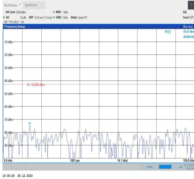
66-66-10MHz-10MHz-QPSK-QPSK-132523-132622-1RB#0-1RB#49-0.009~0.15MHz-PASS
