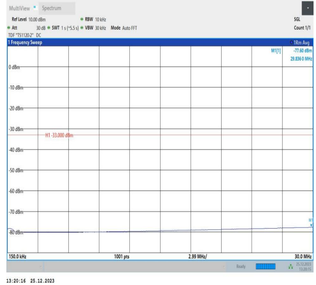
66-66-10MHz-10MHz-QPSK-QPSK-132022-132121-1RB#0-1RB#49-0.15~30MHz-PASS
