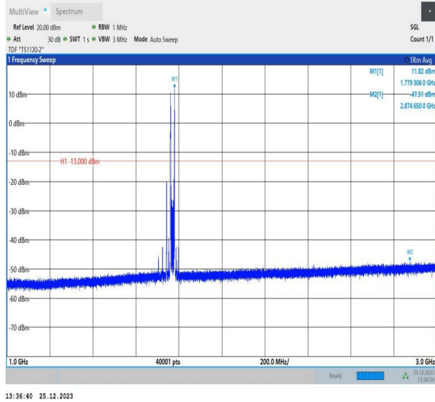
66-66-10MHz-10MHz-16QAM-16QAM-132523-132622-1RB# 0-1RB#49-1000~3000MHz-PASS
