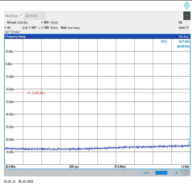
66-66-10MHz-10MHz-16QAM-16QAM-132022-132121-1RB#0-1RB#49-30~1000MHz-PASS
