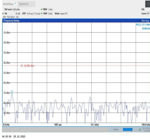
66-66-5MHz-15MHz-QPSK-QPSK-132002-132095-1RB#0-0 RB#0-0.009~0.15MHz-PASS
