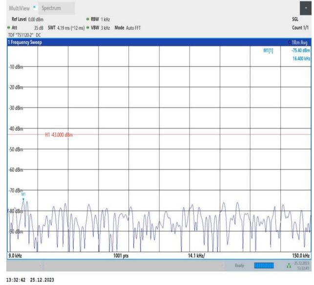
66-66-10MHz-10MHz-16QAM-16QAM-132523-132622-1RB#0-ORB#0-0.009~0.15MHz-PASS
