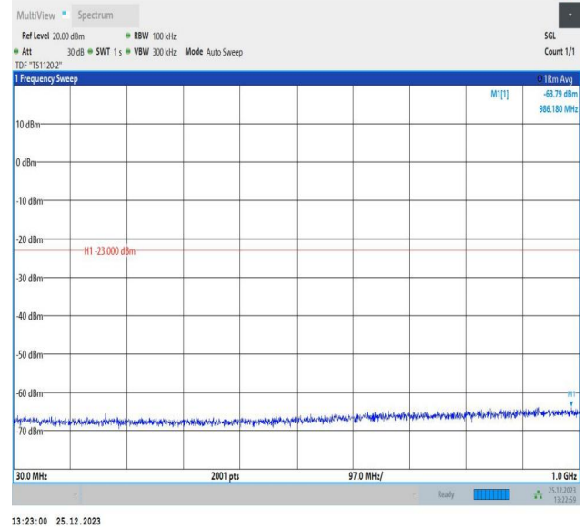
66-66-10MHz-10MHz-16QAM-16QAM-132022-132121-50RB #0-50RB#0-30~1000MHz-PASS
