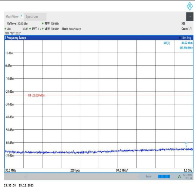
66-66-10MHz-10MHz-16QAM-16QAM-132523-132622-1RB#0-ORB#0-30~1000MHz-PASS
