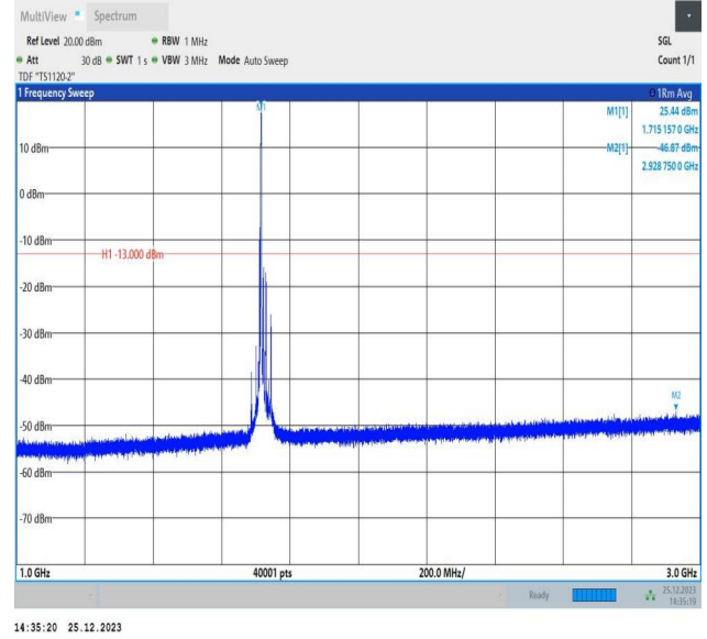
66-66-5MHz-15MHz-QPSK-QPSK-132002-132095-1RB#24-0 RB#0-1000~3000MHz-PASS
