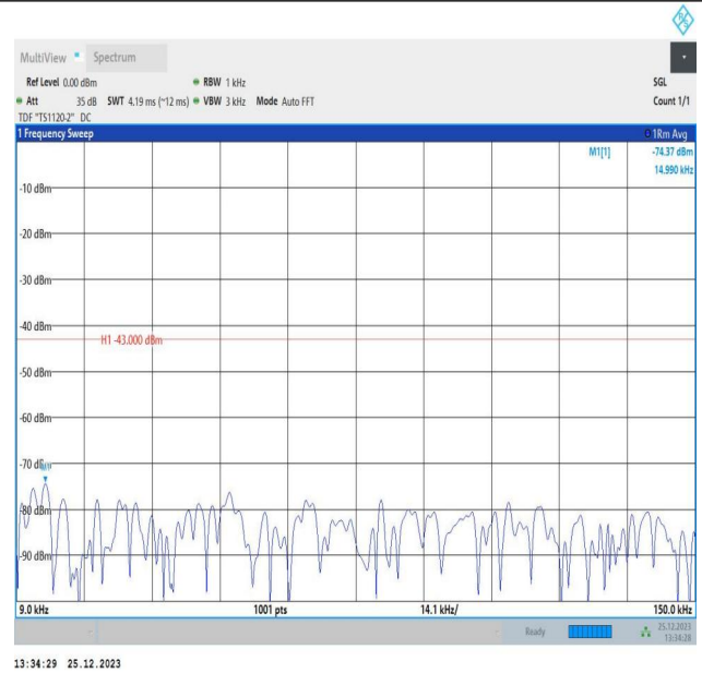
66-66-10MHz-10MHz-16QAM-16QAM-132523-132622-1RB# 49-ORB#0-0.009~0.15MHz-PASS
