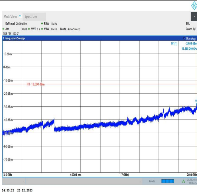
66-66-5MHz-15MHz-QPSK-QPSK-132002-132095-1RB#24- ORB#0-3000~20000MHz-PASS
