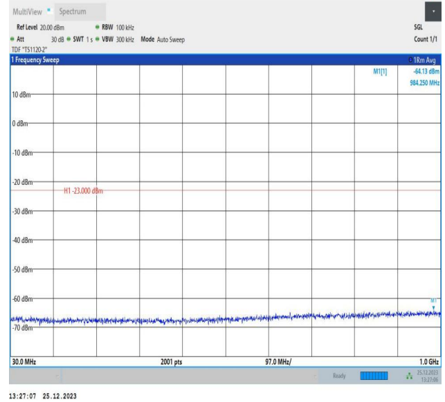
66-66-10MHz-10MHz-16QAM-16QAM-132373-132472-1RB# 49-ORB#0-30~1000MHz-PASS
