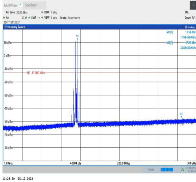
66-66-10MHz-10MHz-16QAM-16QAM-132373-132472-1RB# 0-1RB#49-1000~3000MHz-PASS
