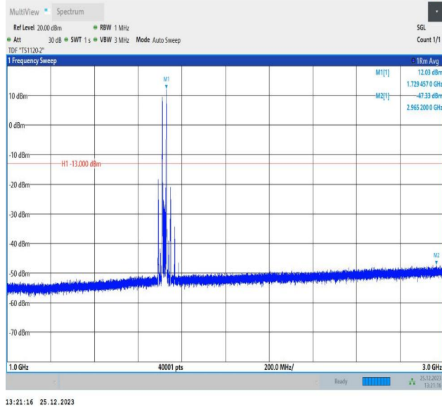
66-66-10MHz-10MHz-16QAM-16QAM-132022-132121-1RB# 0-1RB#49-1000~3000MHz-PASS
