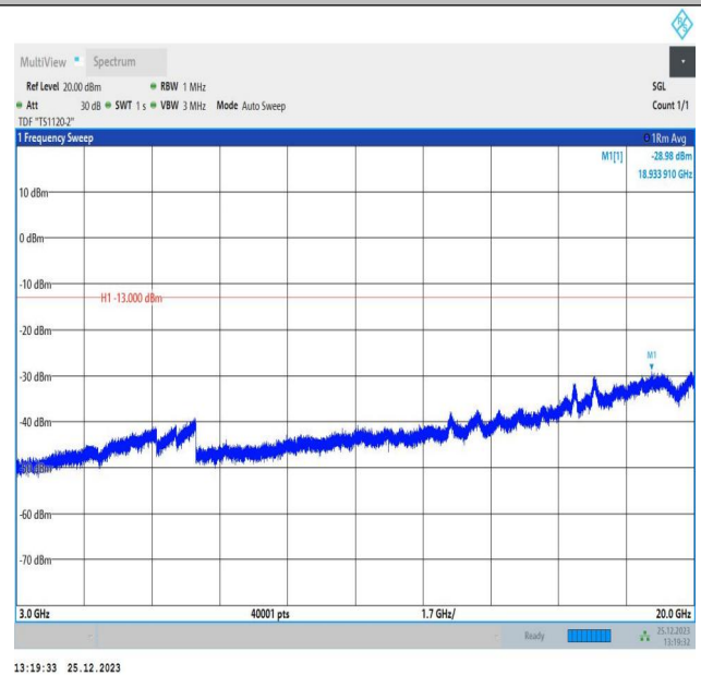
66-66-10MHz-10MHz-16QAM-16QAM-132022-132121-1RB# 49-ORB#0-3000~20000MHz-PASS
