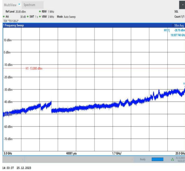
66-66-5MHz-15MHz-QPSK-QPSK-132002-132095-1RB#0-0 RB#0-3000~20000MHz-PASS
