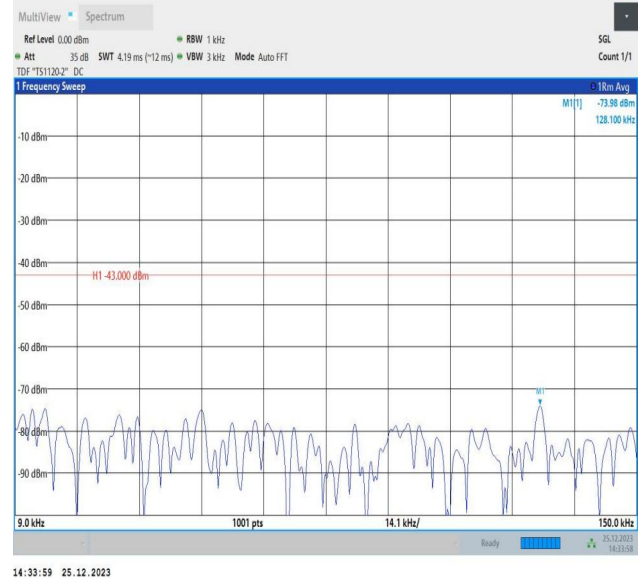
66-66-5MHz-15MHz-16QAM-16QAM-132002-132095-1RB#0-0 ORB#0-0.009~0.15MHz-PASS
