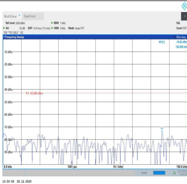
66-66-10MHz-10MHz-QPSK-QPSK-132523-132622-1RB#49 -ORB#0-0.009~0.15MHz-PASS
