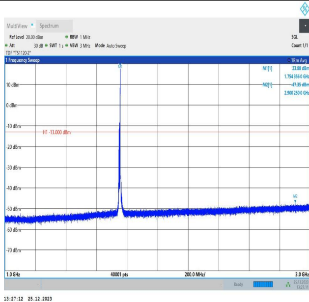
66-66-10MHz-10MHz-16QAM-16QAM-132373-132472-1RB# 49-ORB#0-1000~3000MHz-PASS
