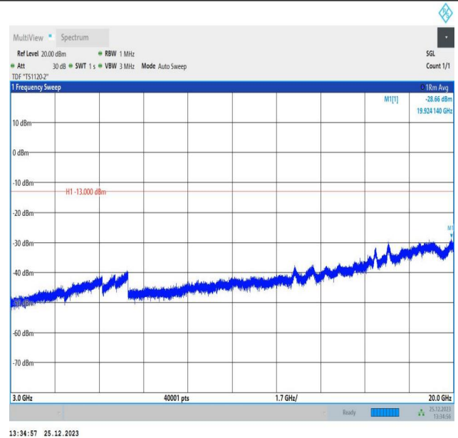
66-66-10MHz-10MHz-16QAM-16QAM-132523-132622-1RB# 49-ORB#0-3000~20000MHz-PASS
