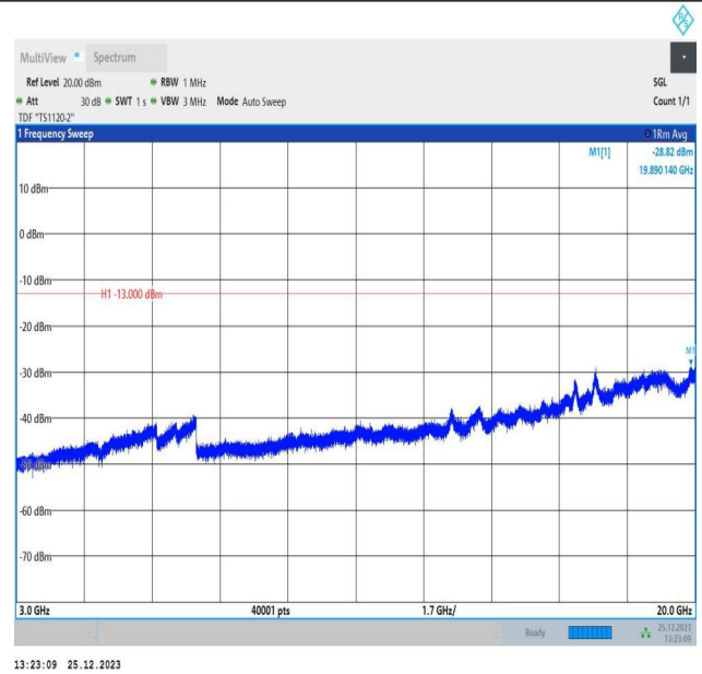
66-66-10MHz-10MHz-16QAM-16QAM-132022-132121-50RB #0-50RB#0-3000~20000MHz-PASS
