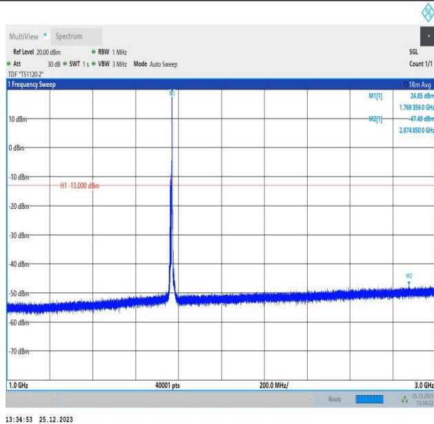
66-66-10MHz-10MHz-16QAM-16QAM-132523-132622-1RB# 49-ORB#0-1000~3000MHz-PASS
