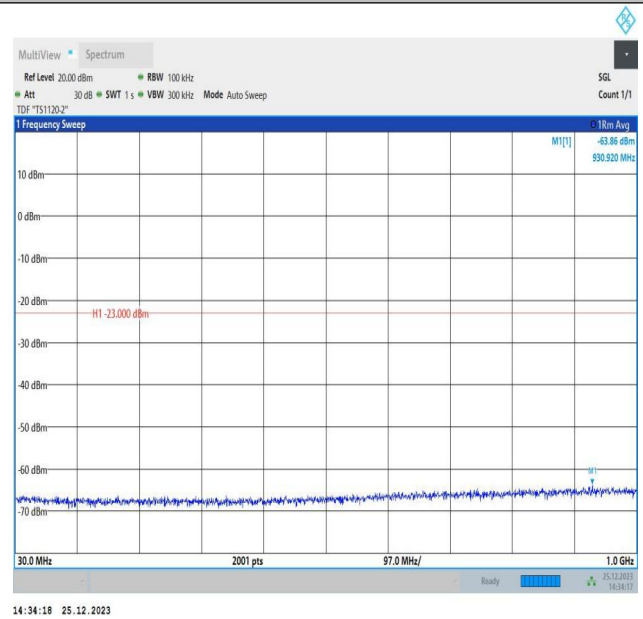
66-66-5MHz-15MHz-16QAM-16QAM-132002-132095-1RB#0-0 ORB#0-30~1000MHz-PASS
