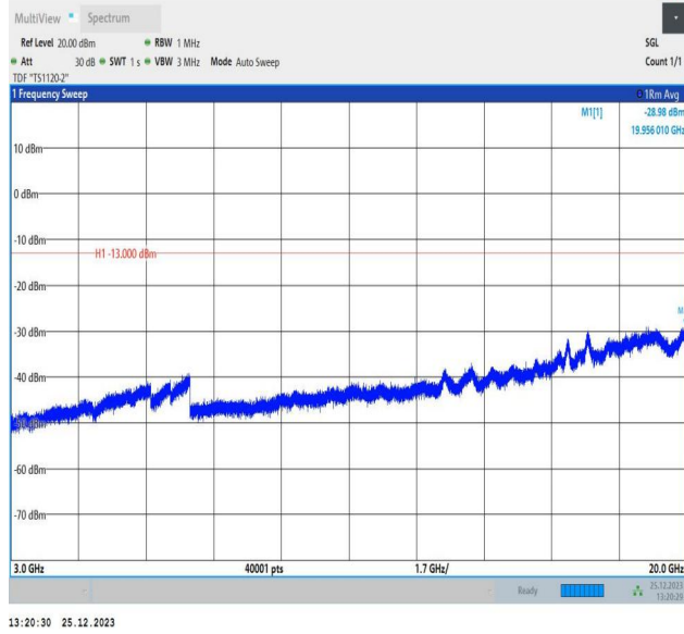
66-66-10MHz-10MHz-QPSK-QPSK-132022-132121-1RB#0-1RB#49-3000~20000MHz-PASS
