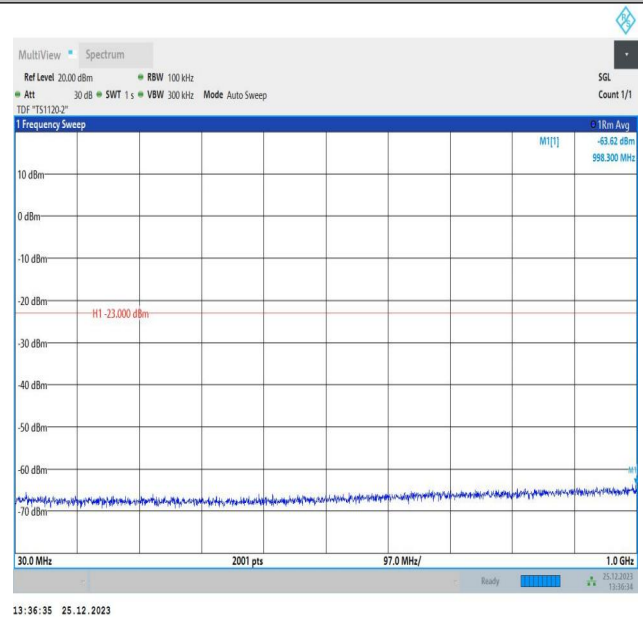
66-66-10MHz-10MHz-16QAM-16QAM-132523-132622-1RB#0-1RB#49-30~1000MHz-PASS
