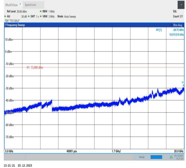
66-66-10MHz-10MHz-16QAM-16QAM-132022-132121-1RB# 0-1RB#49-3000~20000MHz-PASS
