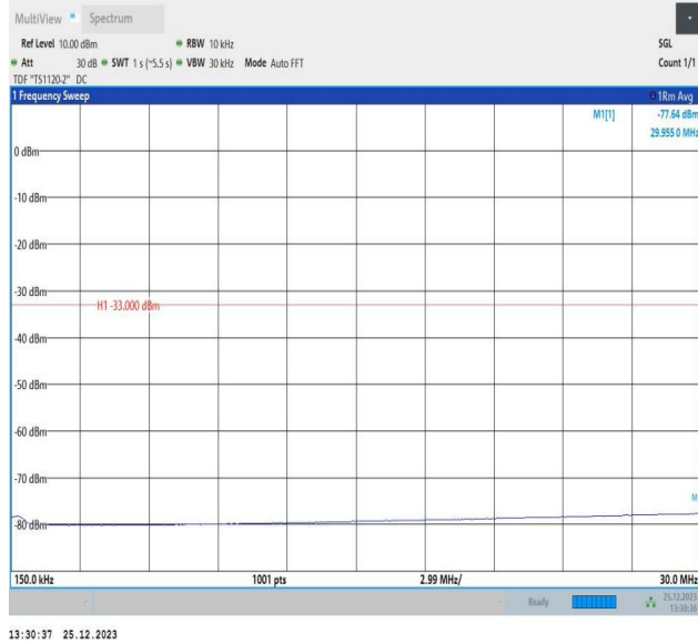
66-66-10MHz-10MHz-16QAM-16QAM-132373-132472-50RB #0-50RB#0-0.15~30MHz-PASS
