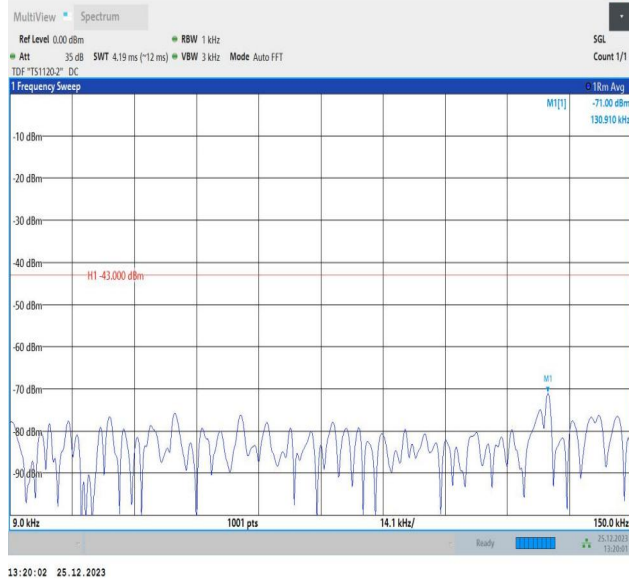
66-66-10MHz-10MHz-QPSK-QPSK-132022-132121-1RB#0-1RB#49-0.009~0.15MHz-PASS
