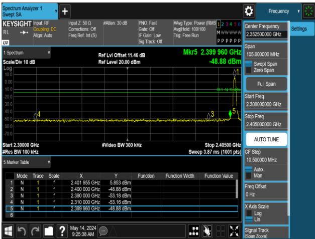
3DH5-Ant1-2402-PASS
