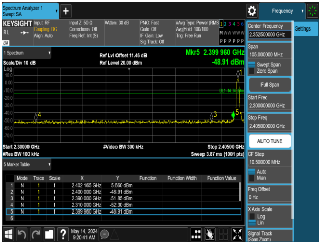
2DH5-Ant1-2402-PASS
