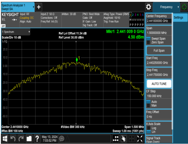
DH5-Ant1-2441-0~Reference-PASS
