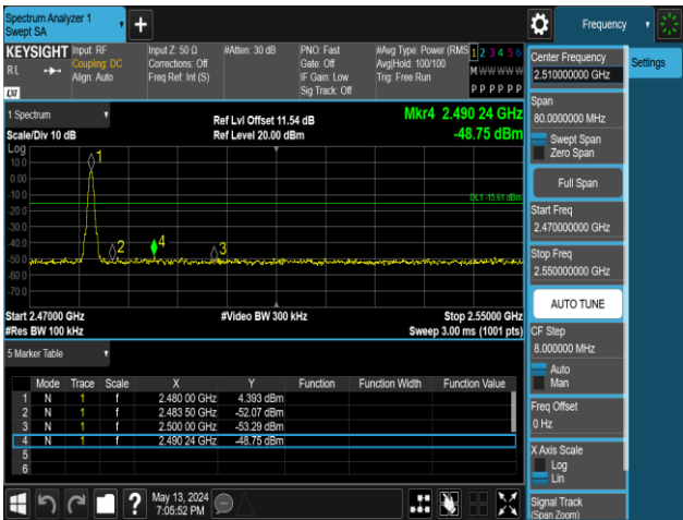
DH5-Ant1-2480-PASS
