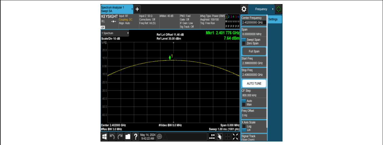
2DH5-Ant1-2402-PASS
