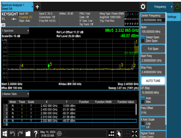
DH5-Ant1-Hop_2402-PASS
