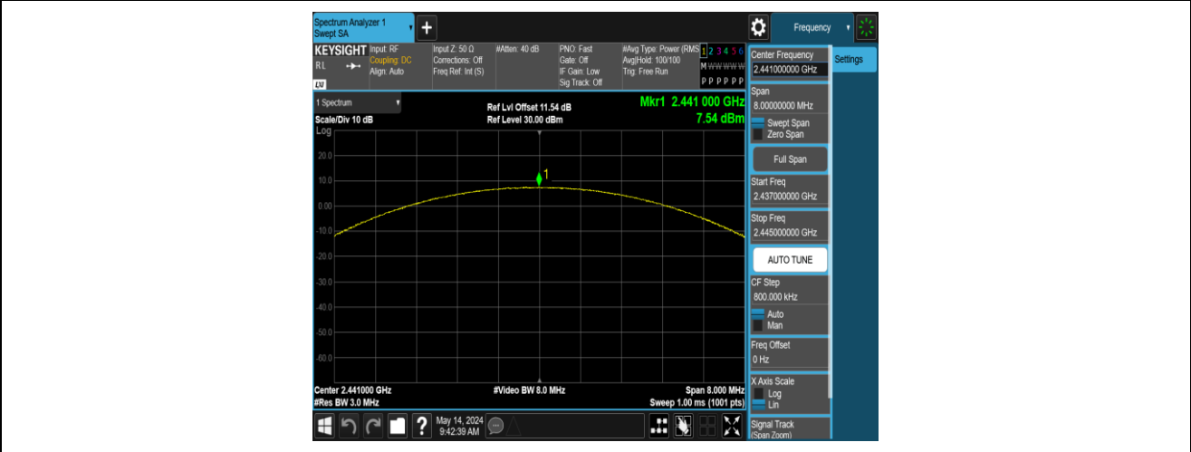
2DH5-Ant1-2441-PASS
