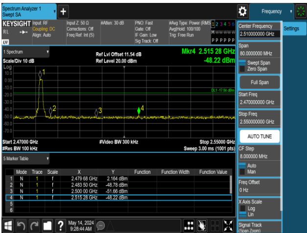
3DH5-Ant1-2480-PASS
