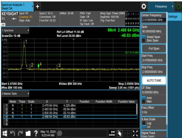
2DH5-Ant1-2480-PASS
