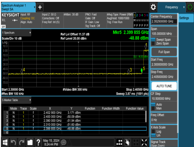
2DH5-Ant1-Hop_2402-PASS
