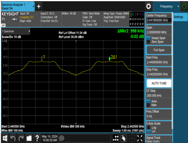
DH5-Ant1-Hop-PASS
