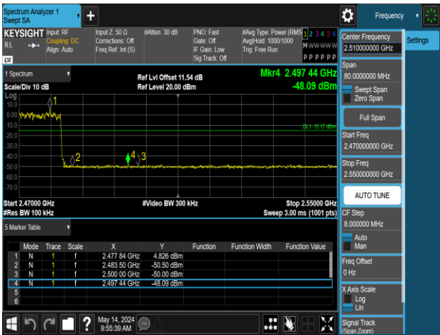
3DH5-Ant1-Hop_2480-PASS
