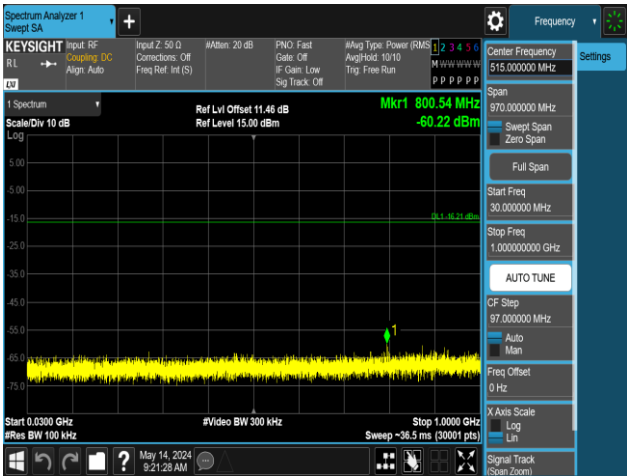
2DH5-Ant1-2402-30~1000-PASS
