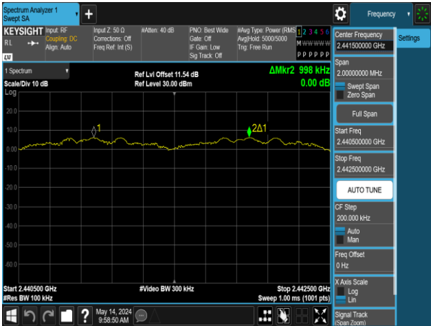
3DH5-Ant1-Hop-PASS
