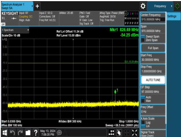
DH5-Ant1-2480-30~1000-PASS
