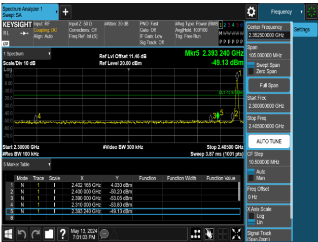
DH5-Ant1-2402-PASS
