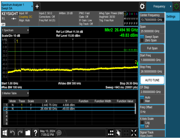
DH5-Ant1-2441-1000~26500-PASS
