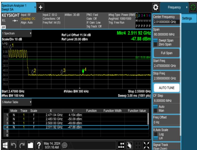
DH5-Ant1-Hop_2480-PASS
