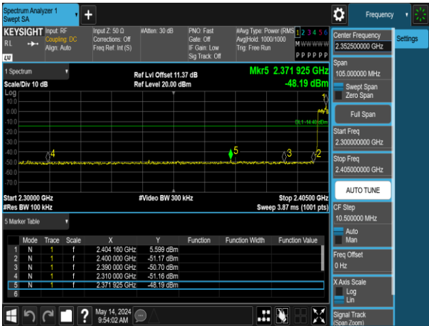
3DH5-Ant1-Hop_2402-PASS
