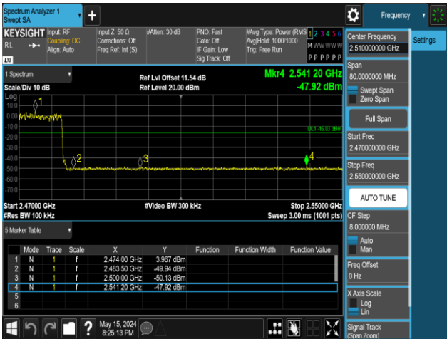
2DH5-Ant1-Hop_2480-PASS
