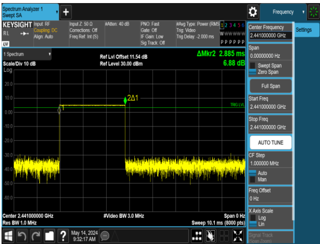
DH5-Ant1-Hop-PASS
