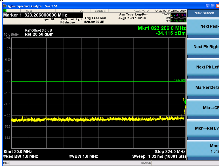
Channel 4183, 30MHz~824MHz
