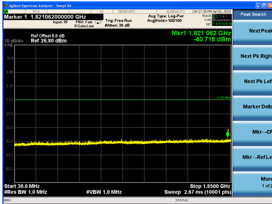
Channel 9400, 30MHz~1850MHz
