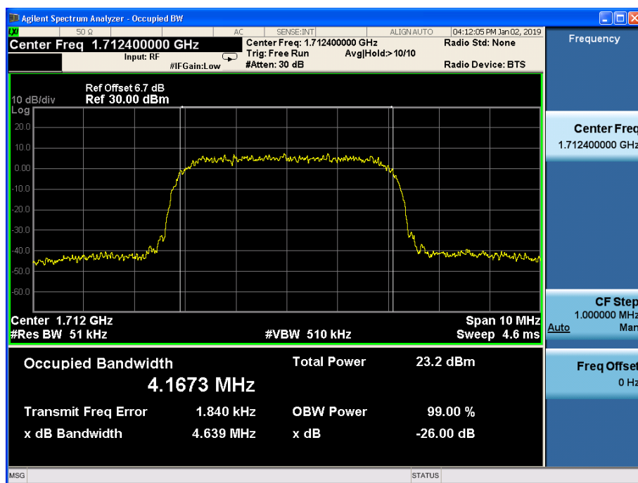
Channel 1312
