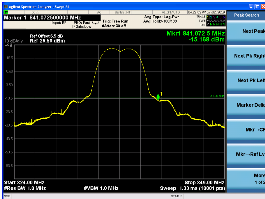
Channel 4183, 824MHz~849MHz
