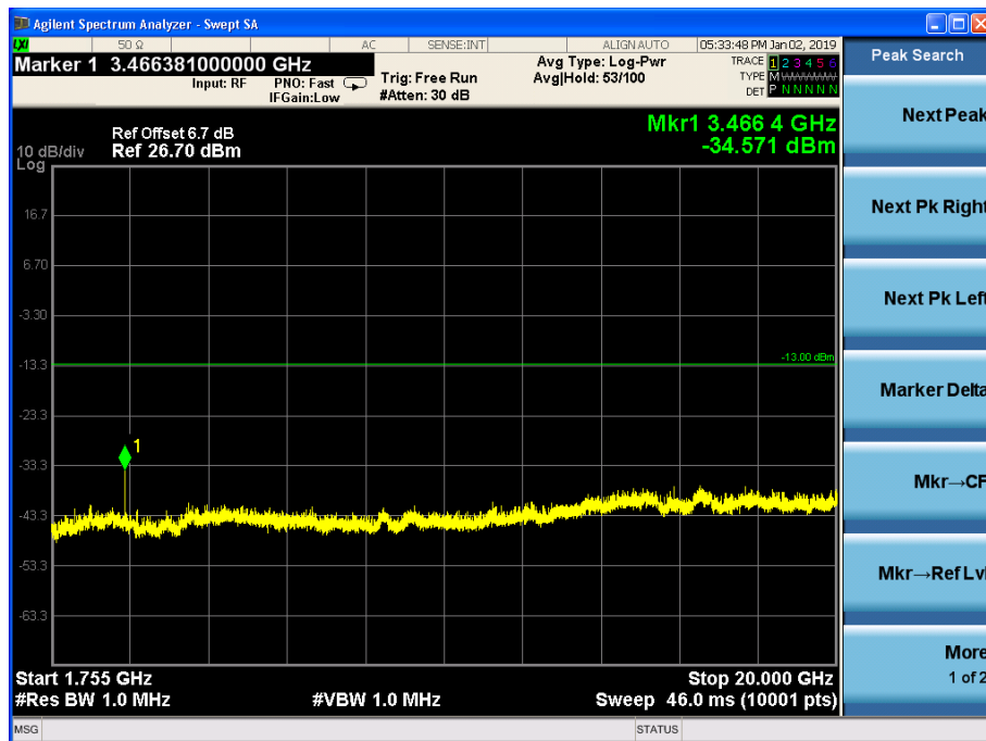
Channel 1412, 1755MHz~20GHz
