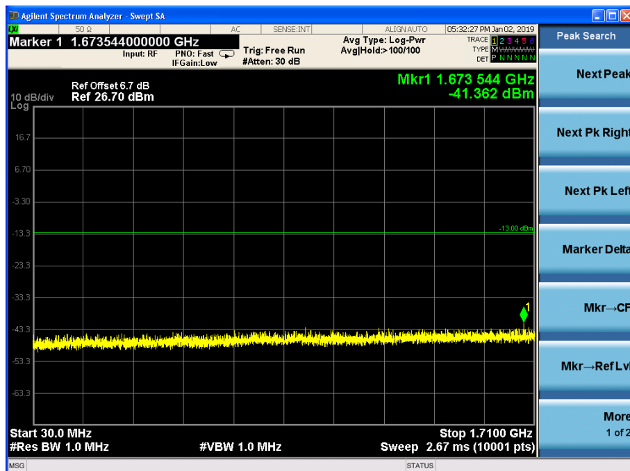
Channel 1412, 30MHz~1710MHz
