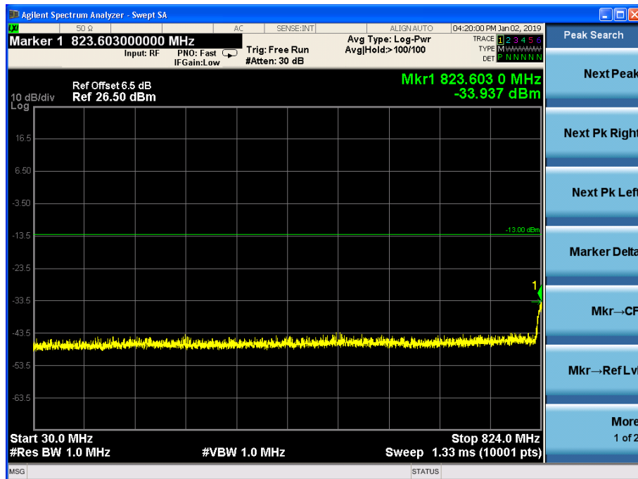
Channel 4183, 30MHz~824MHz
