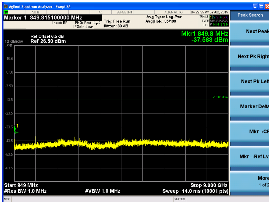
Channel 4183, 849MHz~9GHz
