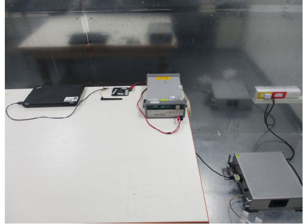
FCC_15_247_BLE_Conduction_Setup
