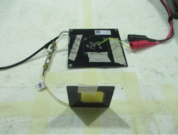
FCC_15_247_BLE_Radiated_ASC_RFANT3216120A5T_Setup
