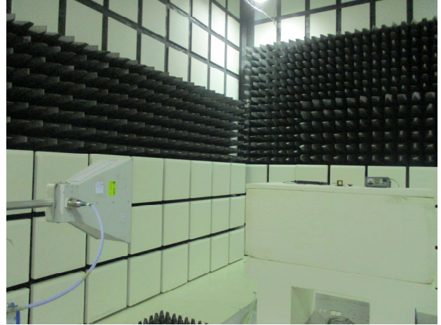
FCC_15_247_BLE_Radiated_ASC_RFANT3216120A5T_Setup
