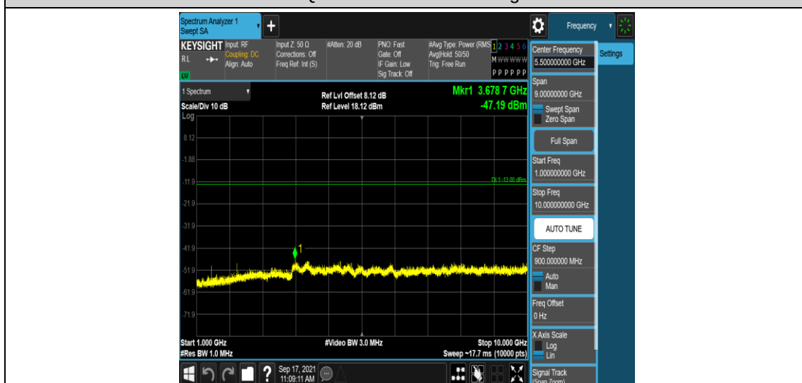
Band12-3MHz-16QAM-23025-1RB#0-Range4:1000~10000MHz
