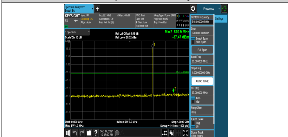
Band12-1.4MHz-16QAM-23017-1RB#0-Range3:30~1000MHz
