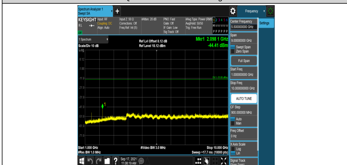
Band12-3MHz-QPSK-23025-1RB#0-Range4:1000~10000MHz
