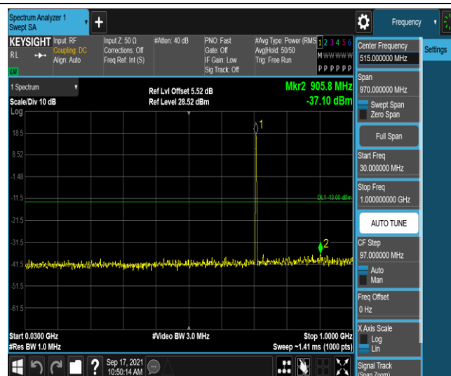
Band12-1.4MHz-QPSK-23173-1RB#0-Range3:30~1000MHz
