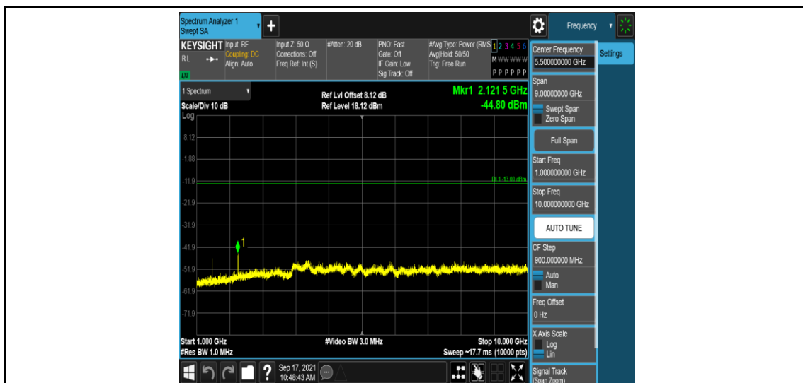
Band12-1.4MHz-QPSK-23095-1RB#0-Range4:1000~10000MHz
