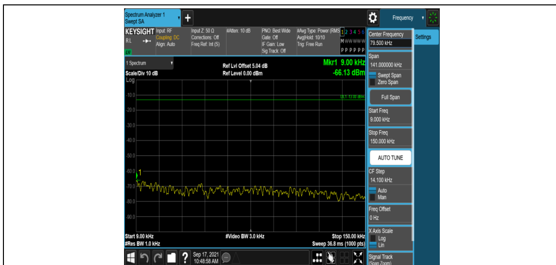
Band12-1.4MHz-16QAM-23095-1RB#0-Range1:0.009~0.15MHz
