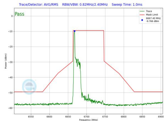
Plot 7-1257. LPI In-Band Emission Plot Antenna WF7 (80MHz 802.11ax RU26 (UNII Band 7) – Ch. 151)
