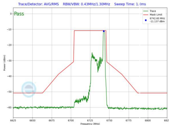
Plot 7-1255. LPI In-Band Emission Plot Antenna WF7 (40MHz 802.11ax RU26 (UNII Band 7) – Ch. 155)
