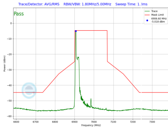
Plot 7-1213. LPI In-Band Emission Plot Antenna WF8 (160MHz 802.11ax RU26 (UNII Band 8) – Ch. 207)
