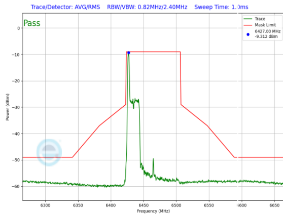
Plot 7-1330. LPI In-Band Emission Plot SDM Primary Antenna WF8 (80MHz 802.11ax RU26 (UNII Band 6) – Ch. 103)
