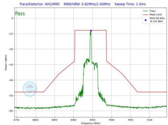
Plot 7-1274. LPI In-Band Emission Plot Antenna WF7 (80MHz 802.11ax RU26 (UNII Band 8) – Ch. 199)
