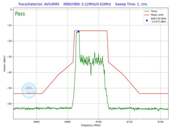
Plot 7-1249. LPI In-Band Emission Plot Antenna WF7 (20MHz 802.11ax RU26 (UNII Band 7) – Ch. 149)
