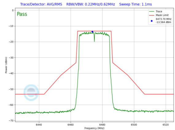
Plot 7-1320. LPI In-Band Emission Plot SDM Primary Antenna WF8 (20MHz 802.11ax RU242 (UNII Band 6) – Ch. 105)
