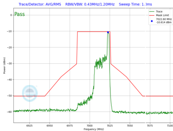
Plot 7-1271. LPI In-Band Emission Plot Antenna WF7 (40MHz 802.11ax RU26 (UNII Band 8) – Ch. 211)
