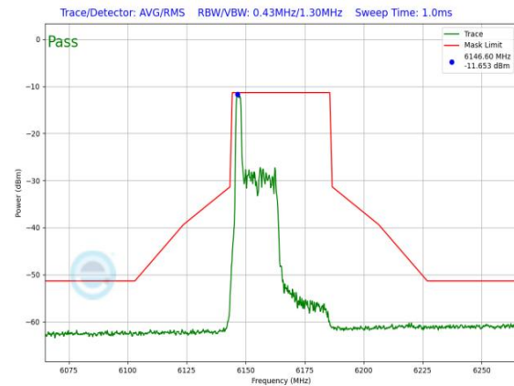
Plot 7-1290. LPI In-Band Emission Plot SDM Primary Antenna WF8 (40MHz 802.11ax RU26 (UNII Band 5) – Ch. 43)
