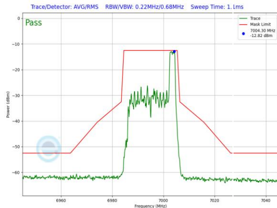
Plot 7-1267. LPI In-Band Emission Plot Antenna WF7 (20MHz 802.11ax RU26 (UNII Band 8) – Ch. 209)
