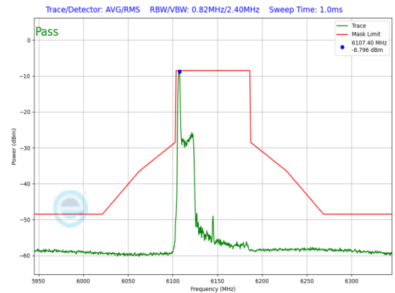
Plot 7-1298. LPI In-Band Emission Plot SDM Primary Antenna WF8 (80MHz 802.11ax RU26 (UNII Band 5) – Ch. 39)
