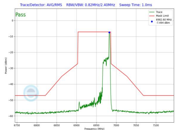
Plot 7-1275. LPI In-Band Emission Plot Antenna WF7 (80MHz 802.11ax RU26 (UNII Band 8) – Ch. 199)
