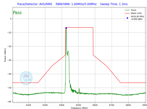
Plot 7-1245. LPI In-Band Emission Plot Antenna WF7 (160MHz 802.11ax RU26 (UNII Band 6) – Ch. 111)
