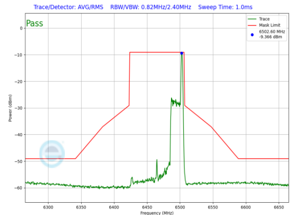
Plot 7-1334. LPI In-Band Emission Plot SDM Primary Antenna WF8 (80MHz 802.11ax RU26 (UNII Band 6) – Ch. 103)
