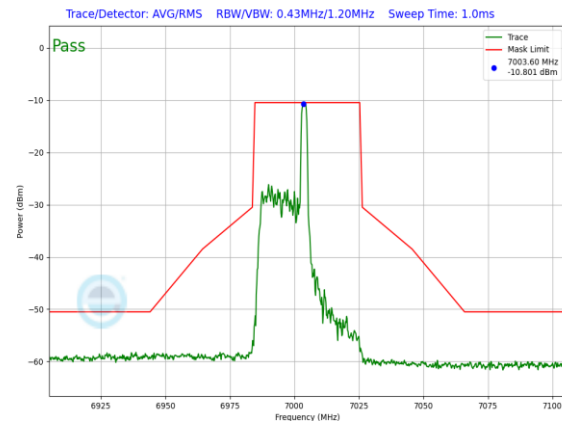
Plot 7-1270. LPI In-Band Emission Plot Antenna WF7 (40MHz 802.11ax RU26 (UNII Band 8) – Ch. 211)
