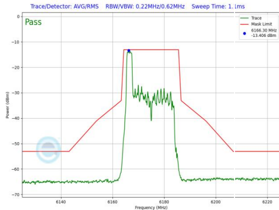
Plot 7-1282. LPI In-Band Emission Plot SDM Primary Antenna WF8 (20MHz 802.11ax RU26 (UNII Band 5) – Ch. 45)
