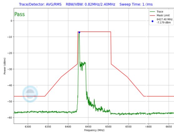
Plot 7-1241. LPI In-Band Emission Plot Antenna WF7 (80MHz 802.11ax RU26 (UNII Band 6) – Ch. 103)
