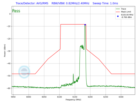
Plot 7-1302. LPI In-Band Emission Plot SDM Primary Antenna WF8 (80MHz 802.11ax RU26 (UNII Band 5) – Ch. 39)
