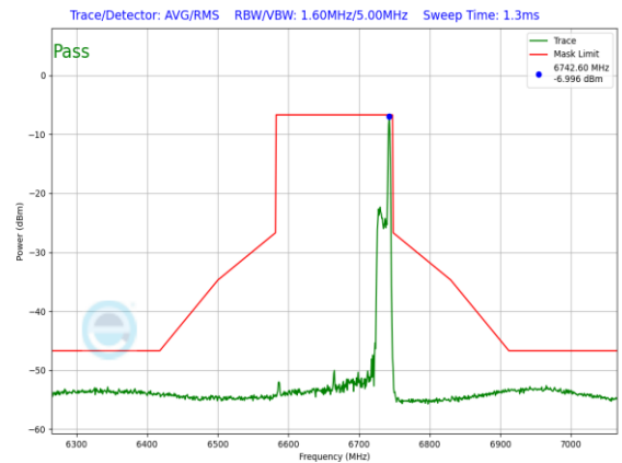
Plot 7-1263. LPI In-Band Emission Plot Antenna WF7 (160MHz 802.11ax RU26 (UNII Band 7) – Ch. 143)
