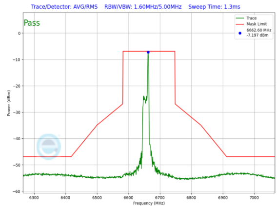
Plot 7-1262. LPI In-Band Emission Plot Antenna WF7 (160MHz 802.11ax RU26 (UNII Band 7) – Ch. 143)
