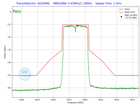
Plot 7-1328. LPI In-Band Emission Plot SDM Primary Antenna WF8 (40MHz 802.11ax RU484 (UNII Band 6) – Ch. 107)
