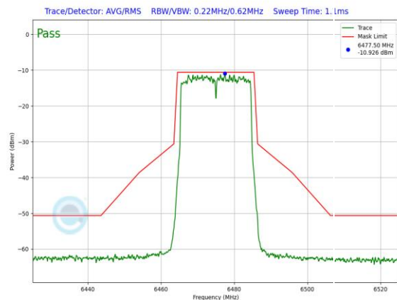
Plot 7-1236. LPI In-Band Emission Plot Antenna WF7 (20MHz 802.11ax RU242 (UNII Band 6) – Ch. 105)
