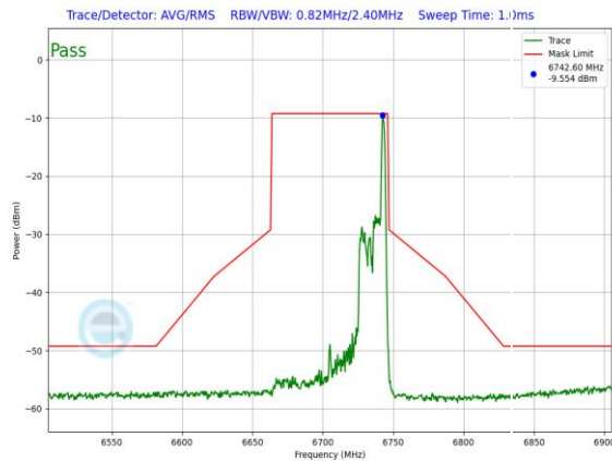
Plot 7-1259. LPI In-Band Emission Plot Antenna WF7 (80MHz 802.11ax RU26 (UNII Band 7) – Ch. 151)
