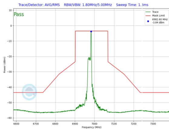
Plot 7-1214. LPI In-Band Emission Plot Antenna WF8 (160MHz 802.11ax RU26 (UNII Band 8) – Ch. 207)
