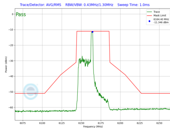
Plot 7-1292. LPI In-Band Emission Plot SDM Primary Antenna WF8 (40MHz 802.11ax RU26 (UNII Band 5) – Ch. 43)
