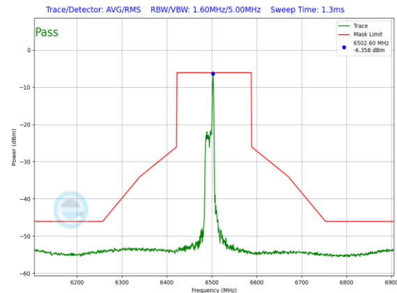
Plot 7-1246. LPI In-Band Emission Plot Antenna WF7 (160MHz 802.11ax RU26 (UNII Band 6) – Ch. 111)
