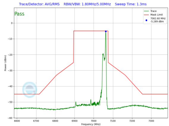
Plot 7-1279. LPI In-Band Emission Plot Antenna WF7 (160MHz 802.11ax RU26 (UNII Band 8) – Ch. 207)
