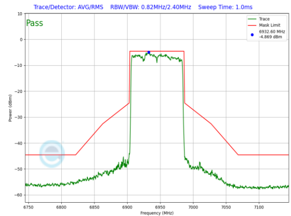
Plot 7-1276. LPI In-Band Emission Plot Antenna WF7 (80MHz 802.11ax RU996 (UNII Band 8) – Ch. 199)
