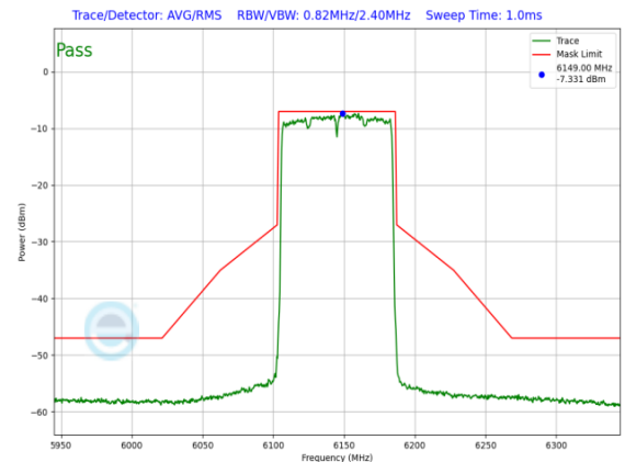
Plot 7-1304. LPI In-Band Emission Plot SDM Primary Antenna WF8 (80MHz 802.11ax RU996 (UNII Band 5) – Ch. 39)
