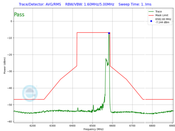
Plot 7-1247. LPI In-Band Emission Plot Antenna WF7 (160MHz 802.11ax RU26 (UNII Band 6) – Ch. 111)
