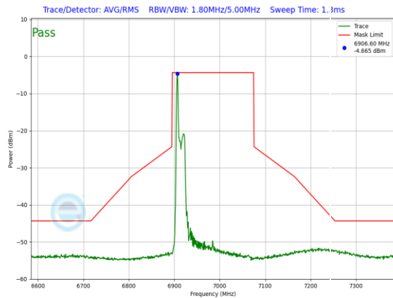
Plot 7-1277. LPI In-Band Emission Plot Antenna WF7 (160MHz 802.11ax RU26 (UNII Band 8) – Ch. 207)
