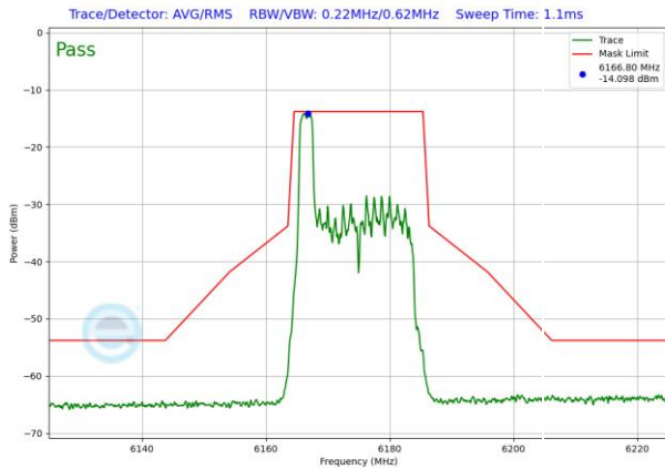
Plot 7-1281. LPI In-Band Emission Plot SDM Primary Antenna WF5B (20MHz 802.11ax RU26 (UNII Band 5) – Ch. 45)
