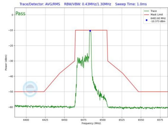
Plot 7-1238. LPI In-Band Emission Plot Antenna WF7 (40MHz 802.11ax RU26 (UNII Band 6) – Ch. 107)
