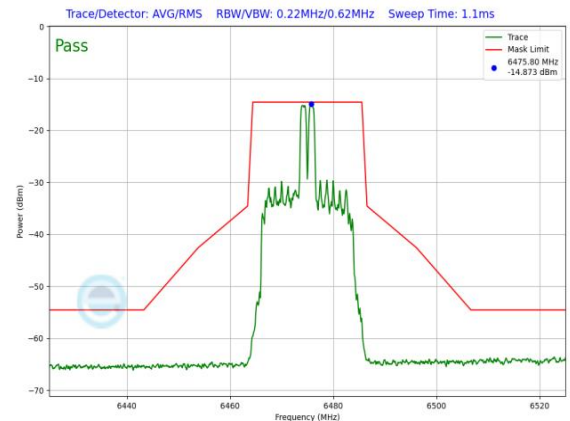
Plot 7-1316. LPI In-Band Emission Plot SDM Primary Antenna WF8 (20MHz 802.11ax RU26 (UNII Band 6) – Ch. 105)
