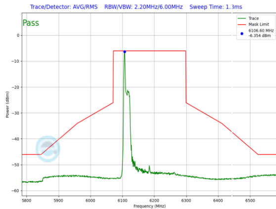
Plot 7-1305. LPI In-Band Emission Plot SDM Primary Antenna WF5B (160MHz 802.11ax RU26 (UNII Band 5) – Ch. 47)
