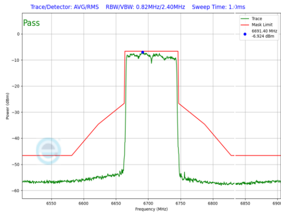
Plot 7-1260. LPI In-Band Emission Plot Antenna WF7 (80MHz 802.11ax RU996 (UNII Band 7) – Ch. 151)
