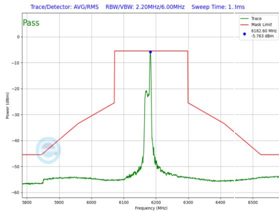
Plot 7-1307. LPI In-Band Emission Plot SDM Primary Antenna WF5B (160MHz 802.11ax RU26 (UNII Band 5) – Ch. 47)
