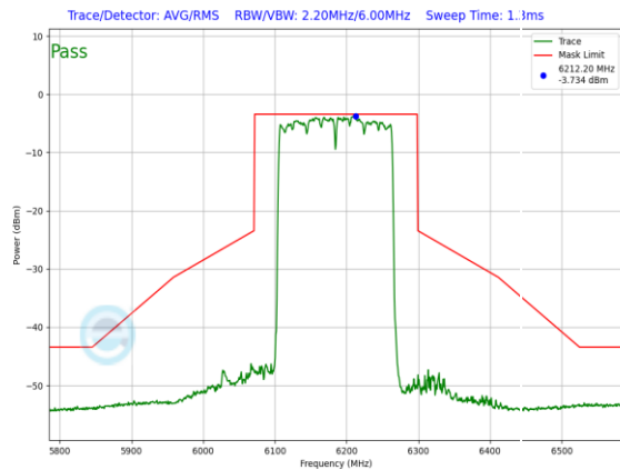
Plot 7-1311. LPI In-Band Emission Plot SDM Primary Antenna WF5B (160MHz 802.11ax RU996x2 (UNII Band 5) – Ch. 47)
