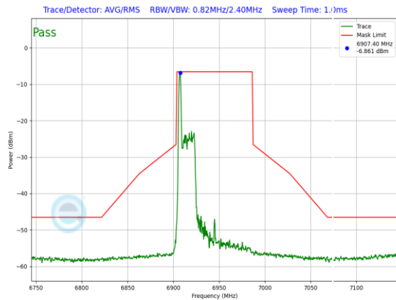
Plot 7-1273. LPI In-Band Emission Plot Antenna WF7 (80MHz 802.11ax RU26 (UNII Band 8) – Ch. 199)
