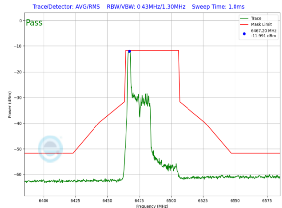
Plot 7-1322. LPI In-Band Emission Plot SDM Primary Antenna WF8 (40MHz 802.11ax RU26 (UNII Band 6) – Ch. 107)
