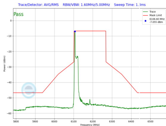
Plot 7-1306. LPI In-Band Emission Plot SDM Primary Antenna WF8 (160MHz 802.11ax RU26 (UNII Band 5) – Ch. 47)
