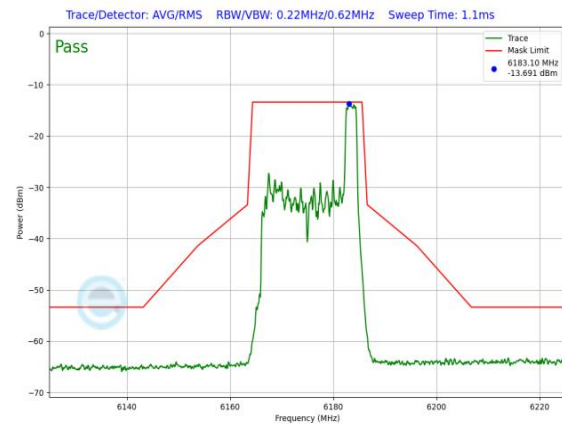
Plot 7-1286. LPI In-Band Emission Plot SDM Primary Antenna WF8 (20MHz 802.11ax RU26 (UNII Band 5) – Ch. 45)
