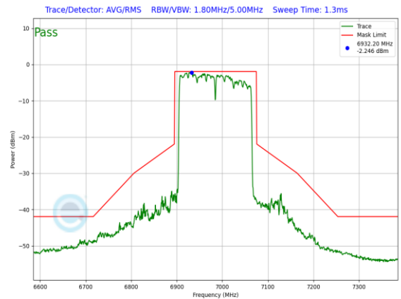
Plot 7-1280. LPI In-Band Emission Plot Antenna WF7 (160MHz 802.11ax RU996x2 (UNII Band 8) – Ch. 207)
