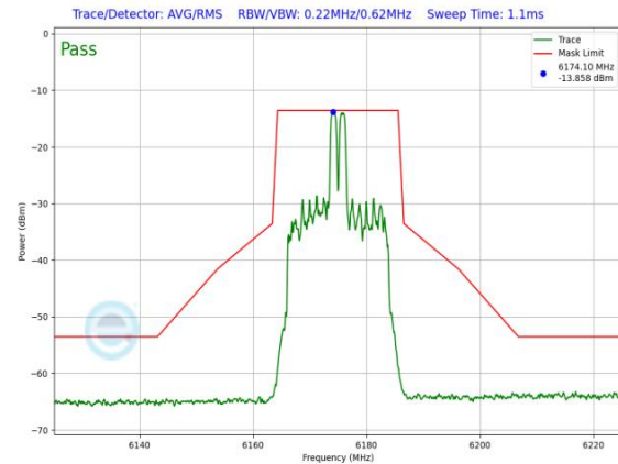
Plot 7-1284. LPI In-Band Emission Plot SDM Primary Antenna WF8 (20MHz 802.11ax RU26 (UNII Band 5) – Ch. 45)
