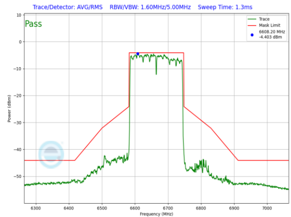
Plot 7-1264. LPI In-Band Emission Plot Antenna WF7 (160MHz 802.11ax RU996x2 (UNII Band 7) – Ch. 143)
