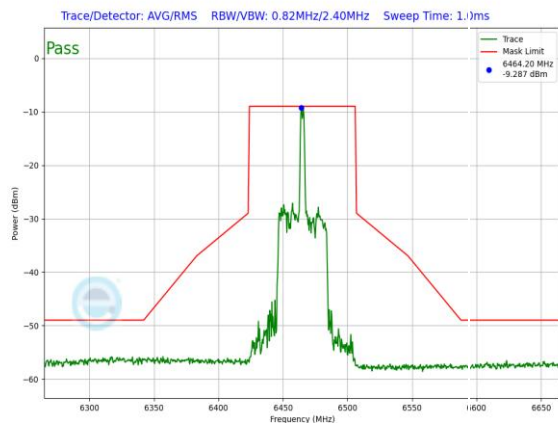
Plot 7-1242. LPI In-Band Emission Plot Antenna WF7 (80MHz 802.11ax RU26 (UNII Band 6) – Ch. 103)
