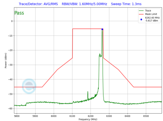
Plot 7-1310. LPI In-Band Emission Plot SDM Primary Antenna WF8 (160MHz 802.11ax RU26 (UNII Band 5) – Ch. 47)
