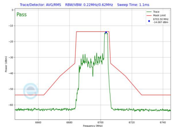
Plot 7-1251. LPI In-Band Emission Plot Antenna WF7 (20MHz 802.11ax RU26 (UNII Band 7) – Ch. 149)
