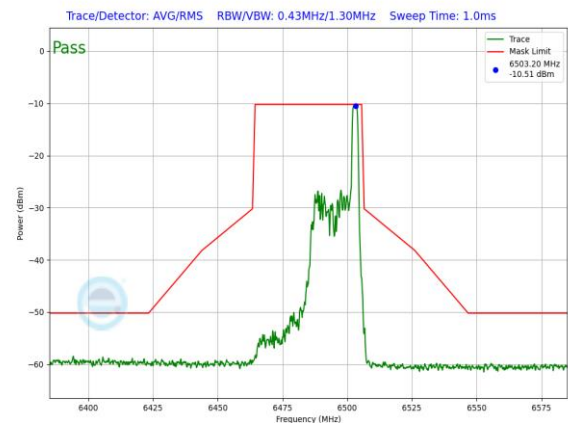
Plot 7-1239. LPI In-Band Emission Plot Antenna WF7 (40MHz 802.11ax RU26 (UNII Band 6) – Ch. 107)
