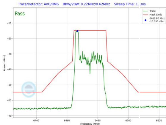
Plot 7-1313. LPI In-Band Emission Plot SDM Primary Antenna WF5B (20MHz 802.11ax RU26 (UNII Band 6) – Ch. 105)
