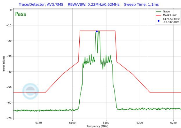
Plot 7-1283. LPI In-Band Emission Plot SDM Primary Antenna WF5B (20MHz 802.11ax RU26 (UNII Band 5) – Ch. 45)
