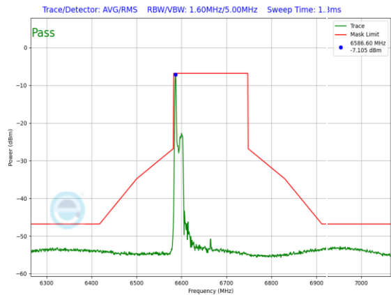
Plot 7-1261. LPI In-Band Emission Plot Antenna WF7 (160MHz 802.11ax RU26 (UNII Band 7) – Ch. 143)
