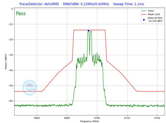
Plot 7-1250. LPI In-Band Emission Plot Antenna WF7 (20MHz 802.11ax RU26 (UNII Band 7) – Ch. 149)
