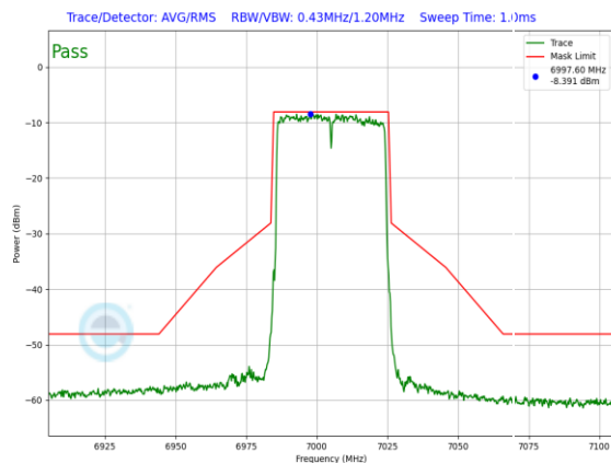
Plot 7-1272. LPI In-Band Emission Plot Antenna WF7 (40MHz 802.11ax RU484 (UNII Band 8) – Ch. 211)
