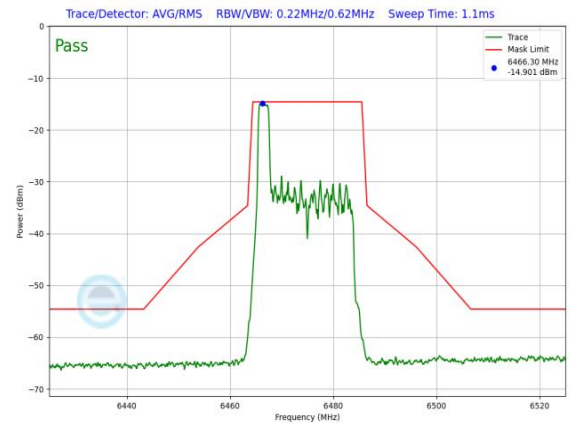
Plot 7-1314. LPI In-Band Emission Plot SDM Primary Antenna WF8 (20MHz 802.11ax RU26 (UNII Band 6) – Ch. 105)
