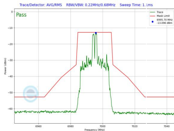
Plot 7-1266. LPI In-Band Emission Plot Antenna WF7 (20MHz 802.11ax RU26 (UNII Band 8) – Ch. 209)
