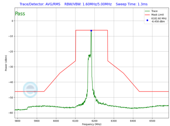
Plot 7-1308. LPI In-Band Emission Plot SDM Primary Antenna WF8 (160MHz 802.11ax RU26 (UNII Band 5) – Ch. 47)
