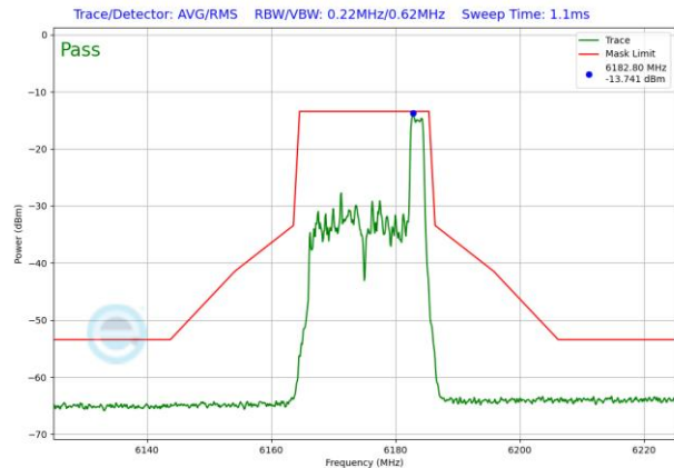
Plot 7-1285. LPI In-Band Emission Plot SDM Primary Antenna WF5B (20MHz 802.11ax RU26 (UNII Band 5) – Ch. 45)
