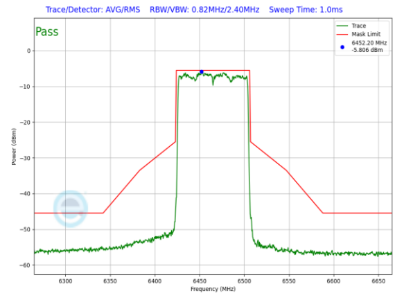
Plot 7-1244. LPI In-Band Emission Plot Antenna WF7 (80MHz 802.11ax RU996 (UNII Band 6) – Ch. 103)
