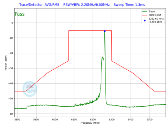
Plot 7-1309. LPI In-Band Emission Plot SDM Primary Antenna WF5B (160MHz 802.11ax RU26 (UNII Band 5) – Ch. 47)
