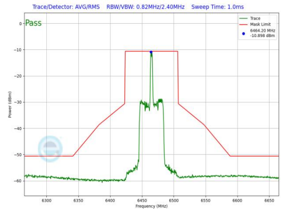
Plot 7-1332. LPI In-Band Emission Plot SDM Primary Antenna WF8 (80MHz 802.11ax RU26 (UNII Band 6) – Ch. 103)
