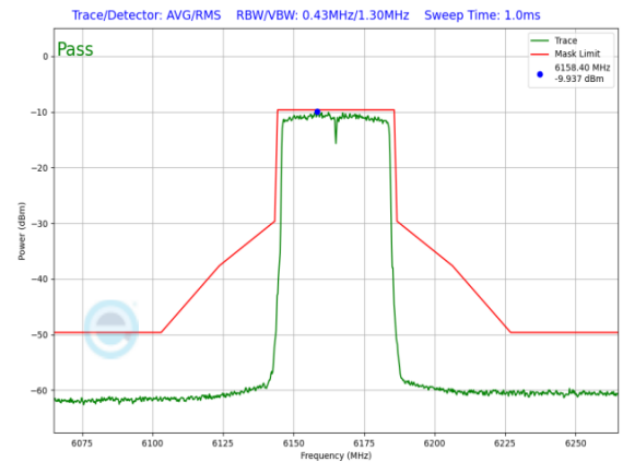
Plot 7-1296. LPI In-Band Emission Plot SDM Primary Antenna WF8 (40MHz 802.11ax RU484 (UNII Band 5) – Ch. 43)
