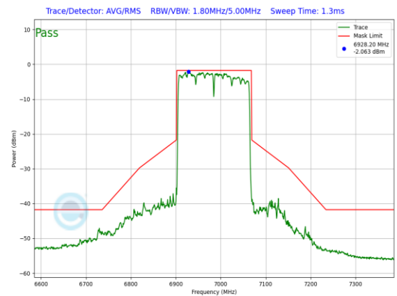
Plot 7-1216. LPI In-Band Emission Plot Antenna WF8 (160MHz 802.11ax RU996x2 (UNII Band 8) – Ch. 207)
