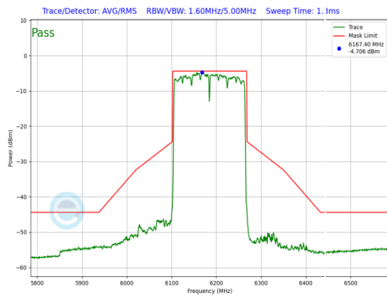
Plot 7-1312. LPI In-Band Emission Plot SDM Primary Antenna WF8 (160MHz 802.11ax RU996x2 (UNII Band 5) – Ch. 47)
