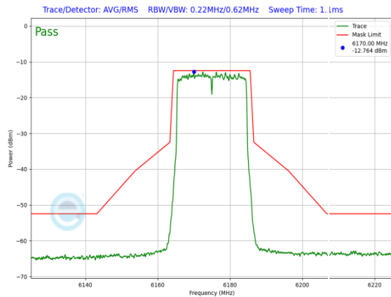
Plot 7-1288. LPI In-Band Emission Plot SDM Primary Antenna WF8 (20MHz 802.11ax RU242 (UNII Band 5) – Ch. 45)
