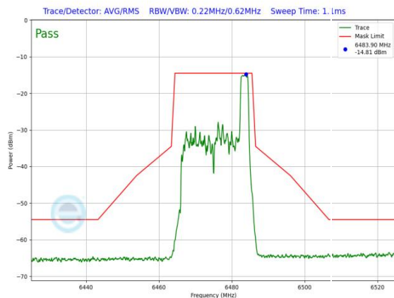
Plot 7-1318. LPI In-Band Emission Plot SDM Primary Antenna WF8 (20MHz 802.11ax RU26 (UNII Band 6) – Ch. 105)
