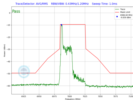
Plot 7-1269. LPI In-Band Emission Plot Antenna WF7 (40MHz 802.11ax RU26 (UNII Band 8) – Ch. 211)
