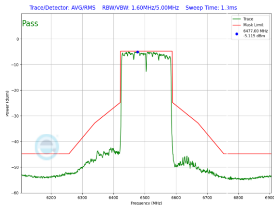
Plot 7-1248. LPI In-Band Emission Plot Antenna WF7 (160MHz 802.11ax RU996x2 (UNII Band 6) – Ch. 111)
