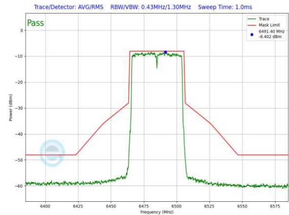
Plot 7-1240. LPI In-Band Emission Plot Antenna WF7 (40MHz 802.11ax RU484 (UNII Band 6) – Ch. 107)
