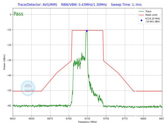
Plot 7-1254. LPI In-Band Emission Plot Antenna WF7 (40MHz 802.11ax RU26 (UNII Band 7) – Ch. 155)
