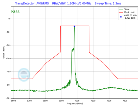
Plot 7-1278. LPI In-Band Emission Plot Antenna WF7 (160MHz 802.11ax RU26 (UNII Band 8) – Ch. 207)
