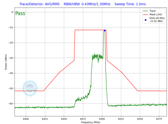
Plot 7-1326. LPI In-Band Emission Plot SDM Primary Antenna WF8 (40MHz 802.11ax RU26 (UNII Band 6) – Ch. 107)
