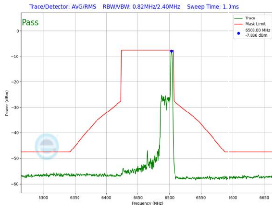
Plot 7-1243. LPI In-Band Emission Plot Antenna WF7 (80MHz 802.11ax RU26 (UNII Band 6) – Ch. 103)
