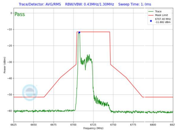
Plot 7-1253. LPI In-Band Emission Plot Antenna WF7 (40MHz 802.11ax RU26 (UNII Band 7) – Ch. 155)
