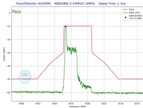
Plot 7-1237. LPI In-Band Emission Plot Antenna WF7 (40MHz 802.11ax RU26 (UNII Band 6) – Ch. 107)
