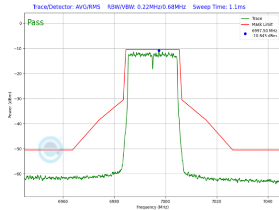
Plot 7-1268. LPI In-Band Emission Plot Antenna WF7 (20MHz 802.11ax RU242 (UNII Band 8) – Ch. 209)
