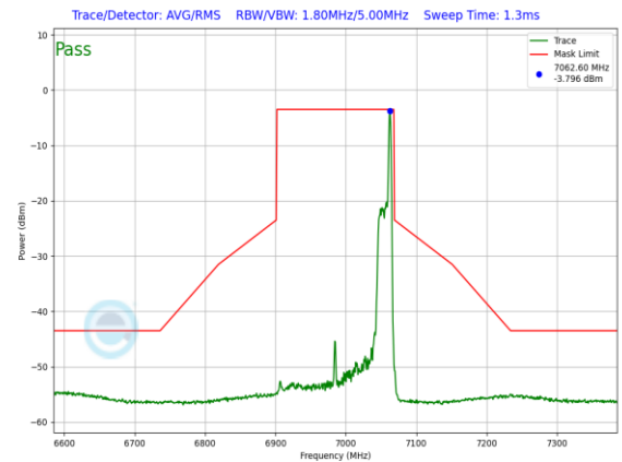
Plot 7-1215. LPI In-Band Emission Plot Antenna WF8 (160MHz 802.11ax RU26 (UNII Band 8) – Ch. 207)
