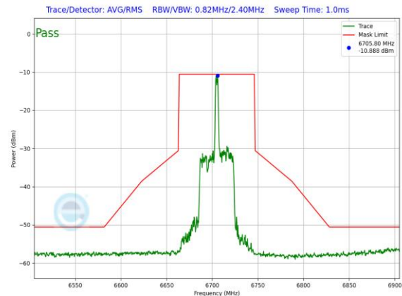
Plot 7-1258. LPI In-Band Emission Plot Antenna WF7 (80MHz 802.11ax RU26 (UNII Band 7) – Ch. 151)
