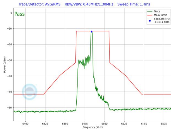
Plot 7-1324. LPI In-Band Emission Plot SDM Primary Antenna WF8 (40MHz 802.11ax RU26 (UNII Band 6) – Ch. 107)
