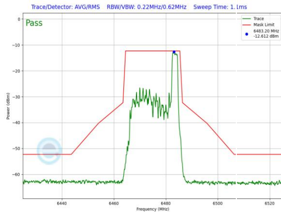
Plot 7-1235. LPI In-Band Emission Plot Antenna WF7 (20MHz 802.11ax RU26 (UNII Band 6) – Ch. 105)
