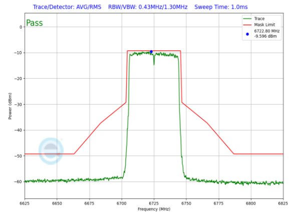
Plot 7-1256. LPI In-Band Emission Plot Antenna WF7 (40MHz 802.11ax RU484 (UNII Band 7) – Ch. 155)
