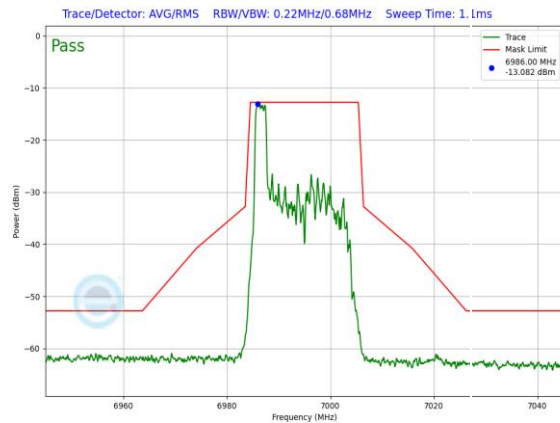
Plot 7-1265. LPI In-Band Emission Plot Antenna WF7 (20MHz 802.11ax RU26 (UNII Band 8) – Ch. 209)
