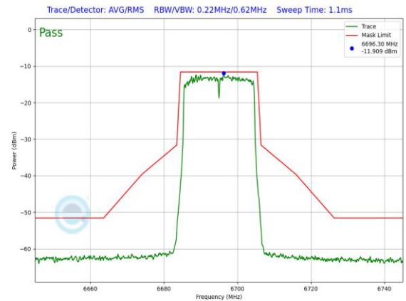
Plot 7-1252. LPI In-Band Emission Plot Antenna WF7 (20MHz 802.11ax RU242 (UNII Band 7) – Ch. 149)
