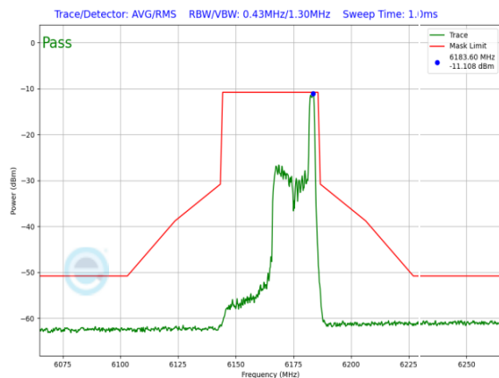
Plot 7-1294. LPI In-Band Emission Plot SDM Primary Antenna WF8 (40MHz 802.11ax RU26 (UNII Band 5) – Ch. 43)
