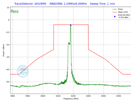
Plot 7-1230. LPI In-Band Emission Plot Antenna WF7 (160MHz 802.11ax RU26 (UNII Band 5) – Ch. 47)
