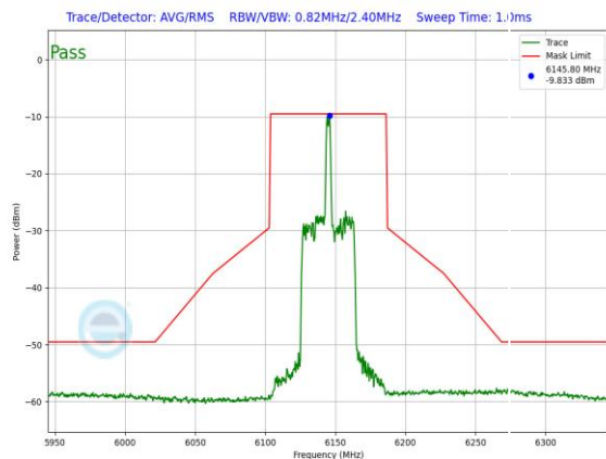
Plot 7-1300. LPI In-Band Emission Plot SDM Primary Antenna WF8 (80MHz 802.11ax RU26 (UNII Band 5) – Ch. 39)
