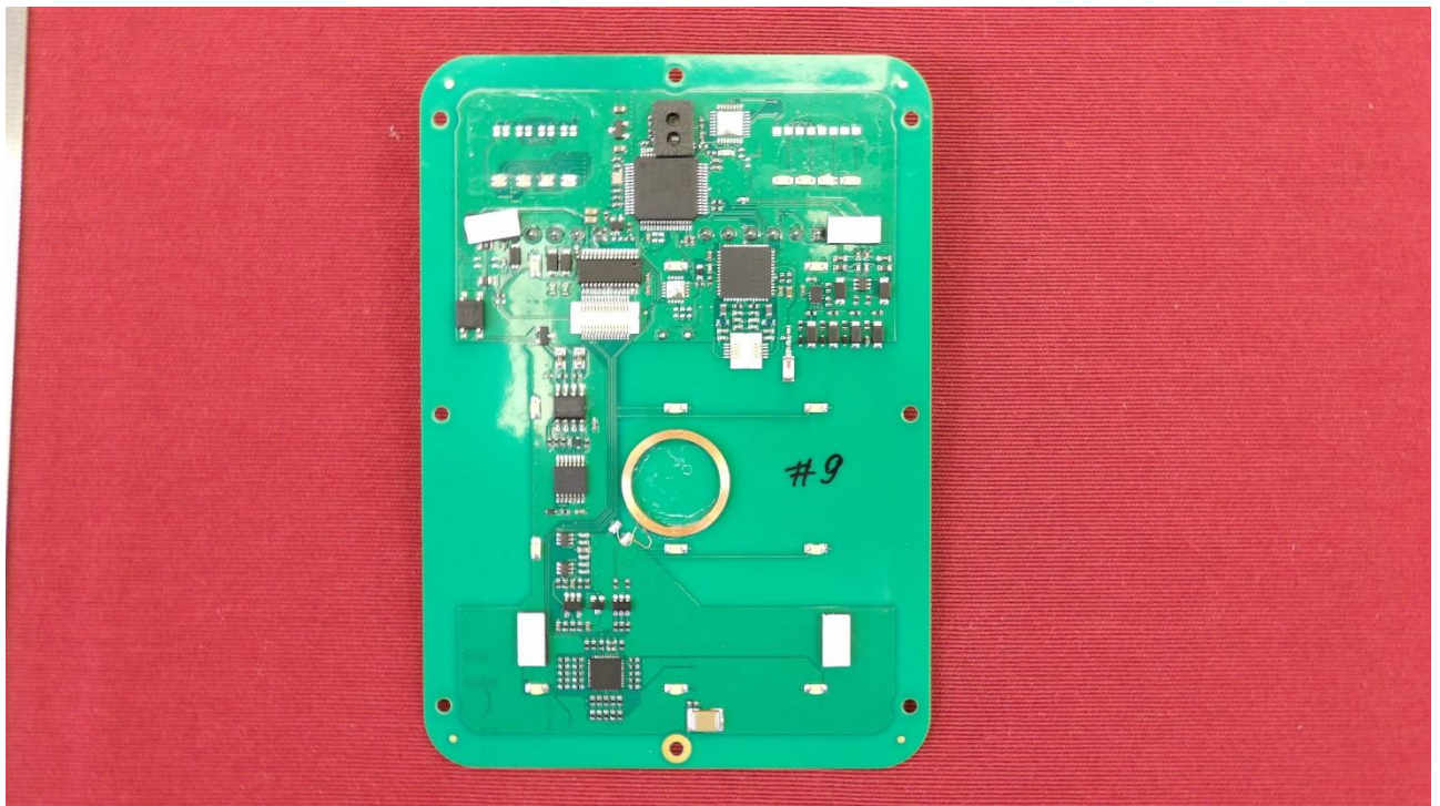
Picture 3: Main PCB – top side
