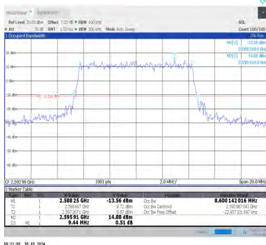
1-N41-30-10-M-3-DFT-16QAM-Outet_Full-24@0-Ant1 1-8.6-9.440-≤10-PASS
