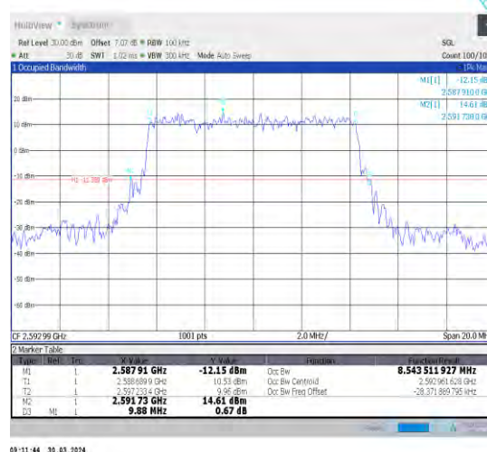
1-N41-30-10-M-2-DFT-PI2BPSK-Outet_Full-24@0-Ant1 nt1-8.544-9.880-≤10-PASS
