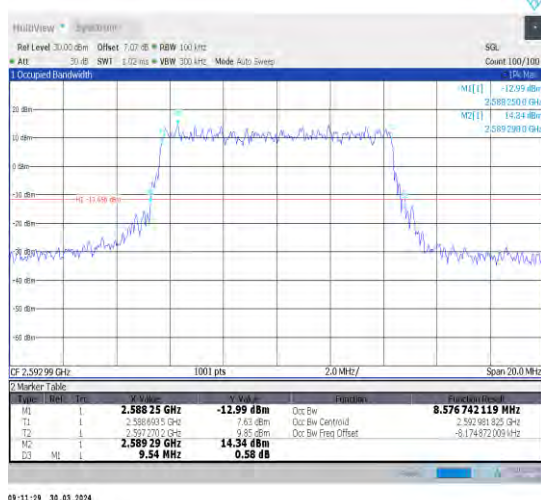
1-N41-30-10-M-1-DFT-QPSK-Outet_Full-24@0-Ant1 -8.577-9.540-≤10-PASS
