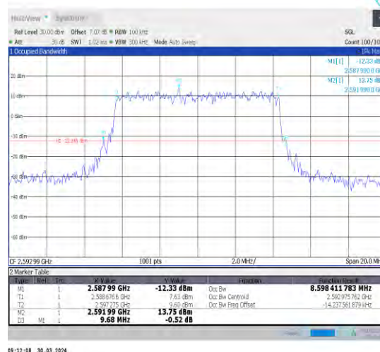
1-N41-30-10-M-4-DFT-64QAM-Outet_Full-24@0-Ant1 1-8.598-9.680-≤10-PASS
