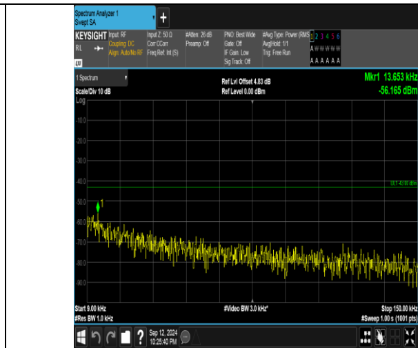
Band4_20MHz_16QAM_20300_100RB#0_0.009~0.15_0.009~0.15
