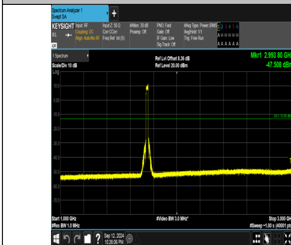
Band4_20MHz_16QAM_20300_100RB#0_1000~3000_1000~3000
