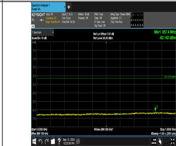
Band4_20MHz_16QAM_20300_100RB#0_30~1000_30~1000
