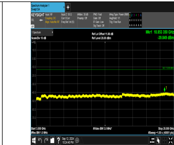
Band4_20MHz_16QAM_20300_1RB#99_3000~20000_3000~20000
