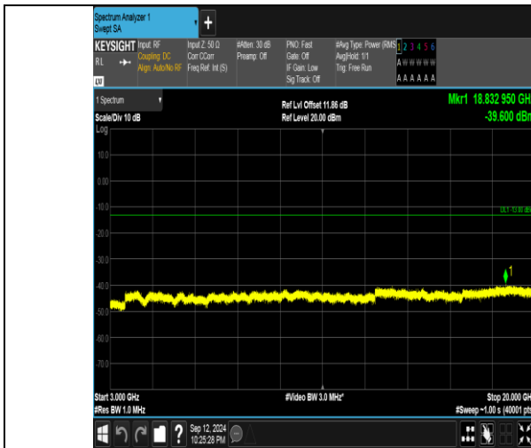
Band4_20MHz_QPSK_20300_100RB#0_3000~20000_3000~20000
