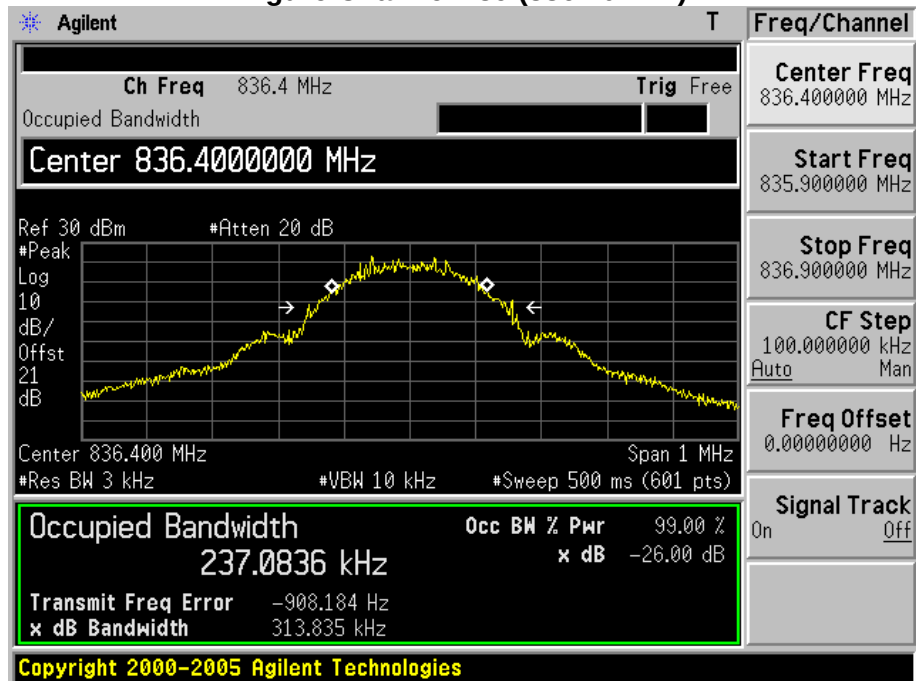
Figure Channel 189 (836.40MHz)
