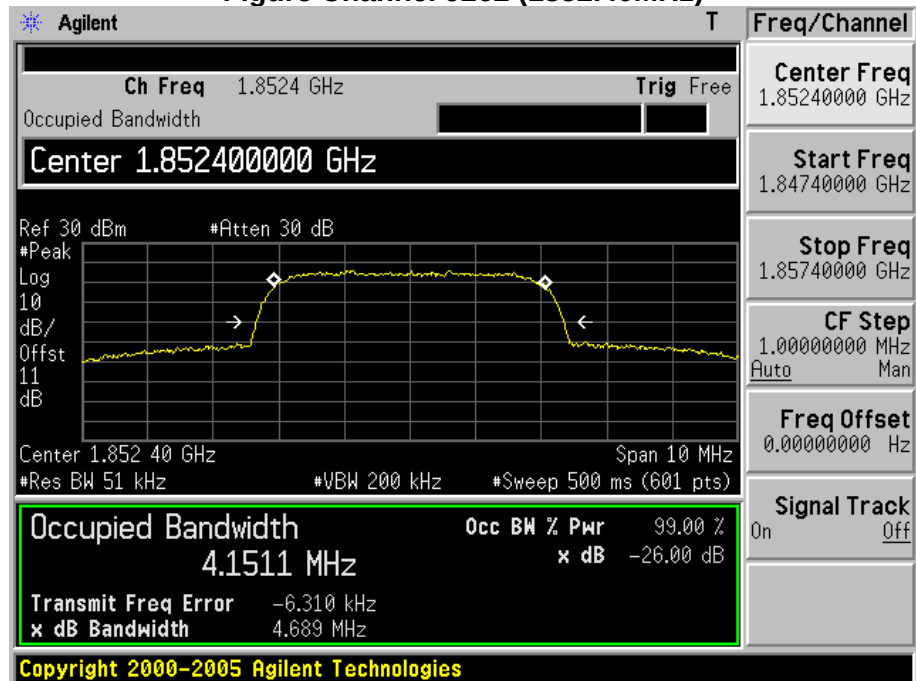
Figure Channel 9262 (1852.40MHz)
