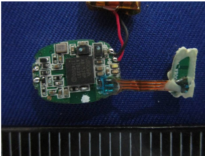
EUT – Left Earbud Board Bottom View
