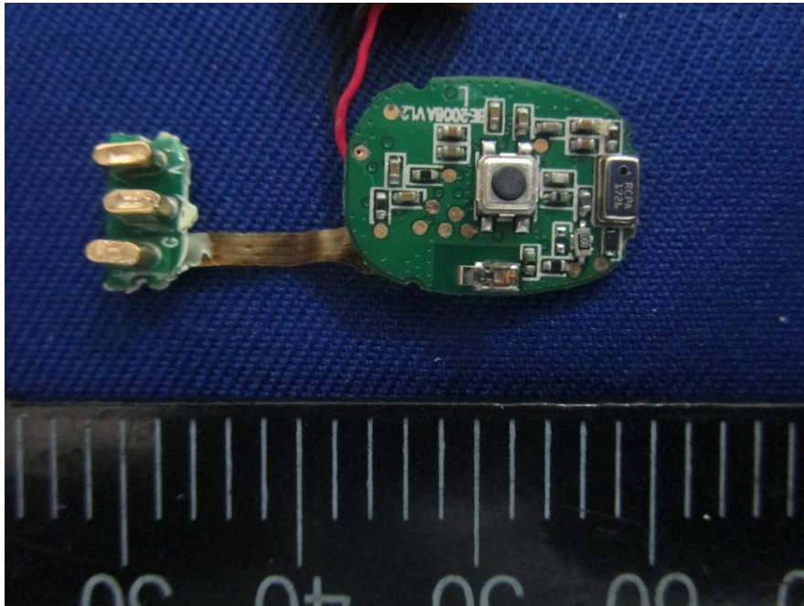
EUT – Left Earbud Board Top View
