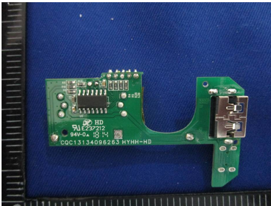
EUT – Main Board Bottom View (Portable Charging Case)
