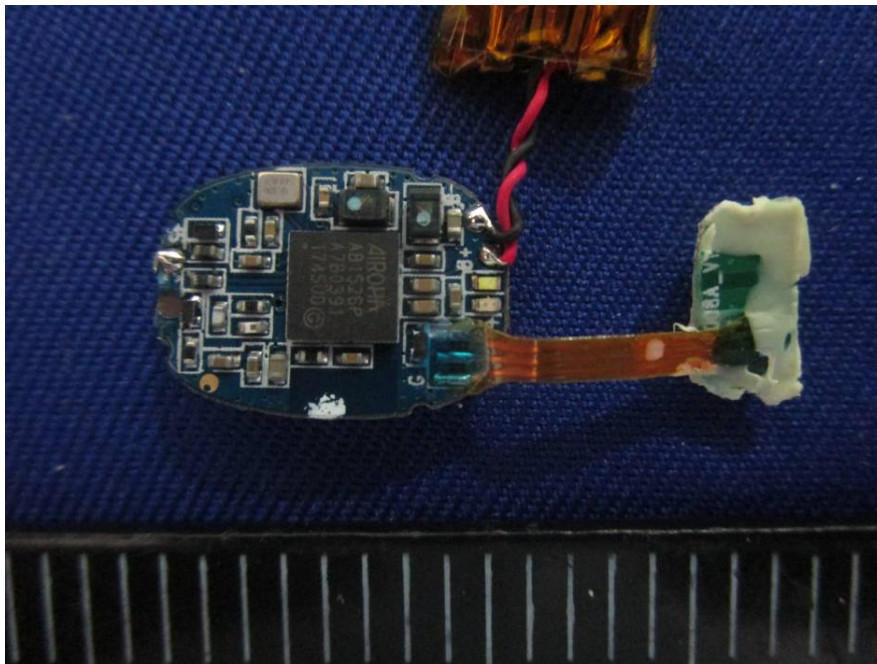
EUT – Right Earbud Board Bottom View
