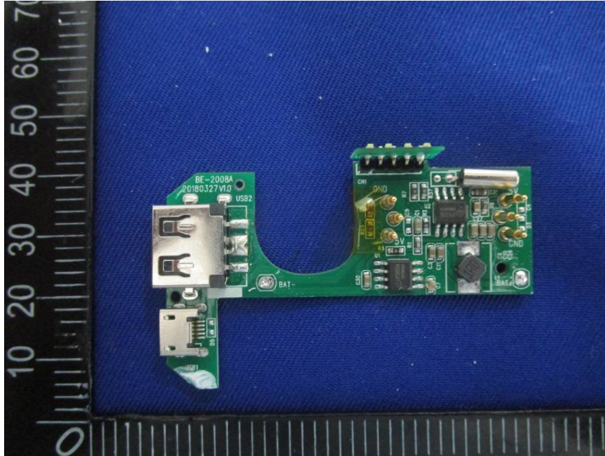
EUT – Main Board Top View (Portable Charging Case)
