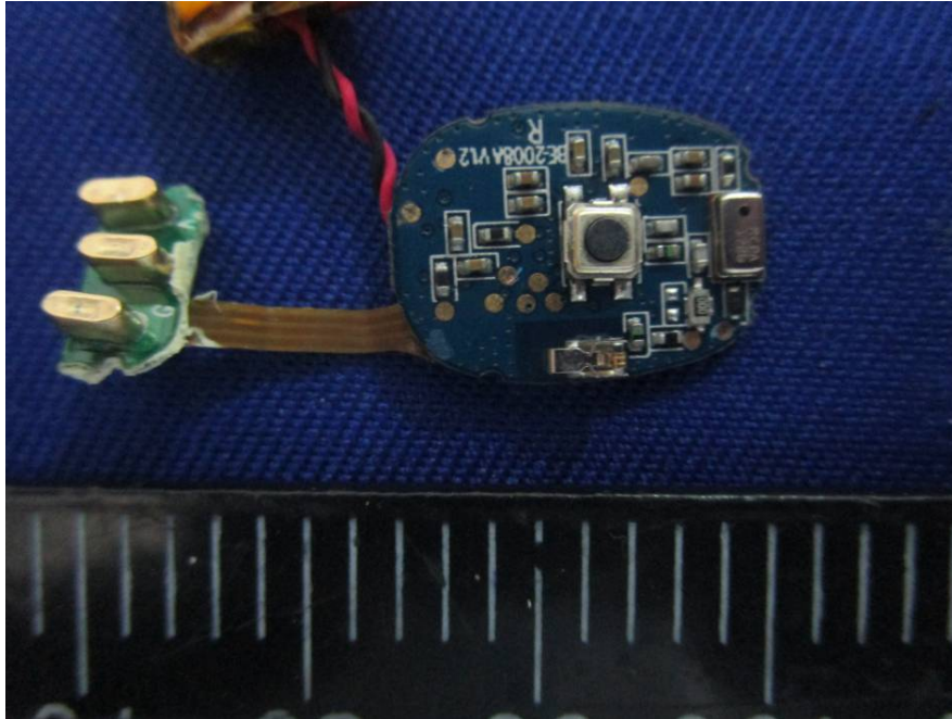
EUT – Right Earbud Board Top View
