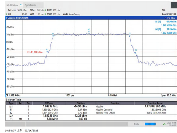
Band2-5MHz-16QAM-18625-25RB#0-PASS
