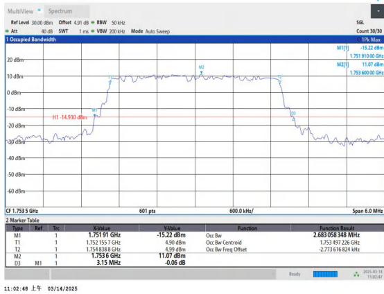
Band4-3MHz-16QAM-20385-15RB#0-PASS
