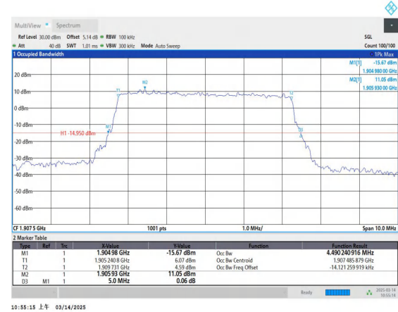
Band2-5MHz-16QAM-19175-25RB#0-PASS
