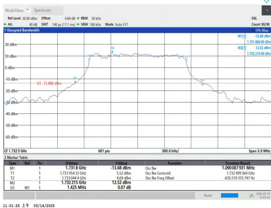
Band4-1.4MHz-QPSK-20175-6RB#0-PASS
