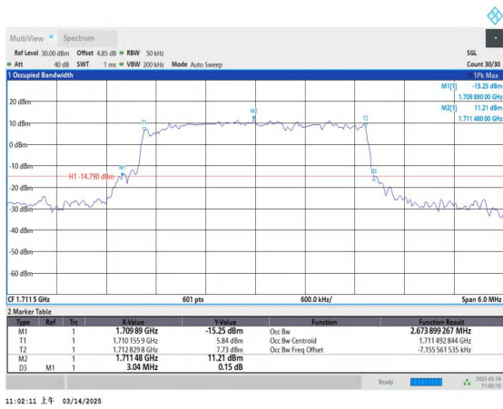
Band4-3MHz-16QAM-19965-15RB#0-PASS
