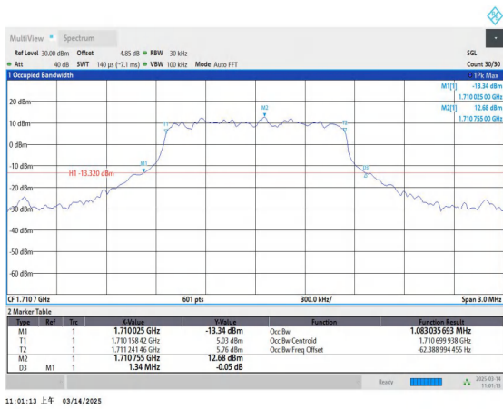
Band4-1.4MHz-16QAM-19957-6RB#0-PASS
