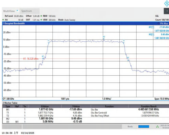
Band2-5MHz-16QAM-18900-25RB#0-PASS
