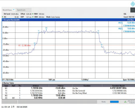
Band4-5MHz-QPSK-20175-25RB#0-PASS
