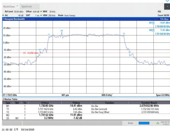
Band4-3MHz-QPSK-20175-15RB#0-PASS
