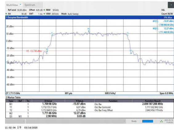
Band4-3MHz-QPSK-19965-15RB#0-PASS
