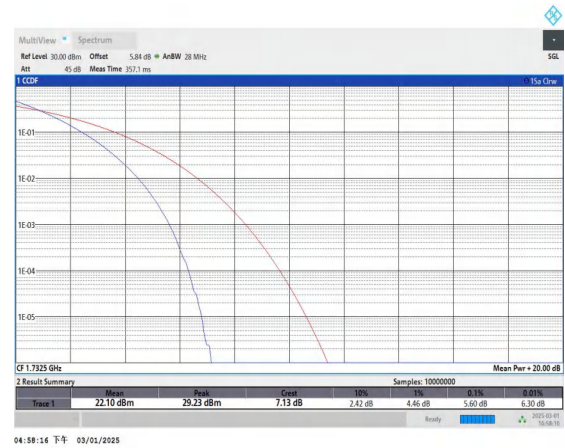
Band4-20MHz-QPSK-20175-100RB#0-PASS
