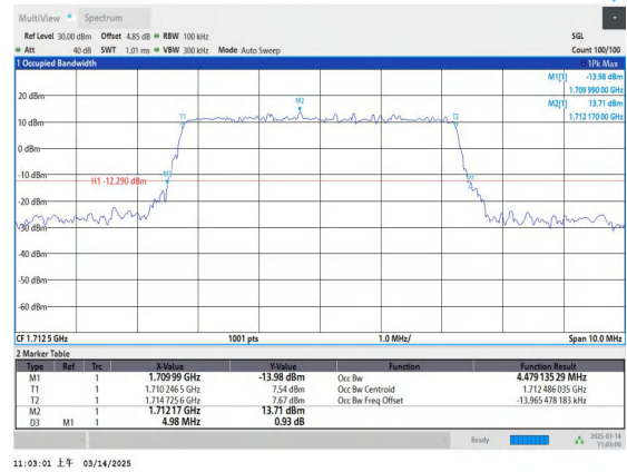
Band4-5MHz-QPSK-19975-25RB#0-PASS
