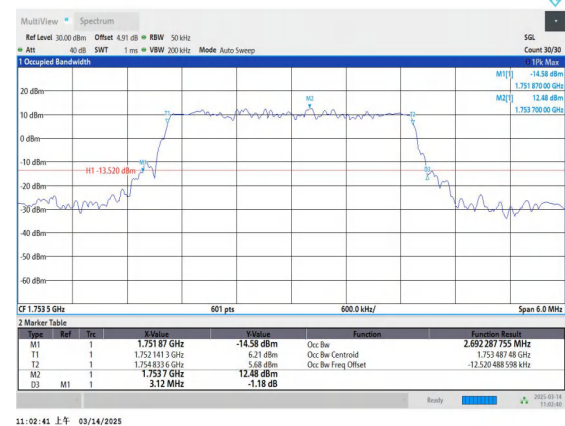
Band4-3MHz-QPSK-20385-15RB#0-PASS
