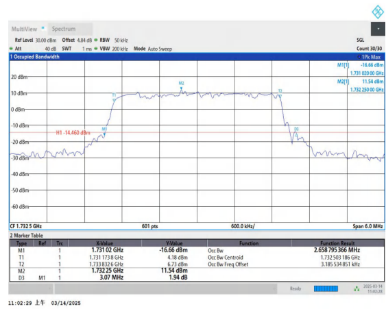
Band4-3MHz-16QAM-20175-15RB#0-PASS
