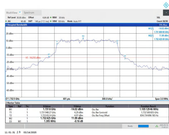
Band4-1.4MHz-16QAM-20175-6RB#0-PASS
