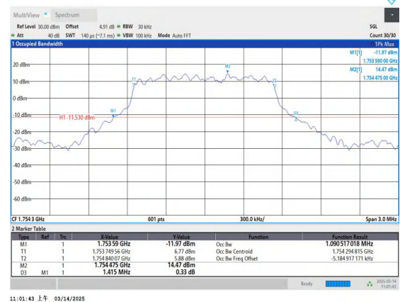
Band4-1.4MHz-QPSK-20393-6RB#0-PASS
