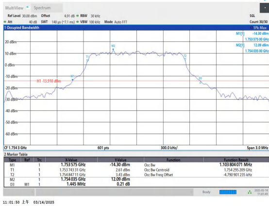
Band4-1.4MHz-16QAM-20393-6RB#0-PASS
