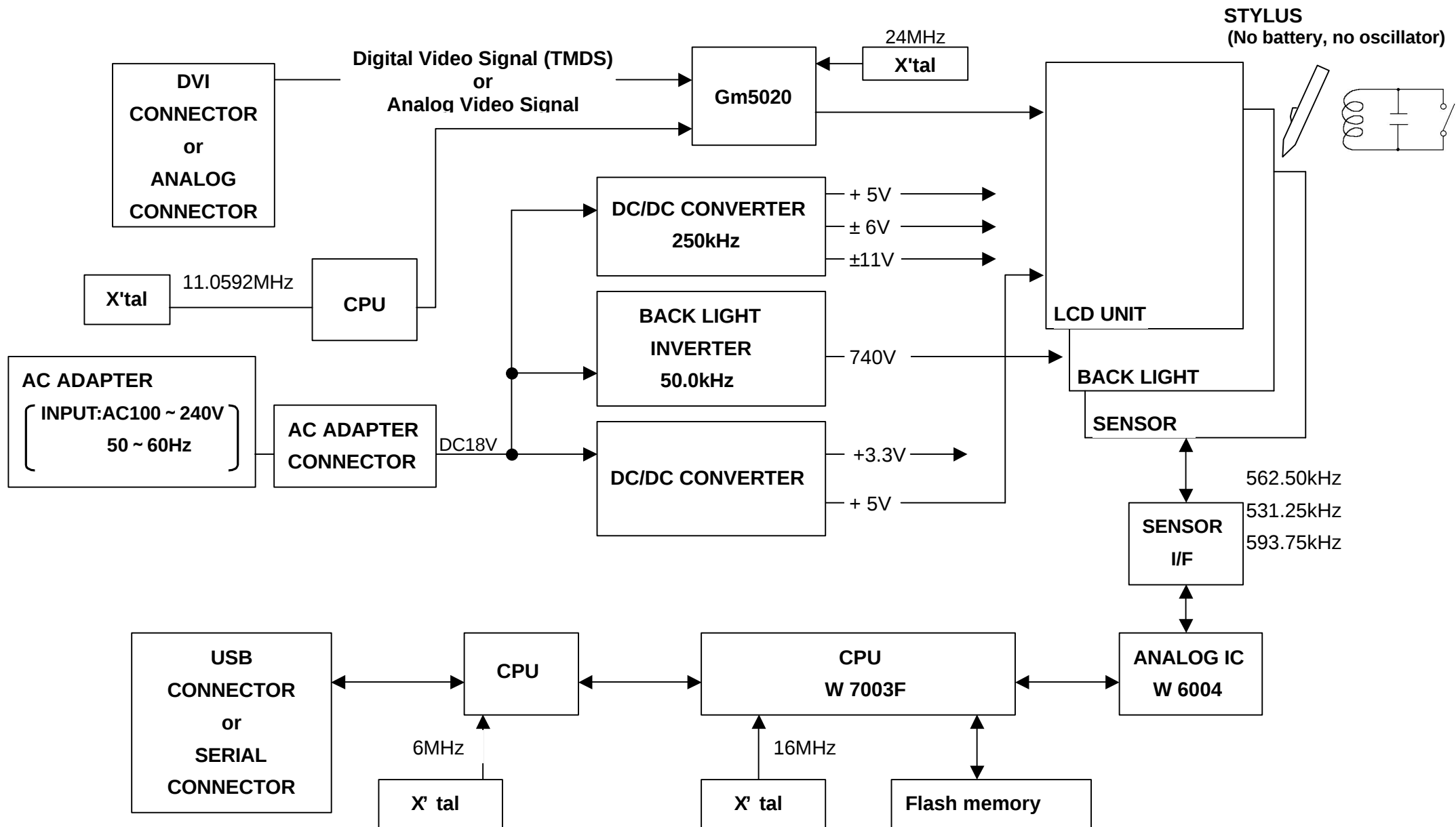
< PL - 800 Block Diagram >
