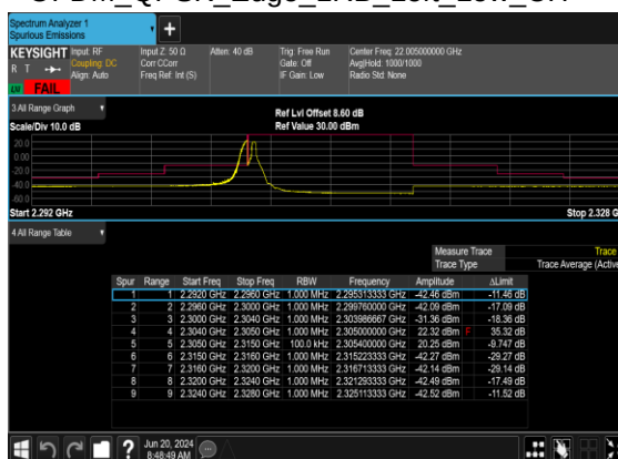
B5_N30(10M)_DFT-s- OFDM_QPSK_Edge_1RB_Left_Low_CH
