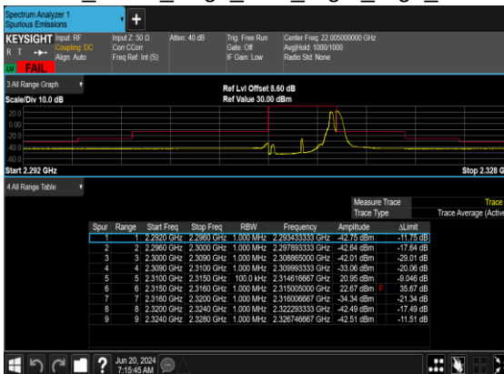
B5_N30(5M)_DFT-s- OFDM_BPSK_Edge_1RB_Right_High_CH
