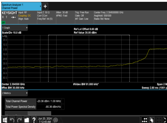
B5_N30(5M)_DFT-s- OFDM_QPSK_Outer_Full_Low_CH_CH_P SS
