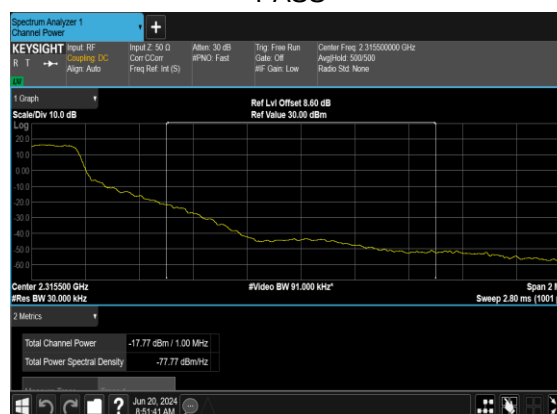
B5_N30(10M)_DFT-s- OFDM_BPSK_Edge_1RB_Right_Low_CH_CHP_ PASS
