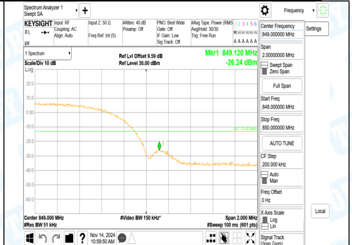
Band5-4233-5-PASS
