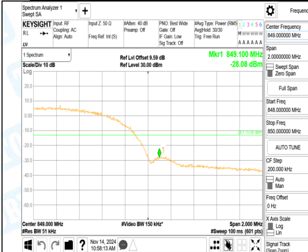
Band5-4233-4-PASS
