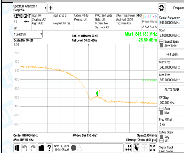
Band5-4233-4-PASS
