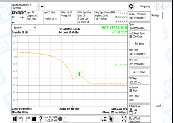
Band5-4233-5-PASS
