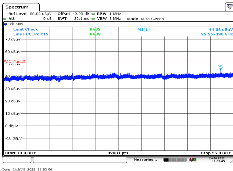
Plot 4: 18 GHz to 26 GHz, vertical & horizontal polarization, valid for all modes and channels of both antennas
