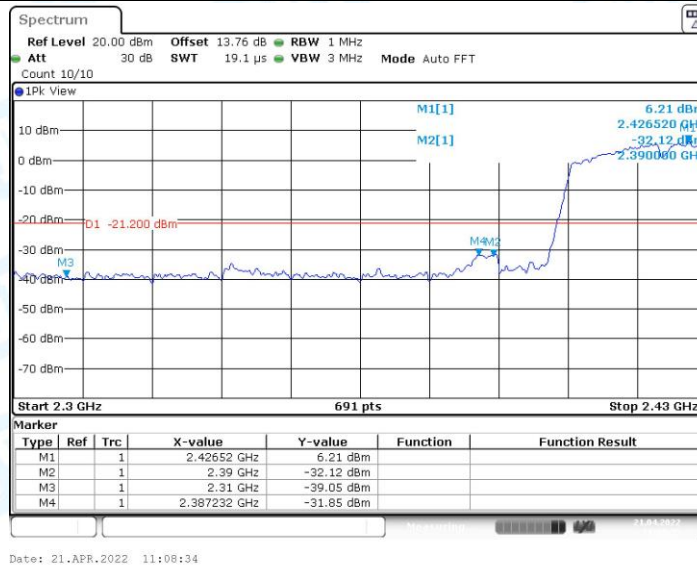
11N40SISO_Ant1_Low_2422_Peak
