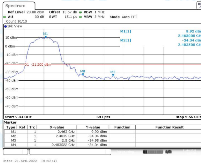
11G_Ant1_High_2462_Peak
