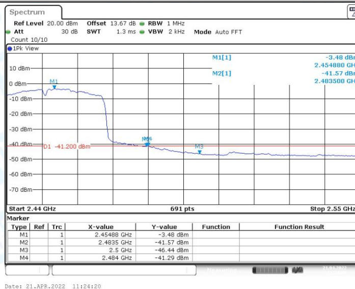
11N40SISO_Ant1_High_2452_AV
