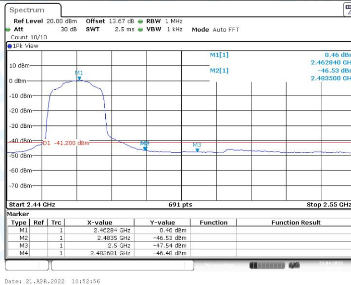
11G_Ant1_High_2462_AV
