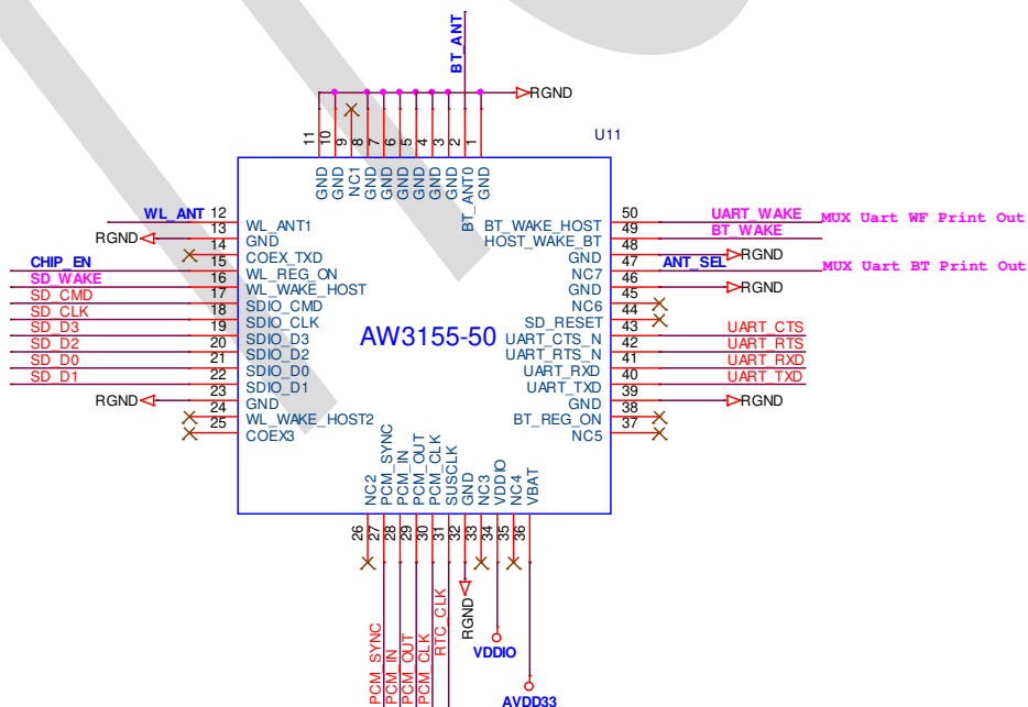
Figure 3. Application Circuit Diagram of AW3155-50
