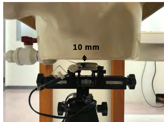
Fig.9 EUT Back side (headset) to flat phantom
