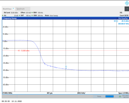
Band5-10MHz-16QAM-20600-50RB#0
