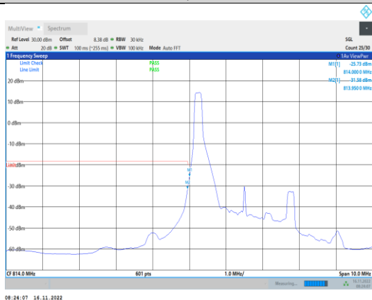
Band26-3MHz-64QAM-26705-1RB#0
