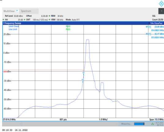
Band26-1.4MHz-64QAM-26697-1RB#0
