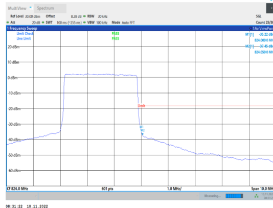
Band26-3MHz-QPSK-26775-15RB#0
