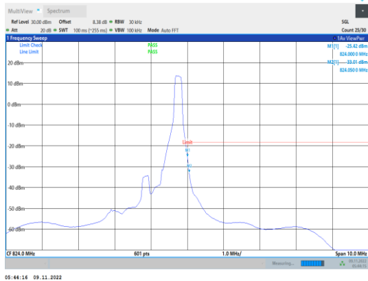
Band26-1.4MHz-16QAM-26783-1RB#5
