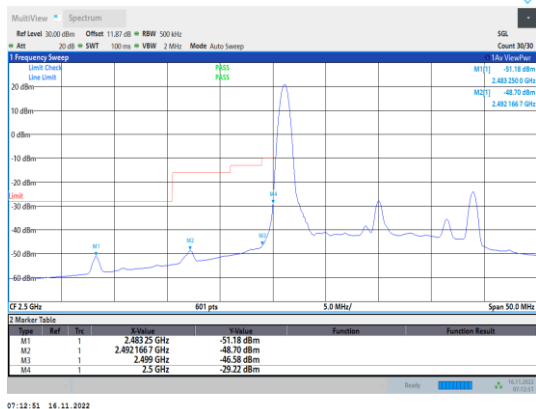
Band7-20MHz-64QAM-20850-1RB#0
