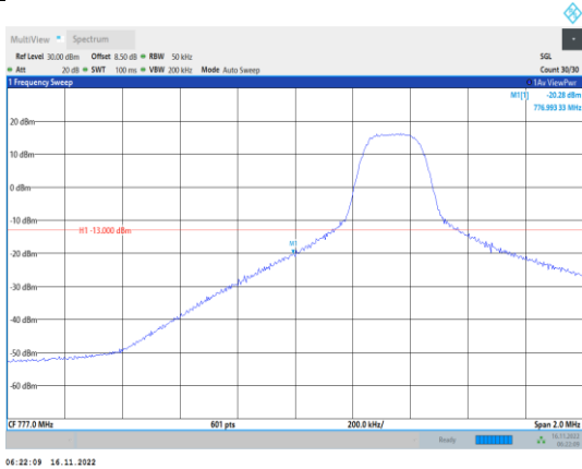
Band13-5MHz-64QAM-23205-1RB#0
