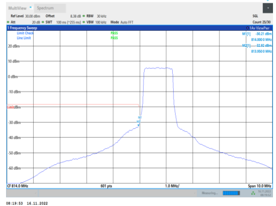
Band26-1.4MHz-64QAM-26697-6RB#0
