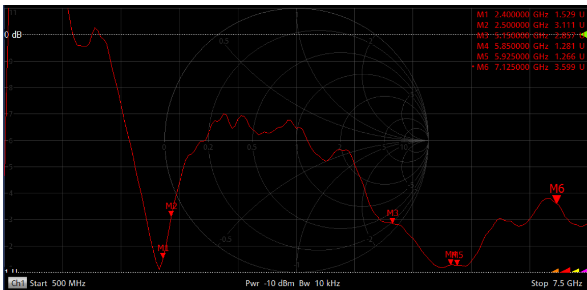
WiFi2 5GHz Antenna
