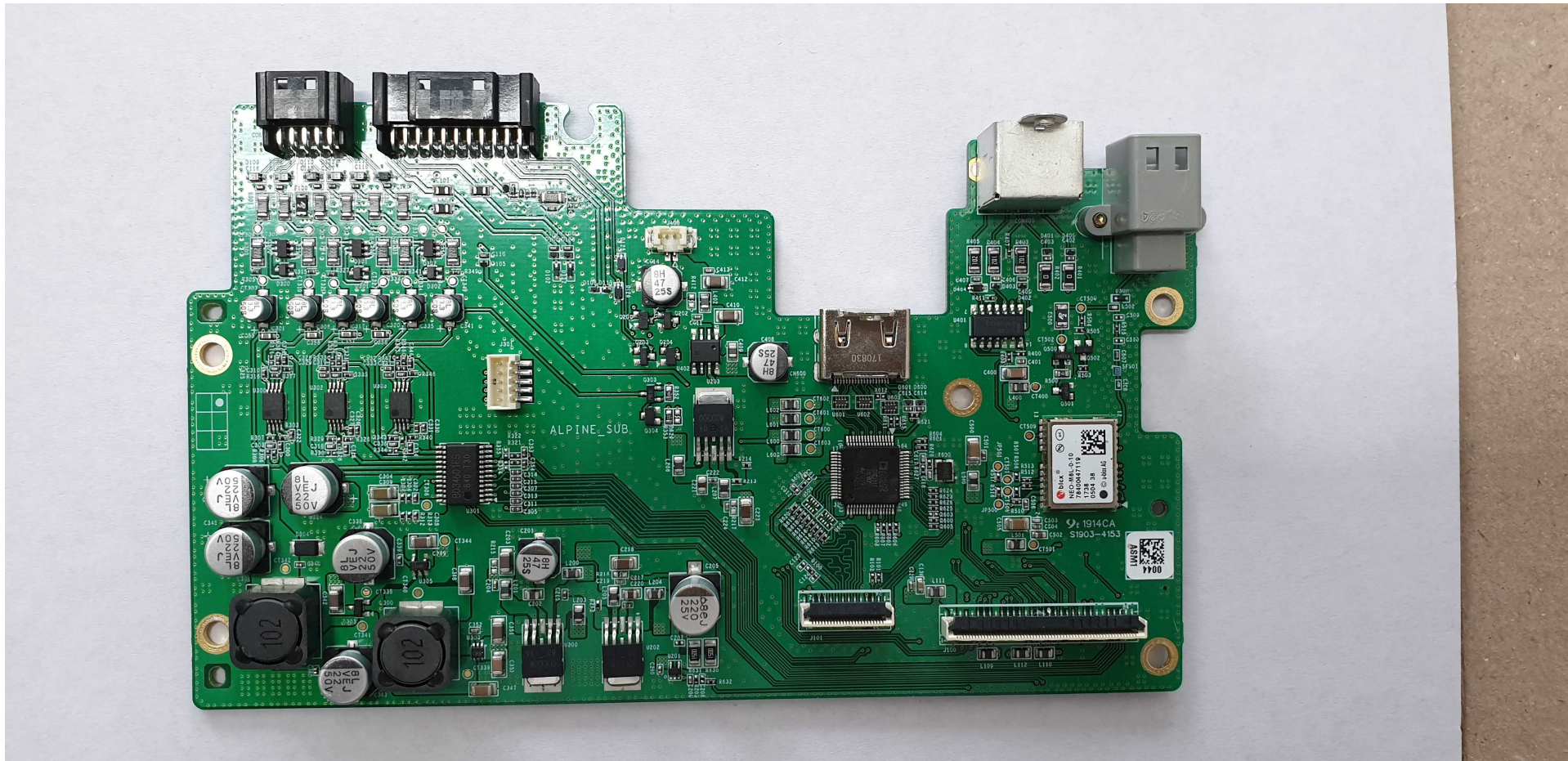
[SUB Board (Top)]
