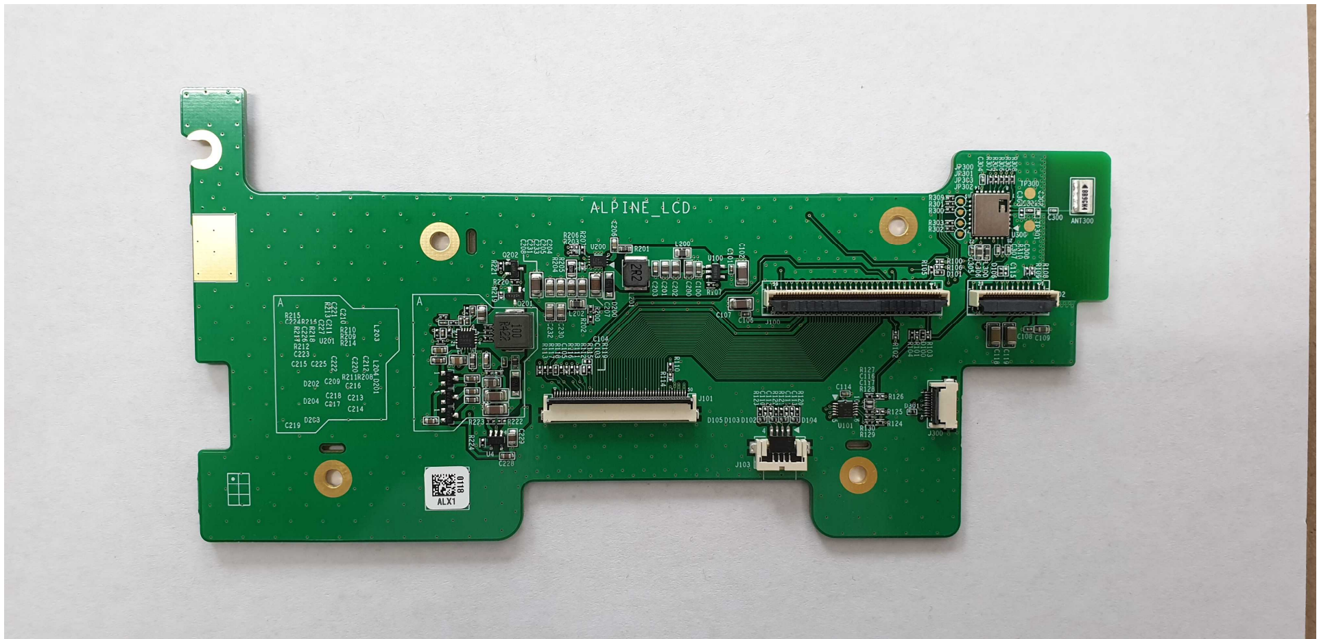
[LCD Board (Bottom)]
