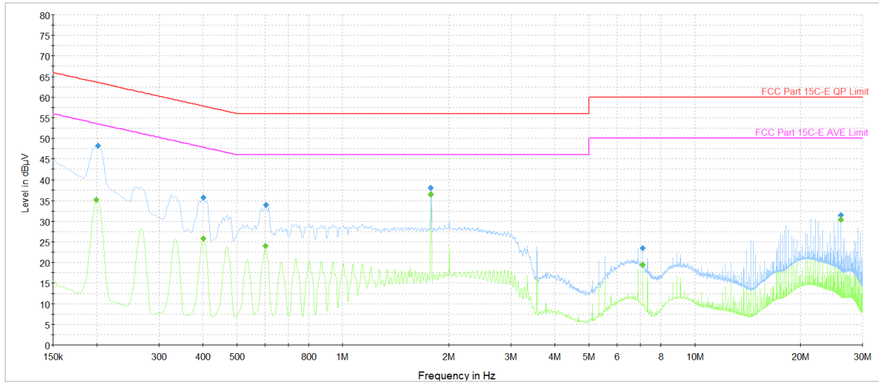
Plot 7-39. AC Line Conducted Plot with Bluetooth HDR (L1, 4Mbps ePA - Ch.38 with Laptop + Magnetic Charger)
