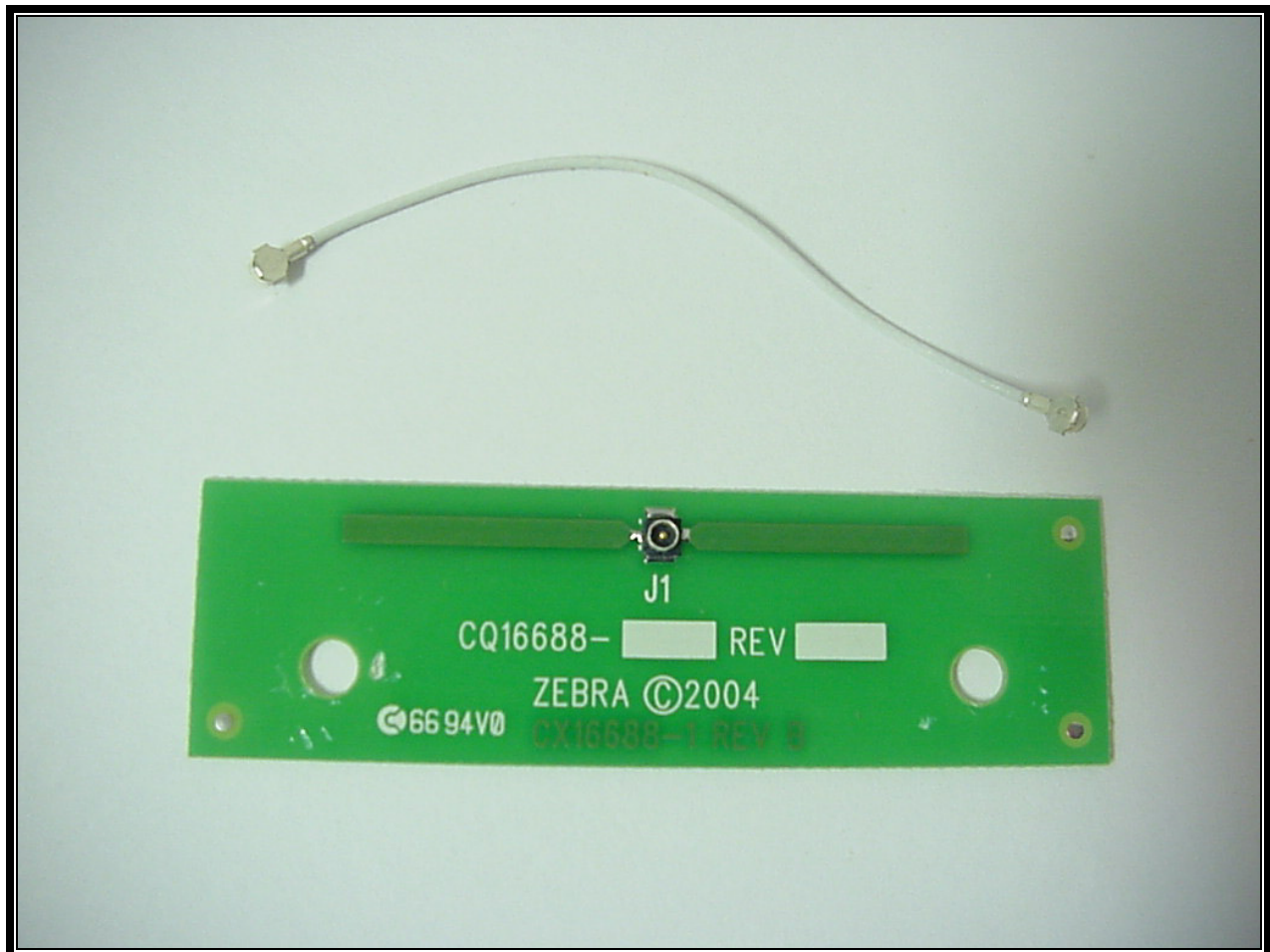
PHOTOGRAPH 11: FRONT OF CQ16688 SHOWING CABLE USED IN TESTING
