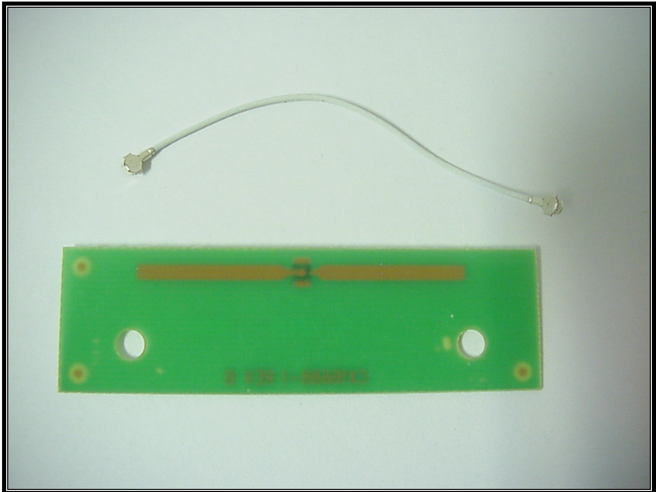
PHOTOGRAPH 12: BACK OF CQ16688 SHOWING CABLE USED IN TESTING
