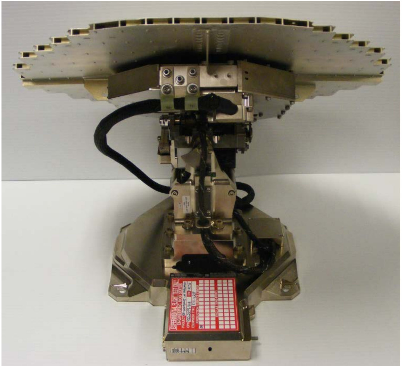
Figure C-2 – RTA-4218 External Photograph - Bottom
