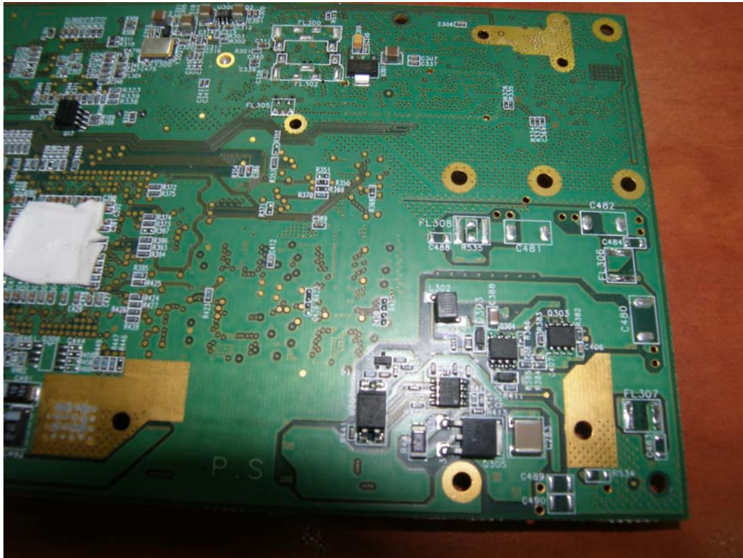
Photo5. PCB print side
