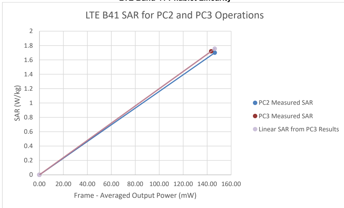
Figure 13-7 LTE Band 41 Phablet Linearity
