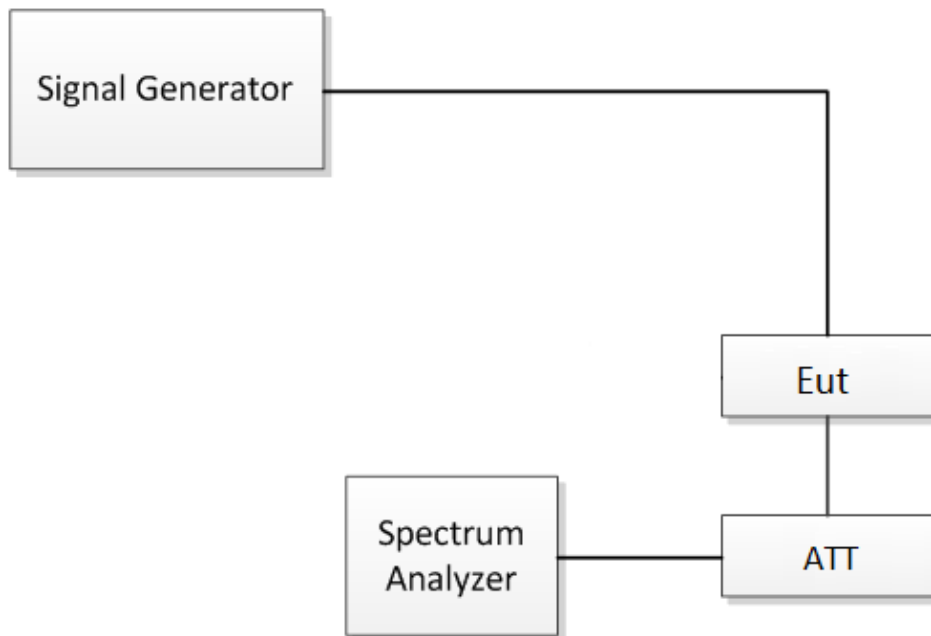
Fig.1 RF Output Power test configuration
