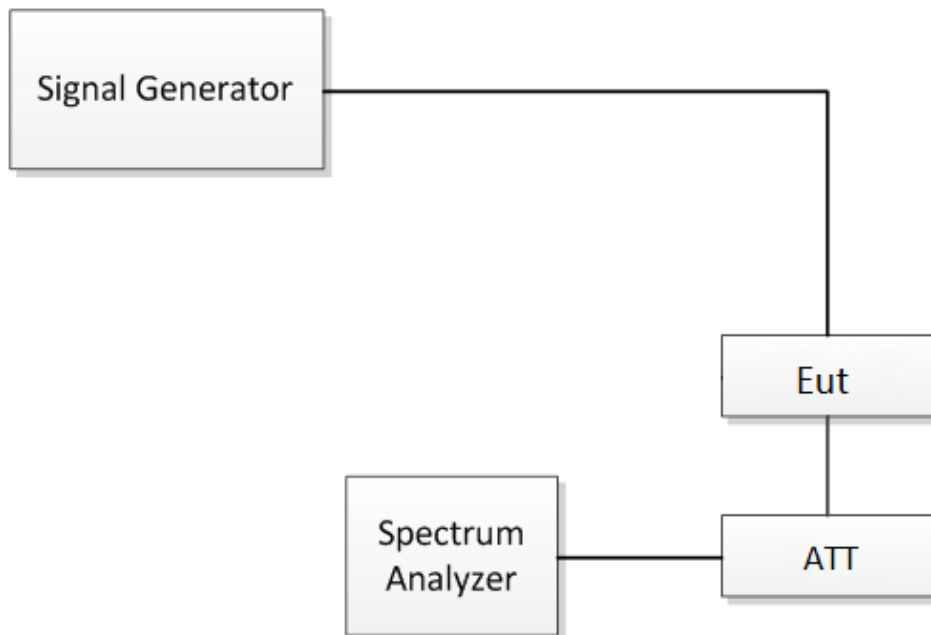
Fig.4. Occupied bandwidth test configuration
