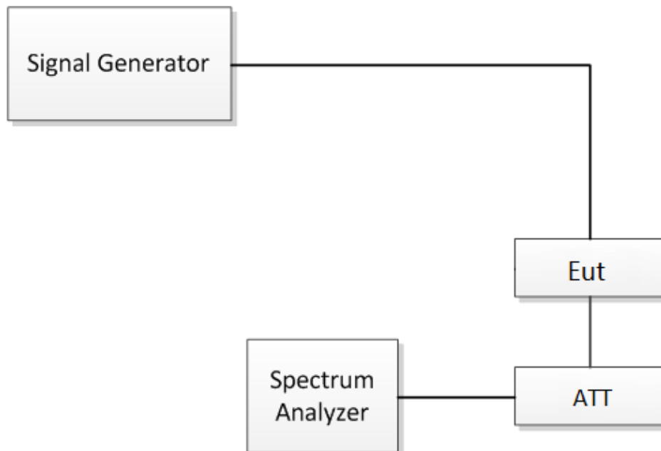
Fig.5. Out of Band rejection test configuration
