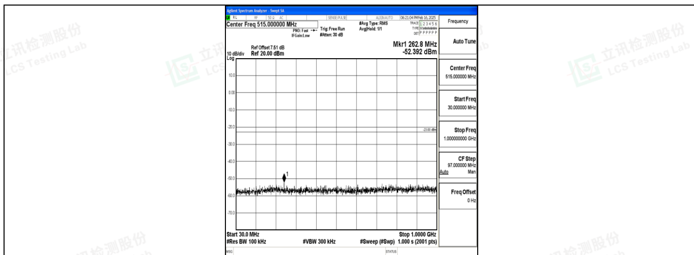
Band2_5MHz_QPSK_19175_1RB#0_30~1000_30~1000
