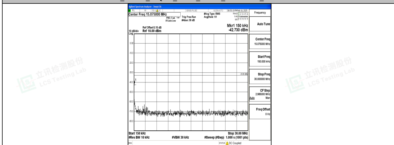
Band2_15MHz_16QAM_18675_1RB#0_0.15~30_0.15~30
