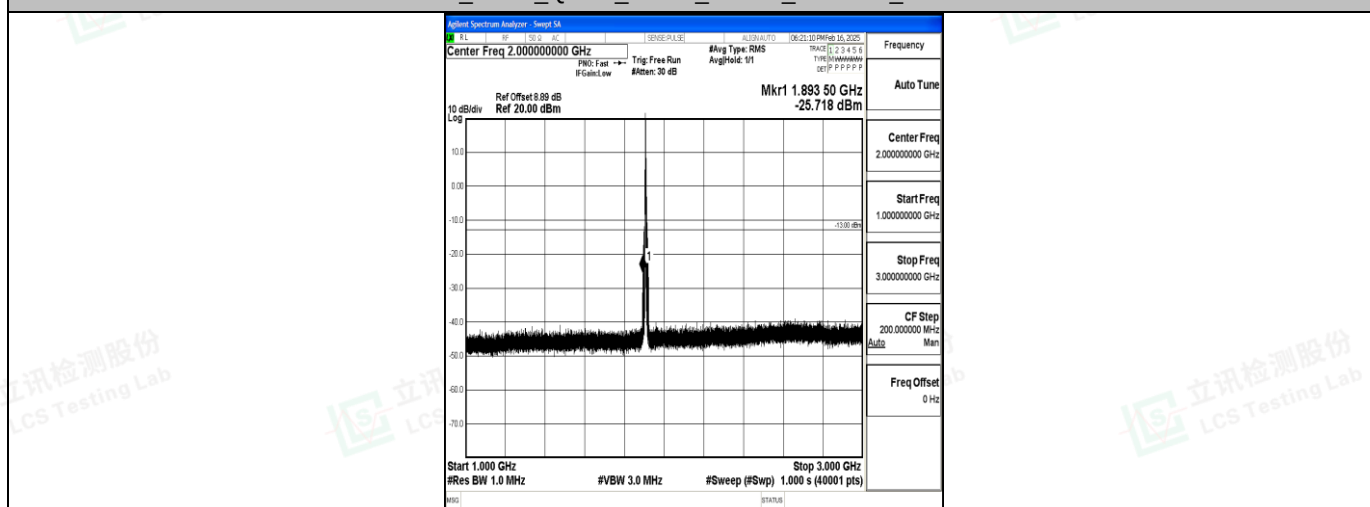
Band2_5MHz_QPSK_19175_1RB#0_1000~3000_1000~3000
