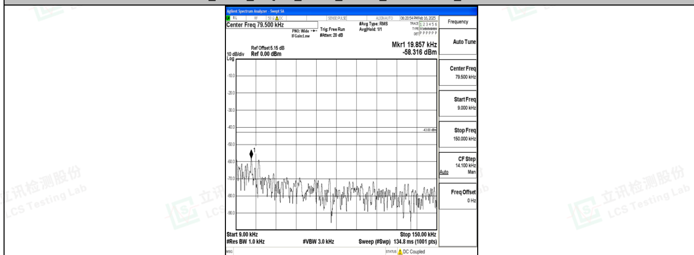
Band2_5MHz_QPSK_19175_1RB#0_0.009~0.15_0.009~0.15
