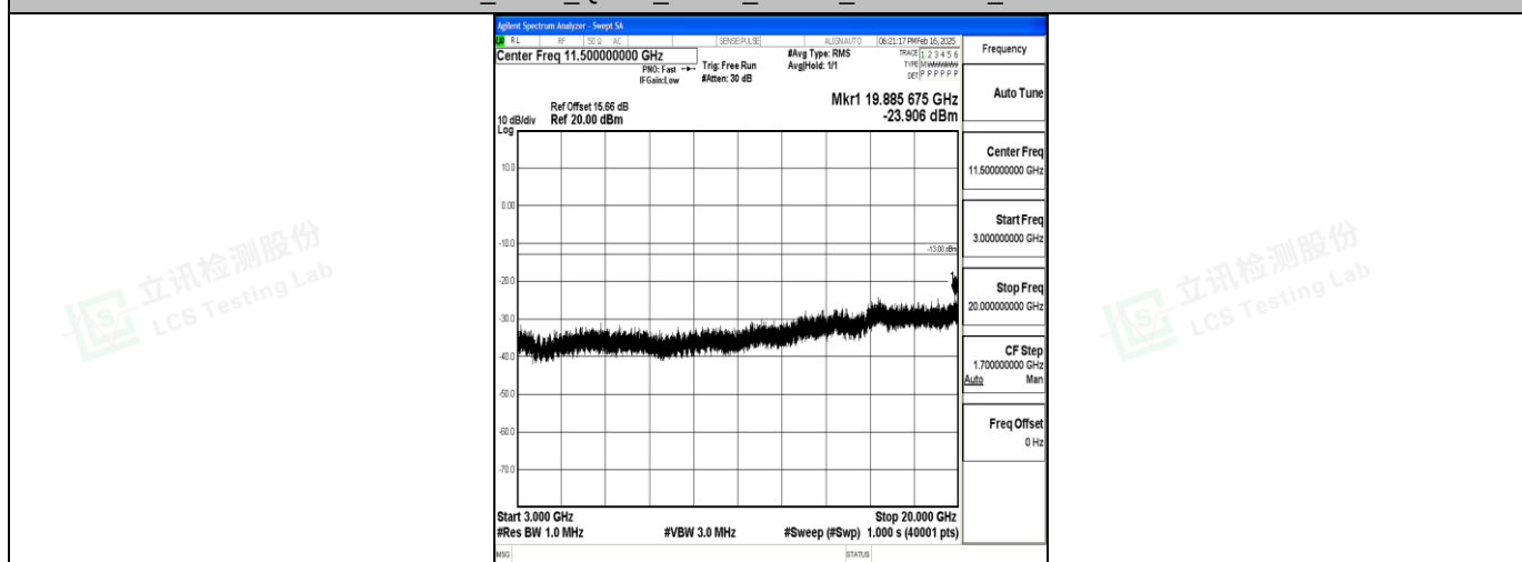
Band2_5MHz_QPSK_19175_1RB#0_3000~20000_3000~20000
