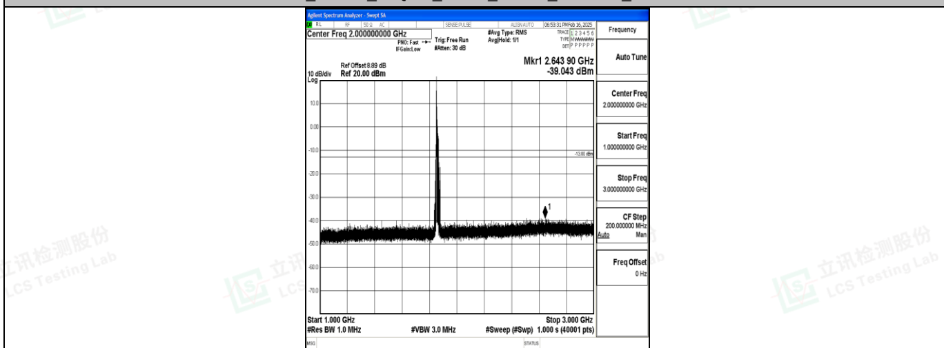
Band2_15MHz_16QAM_18675_1RB#0_1000~3000_1000~3000
