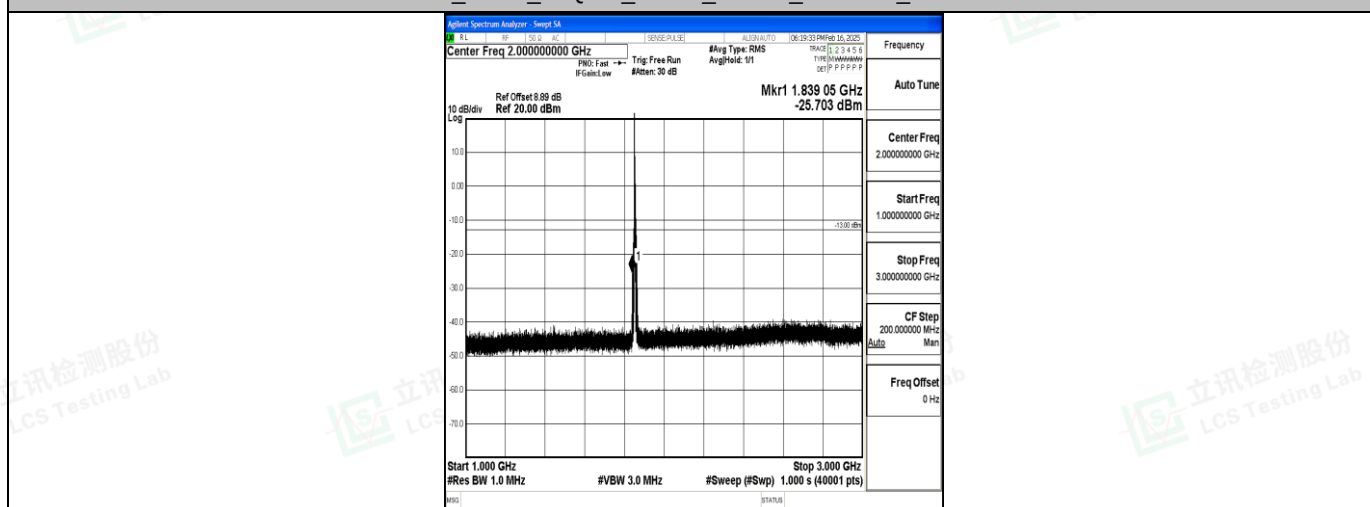
Band2_5MHz_16QAM_18625_1RB#0_1000~3000_1000~3000
