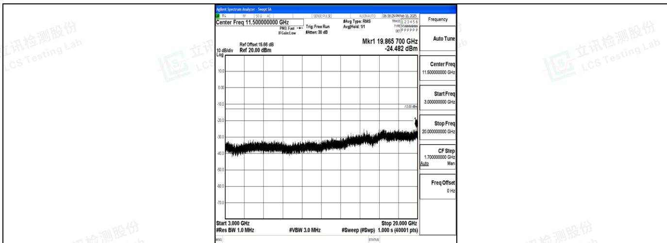
Band2_10MHz_16QAM_18900_1RB#0_3000~20000_3000~20000
