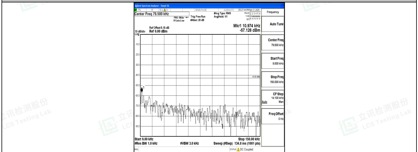
Band2_3MHz_QPSK_19185_1RB#0_0.009~0.15_0.009~0.15
