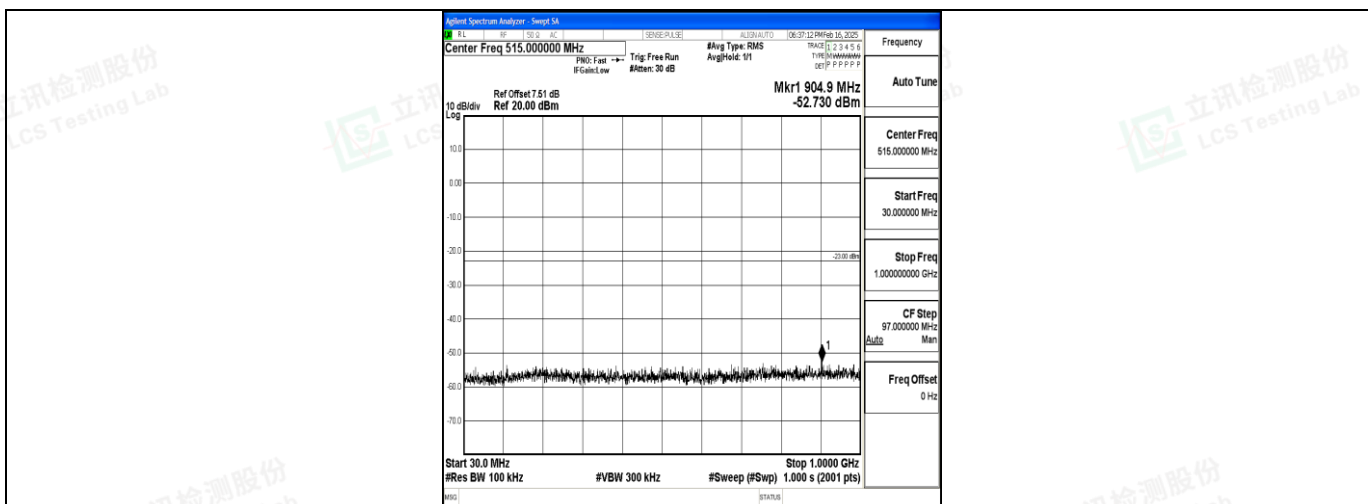
Band2_10MHz_16QAM_18650_1RB#0_30~1000_30~1000
