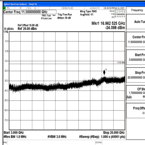
Band2_10MHz_QPSK_18650_1RB#0_3000~20000_3000~20000
