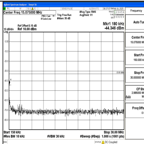
Band2_10MHz_16QAM_18650_1RB#0_0.15~30_0.15~30
