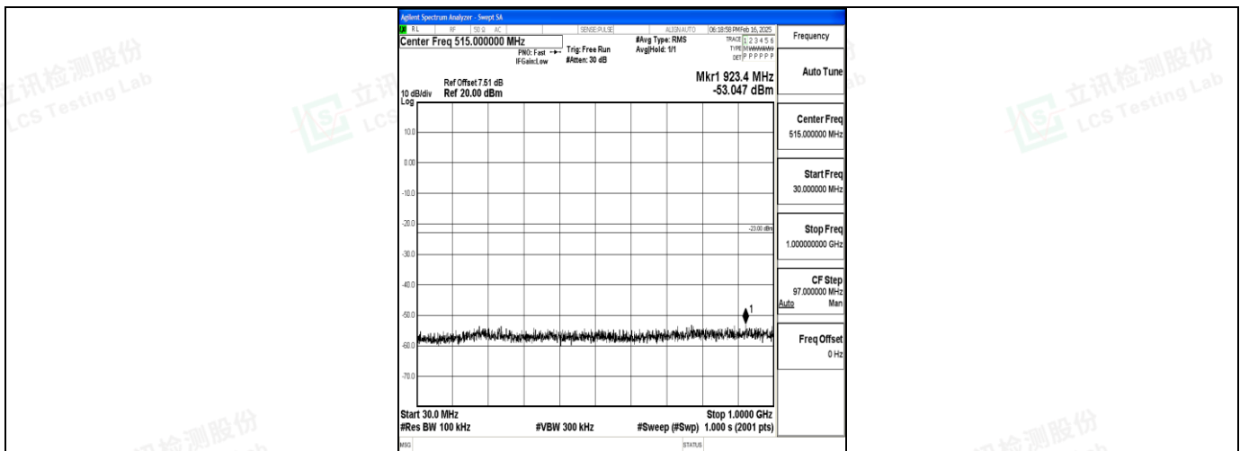
Band2_5MHz_QPSK_18625_1RB#0_30~1000_30~1000
