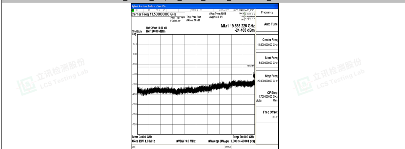
Band2_15MHz_16QAM_18675_1RB#0_3000~20000_3000~20000
