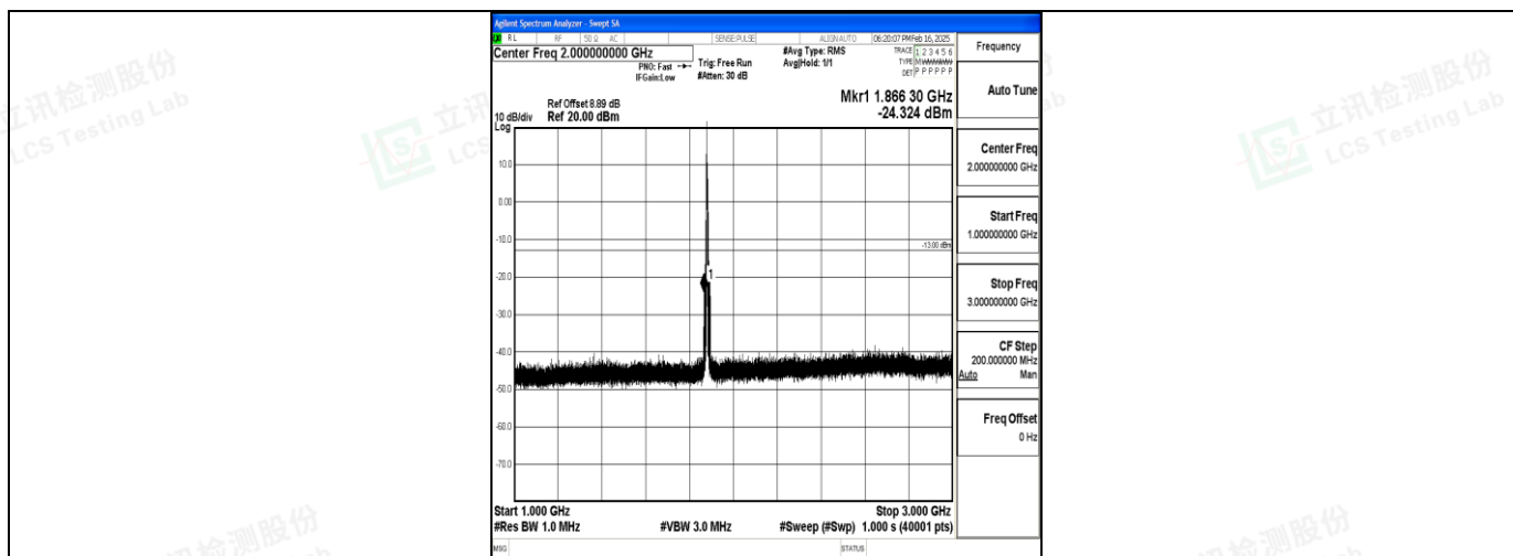
Band2_5MHz_QPSK_18900_1RB#0_1000~3000_1000~3000
