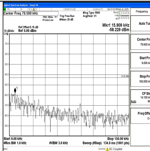
Band2_10MHz_16QAM_18650_1RB#0_0.009~0.15_0.009~0.15
