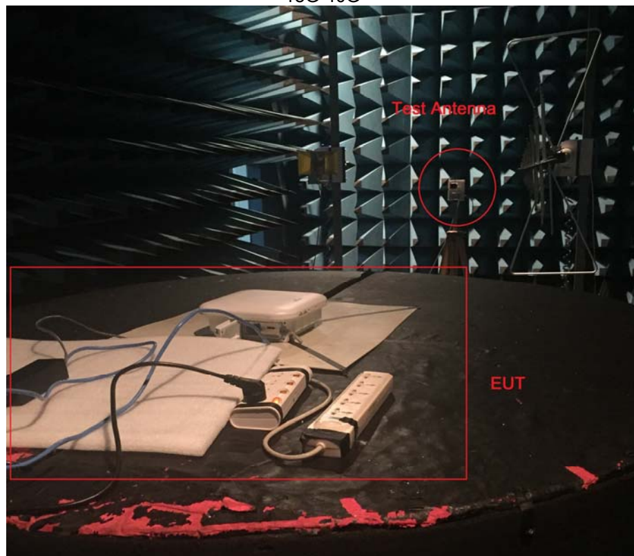
18G-40G
