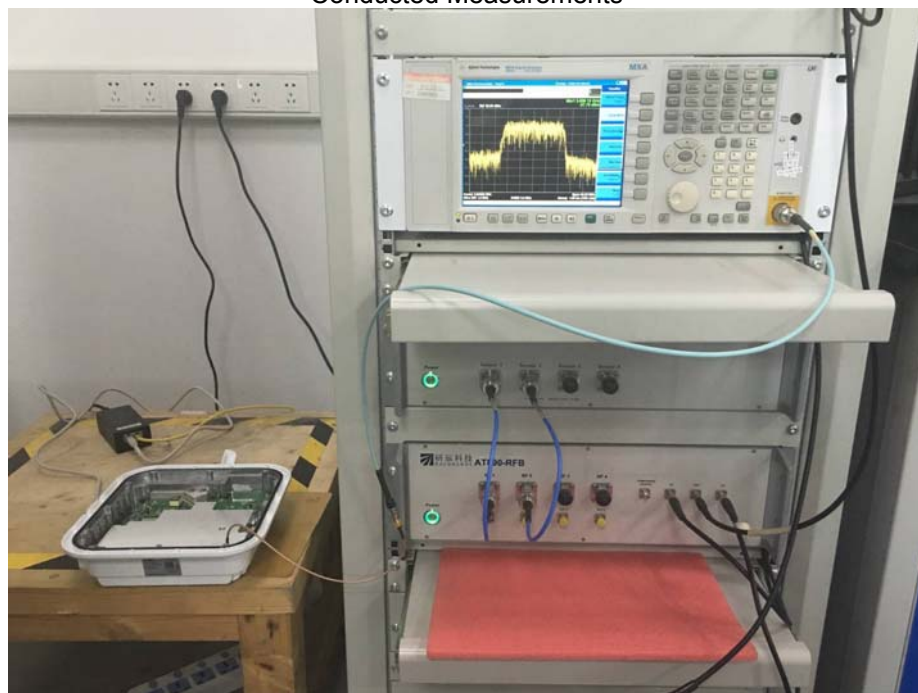
Conducted Measurements
