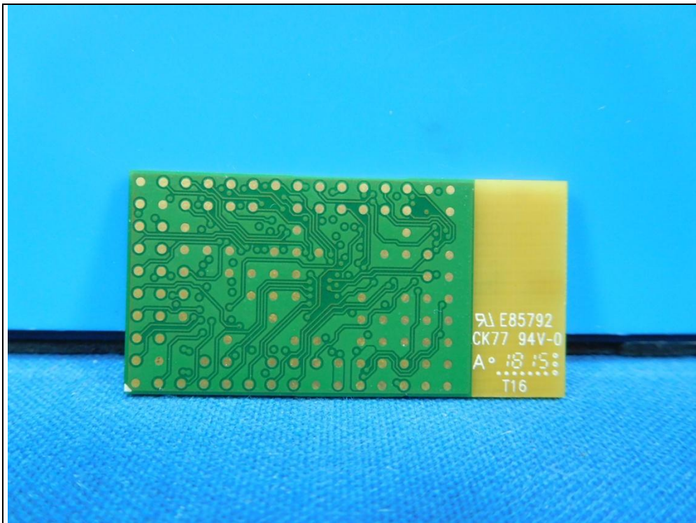
Flash chip No. 1 (Brand: Winbond, Model: W25Q32 series)
