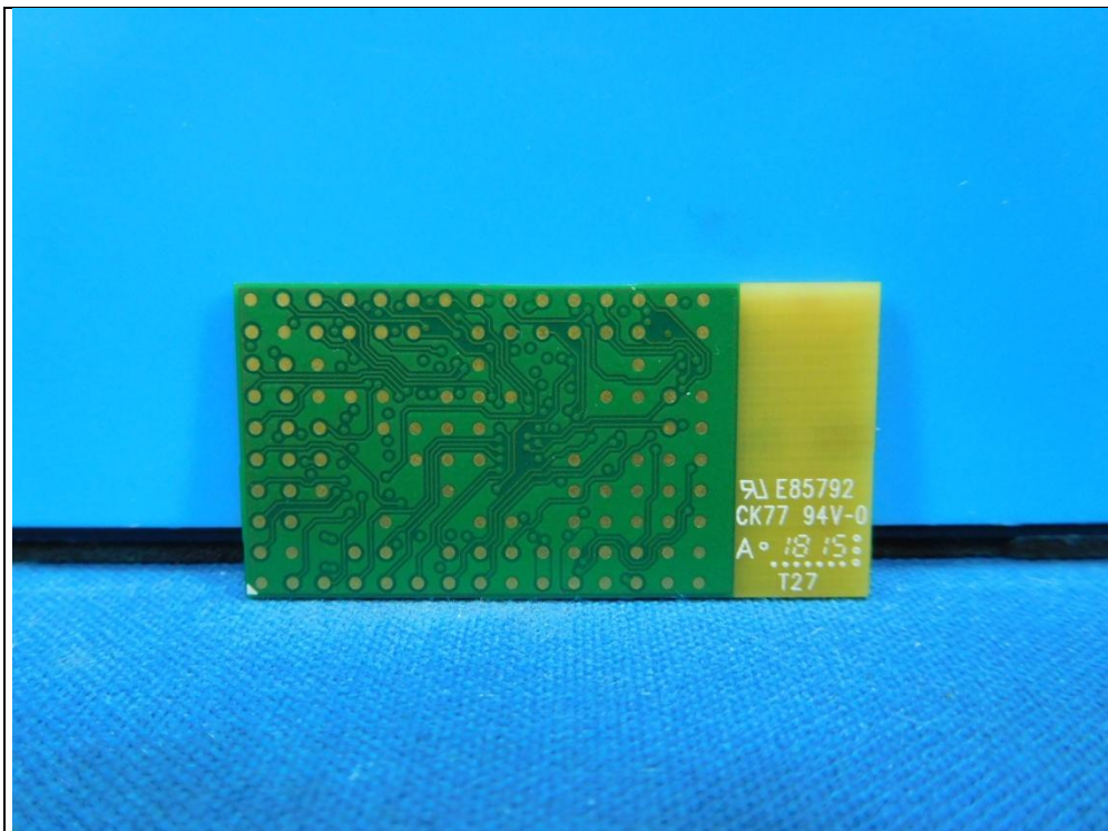
Flash chip No. 2 (Brand: GigaDevice, Model: GD25Q32 series)
