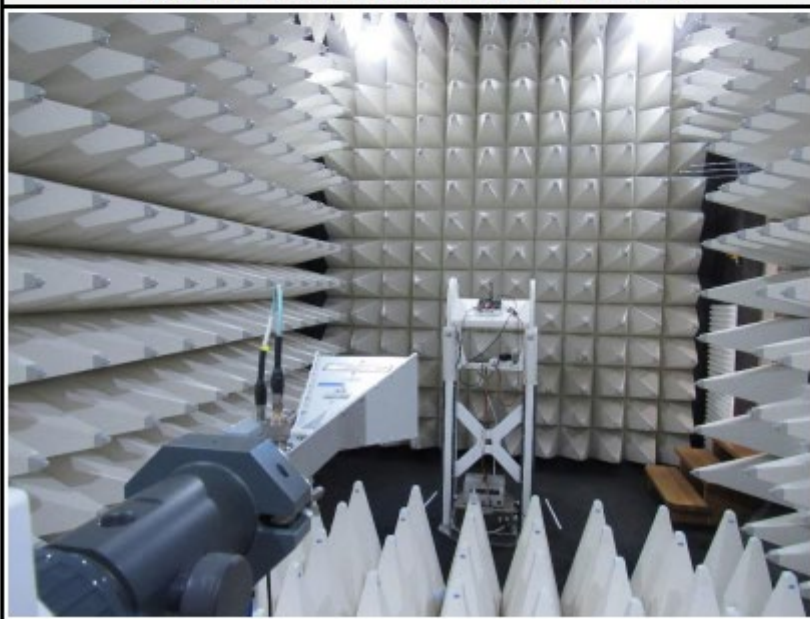
Setup for measurements above 1 GHz-Antenna 1
