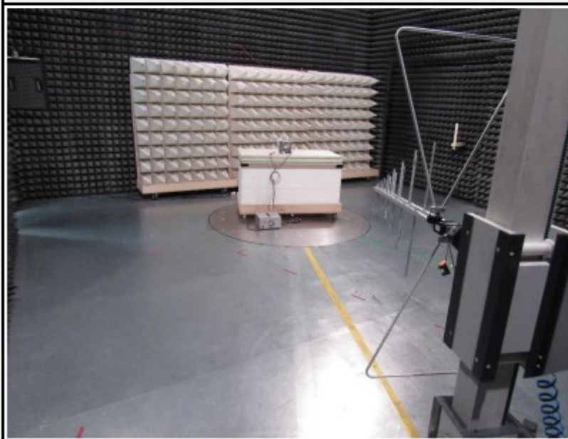
Setup for measurements below 1 GHz- Antenna 2
