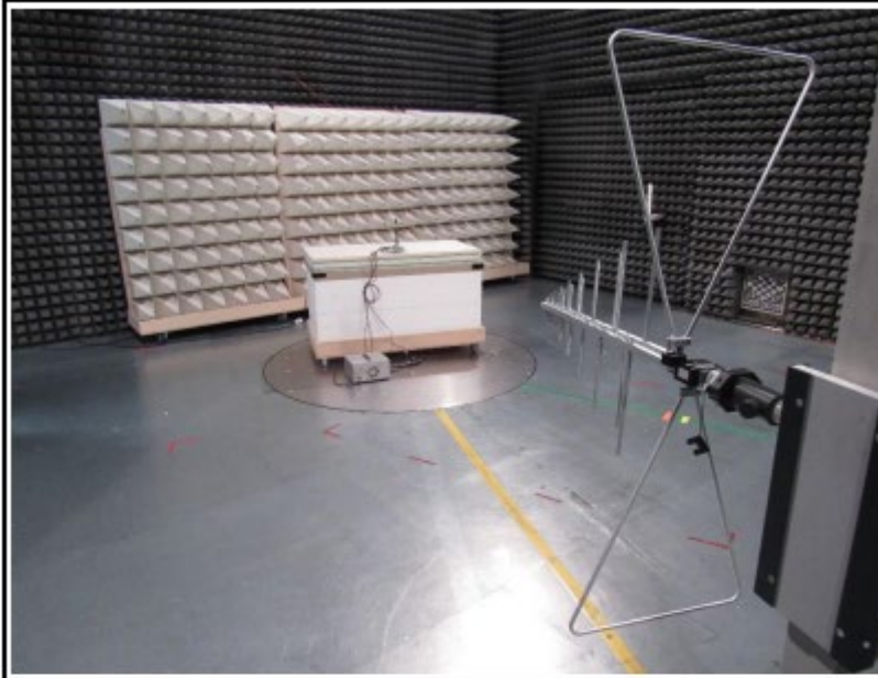
Setup for measurements below 1 GHz- Antenna 1
