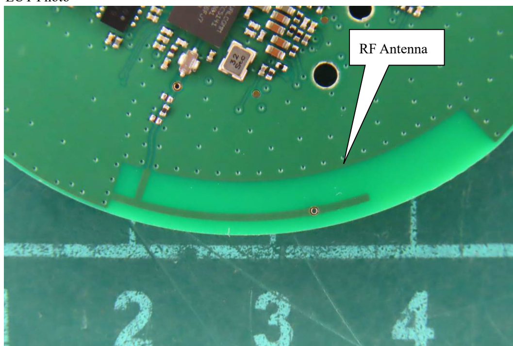
(32) EUT Photo
