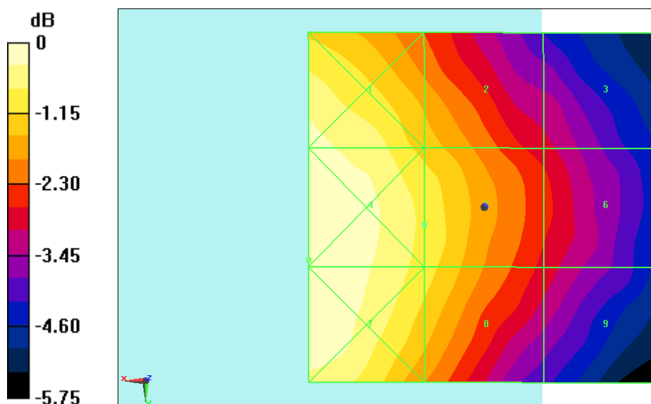
Fig B.4 HAC RF E-Field LTE Band41 QPSK PC3
