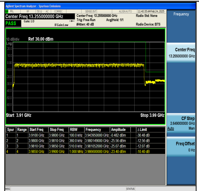
NTNV-n77(3700-3980)-PC2-30-70-H-CP-QPSK- Outer_Full-PASS
