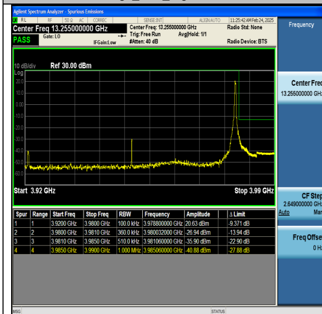
NTNV-n77(3700-3980)-PC2-30-60-H-CP-QPSK- Edge_1RB_Right-PASS
