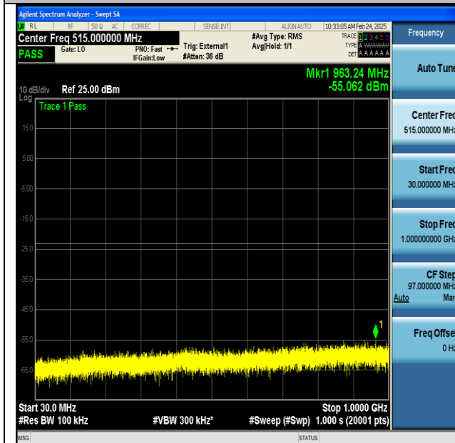
NTNV-n77(3700-3980)-PC2-30-100-H-CP-QPSK- Edge_1RB_Left-30-1000-PASS
