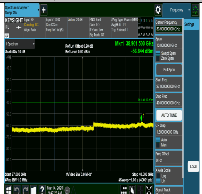
NTNV-n77(3700-3980)-PC2-30-100-M-DFT-BPSK- Edge_1RB_Left-27000-40000-PASS
