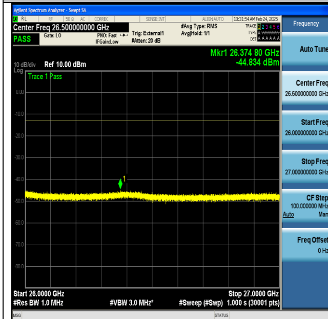
NTNV-n77(3700-3980)-PC2-30-100-H-DFT-BPSK- Edge_1RB_Left-26000-27000-PASS
