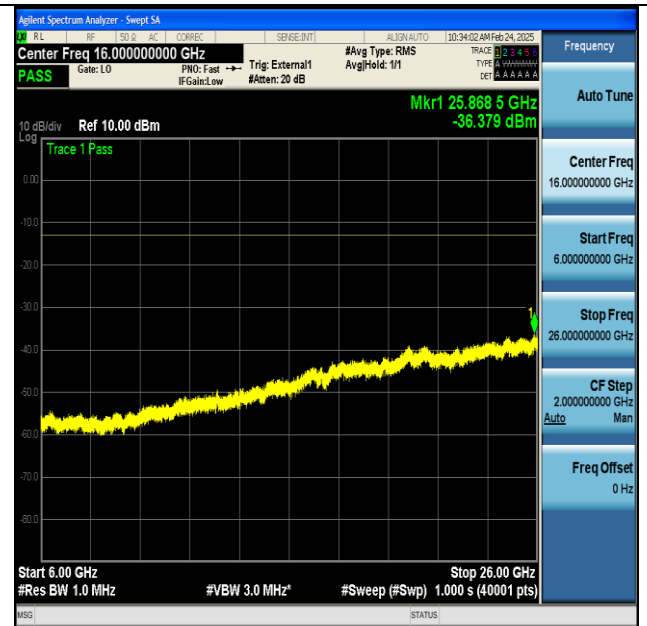
NTNV-n77(3700-3980)-PC2-30-100-H-CP-QPSK- Edge_1RB_Left-6000-26000-PASS
