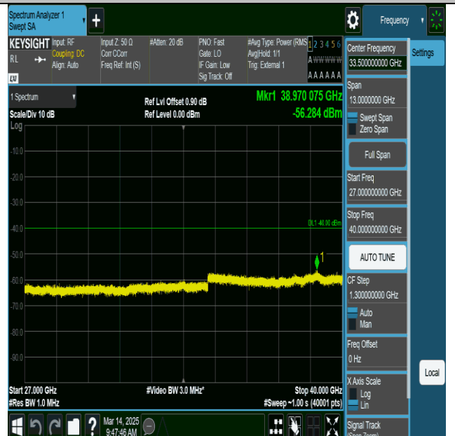
NTNV-n77(3700-3980)-PC2-30-100-M-CP-QPSK- Edge_1RB_Left-27000-40000-PASS
