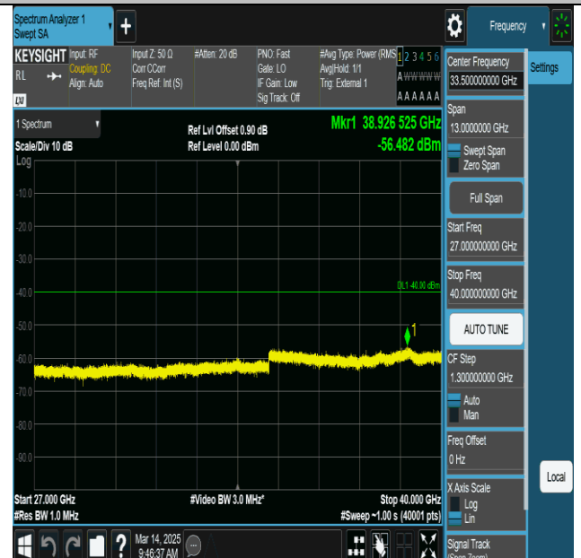
NTNV-n77(3700-3980)-PC2-30-100-L-DFT-BPSK- Edge_1RB_Left-27000-40000-PASS
