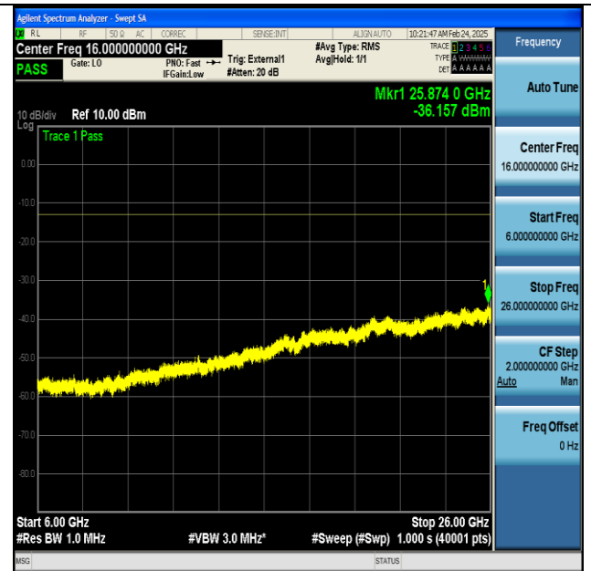
NTNV-n77(3700-3980)-PC2-30-100-L-DFT-BPSK- Edge_1RB_Left-6000-26000-PASS
