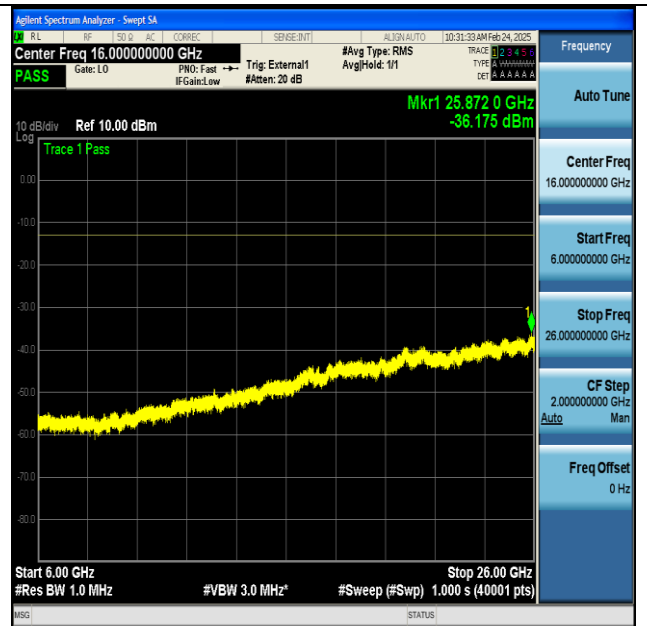
NTNV-n77(3700-3980)-PC2-30-100-H-DFT-BPSK- Edge_1RB_Left-6000-26000-PASS
