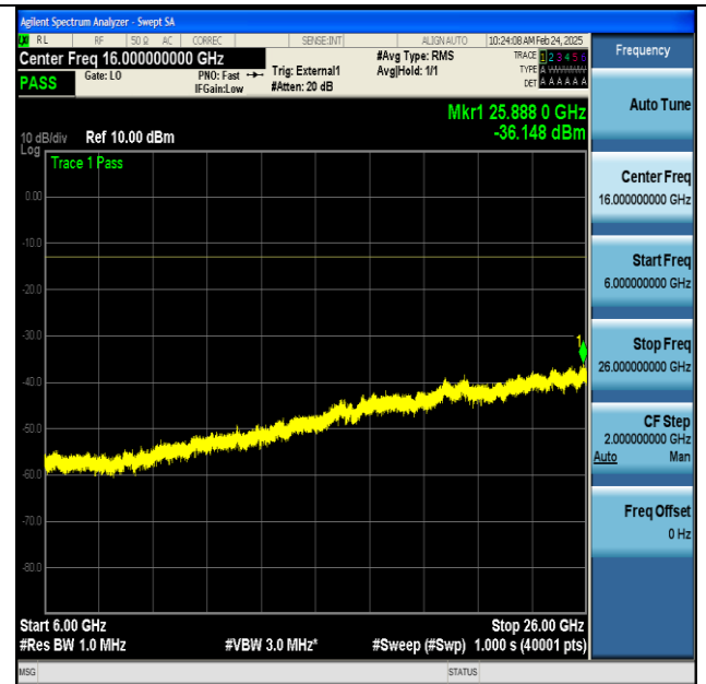
NTNV-n77(3700-3980)-PC2-30-100-L-CP-QPSK- Edge_1RB_Left-6000-26000-PASS
