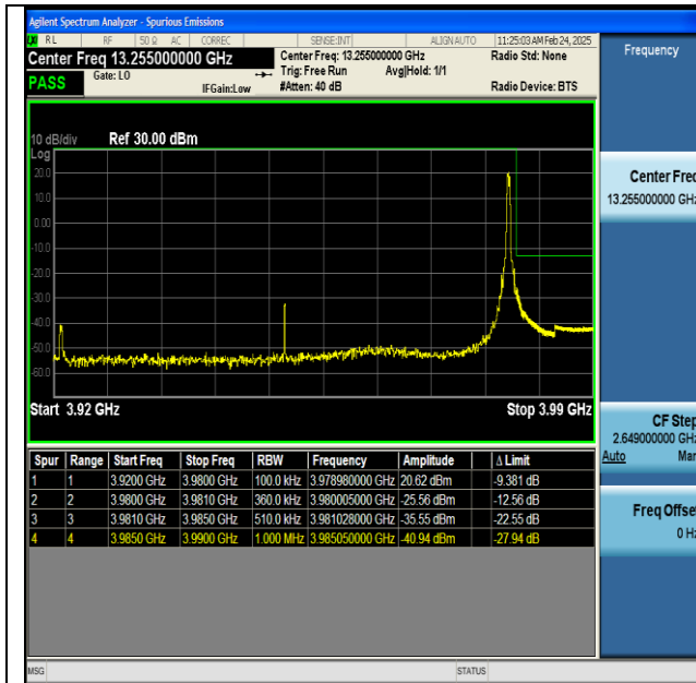
NTNV-n77(3700-3980)-PC2-30-60-H-DFT-BPSK- Edge_1RB_Right-PASS
