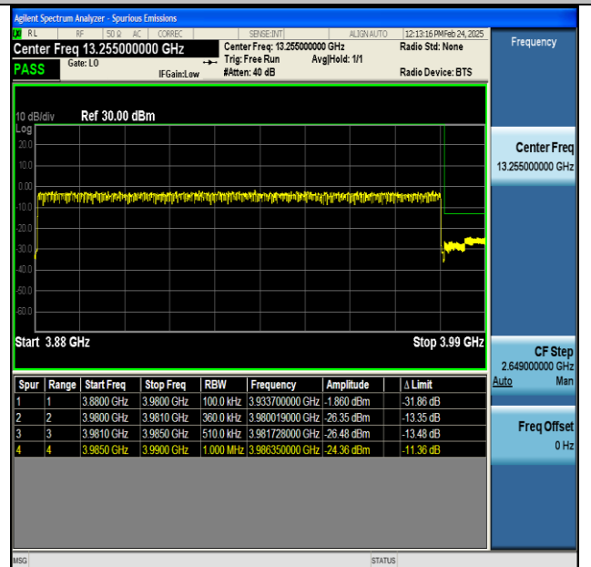
NTNV-n77(3700-3980)-PC2-30-100-H-CP-QPSK- Outer_Full-PASS
