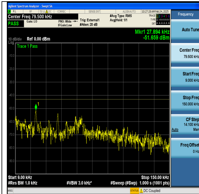
NTNV-n77(3700-3980)-PC2-30-100-M-CP-QPSK- Edge_1RB_Left-0.009-0.15-PASS
