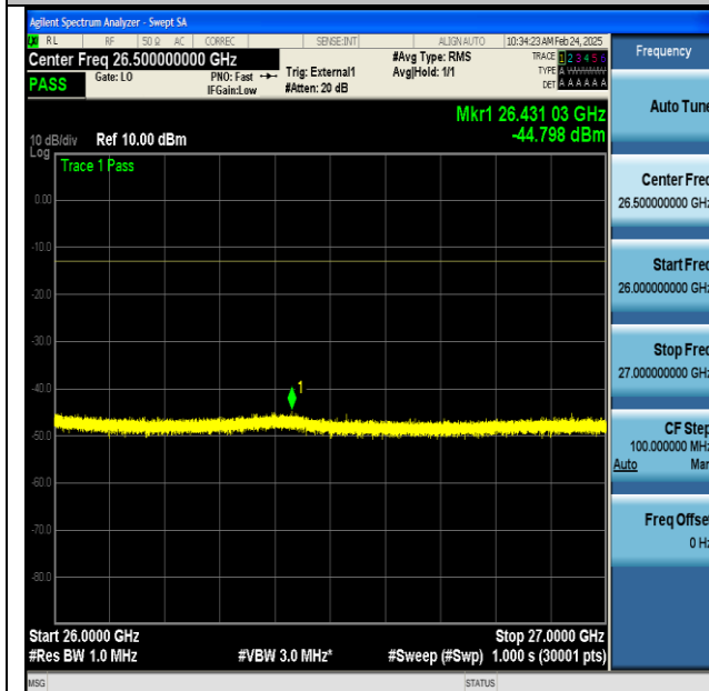
NTNV-n77(3700-3980)-PC2-30-100-H-CP-QPSK- Edge_1RB_Left-26000-27000-PASS
