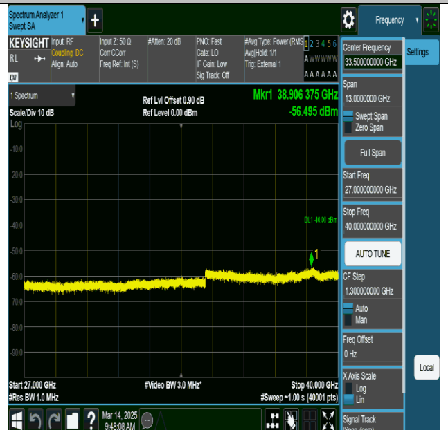
NTNV-n77(3700-3980)-PC2-30-100-H-DFT-BPSK- Edge_1RB_Left-27000-40000-PASS
