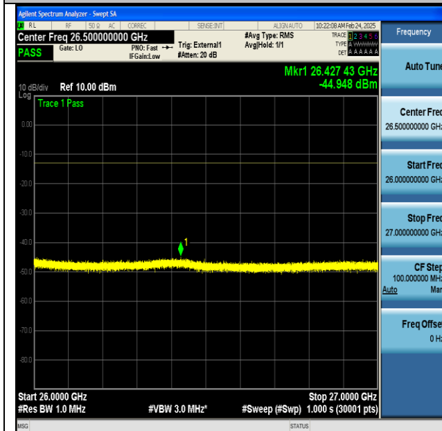
NTNV-n77(3700-3980)-PC2-30-100-L-DFT-BPSK- Edge_1RB_Left-26000-27000-PASS
