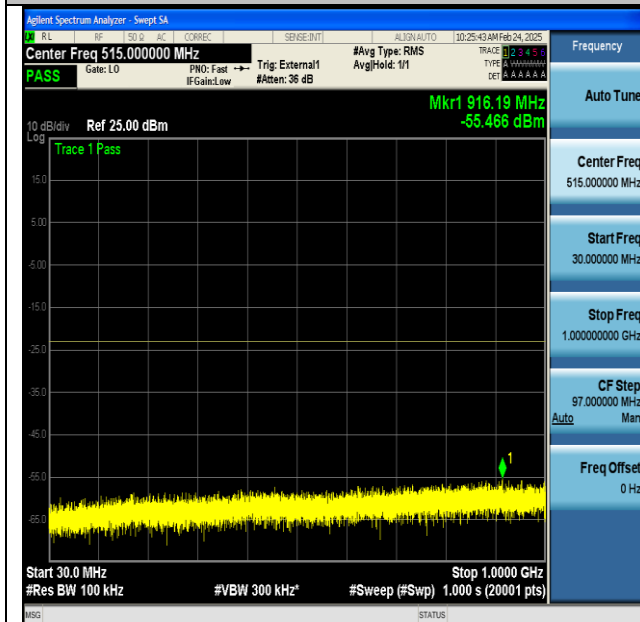
NTNV-n77(3700-3980)-PC2-30-100-M-DFT-BPSK- Edge_1RB_Left-30-1000-PASS
