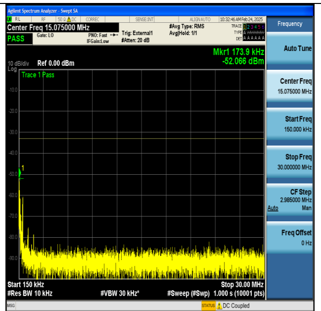
NTNV-n77(3700-3980)-PC2-30-100-H-CP-QPSK- Edge_1RB_Left-0.15-30-PASS
