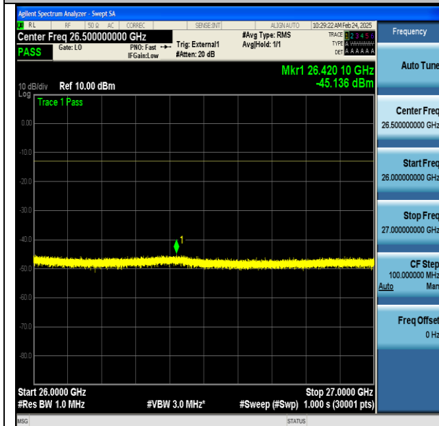
NTNV-n77(3700-3980)-PC2-30-100-M-CP-QPSK- Edge_1RB_Left-26000-27000-PASS
