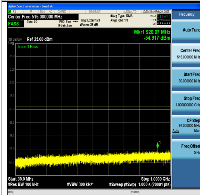
NTNV-n77(3700-3980)-PC2-30-100-H-DFT-BPSK- Edge_1RB_Left-30-1000-PASS
