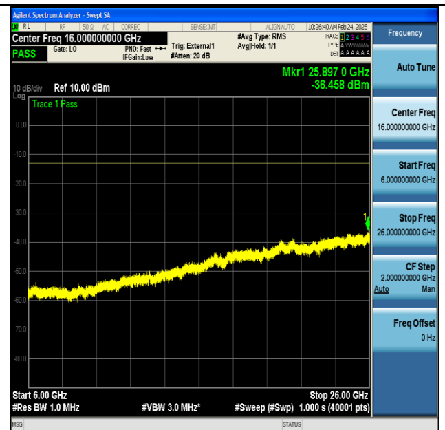
NTNV-n77(3700-3980)-PC2-30-100-M-DFT-BPSK- Edge_1RB_Left-6000-26000-PASS
