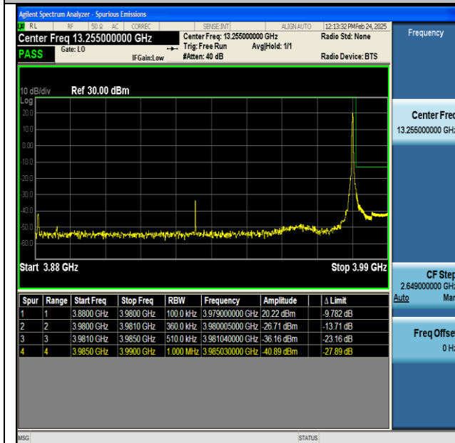
NTNV-n77(3700-3980)-PC2-30-100-H-CP-QPSK- Edge_1RB_Right-PASS
