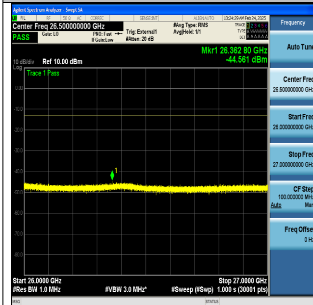
NTNV-n77(3700-3980)-PC2-30-100-L-CP-QPSK- Edge_1RB_Left-26000-27000-PASS
