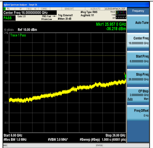
NTNV-n77(3700-3980)-PC2-30-100-M-CP-QPSK- Edge_1RB_Left-6000-26000-PASS
