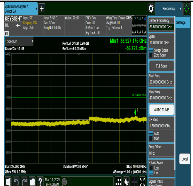
NTNV-n77(3700-3980)-PC2-30-100-L-CP-QPSK- Edge_1RB_Left-27000-40000-PASS
