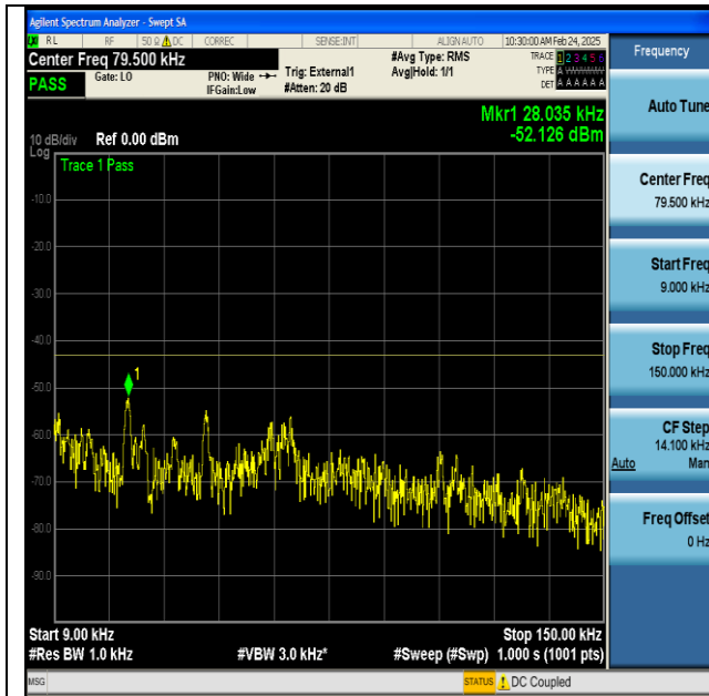
NTNV-n77(3700-3980)-PC2-30-100-H-DFT-BPSK- Edge_1RB_Left-0.009-0.15-PASS
