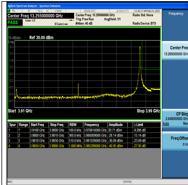
NTNV-n77(3700-3980)-PC2-30-70-H-DFT-BPSK- Edge_1RB_Right-PASS
