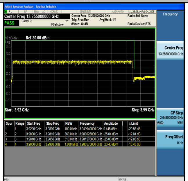
NTNV-n77(3700-3980)-PC2-30-60-H-CP-QPSK- Outer_Full-PASS
