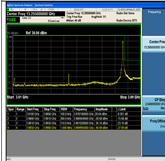
NTNV-n77(3700-3980)-PC2-30-70-H-CP-QPSK- Edge_1RB_Right-PASS
