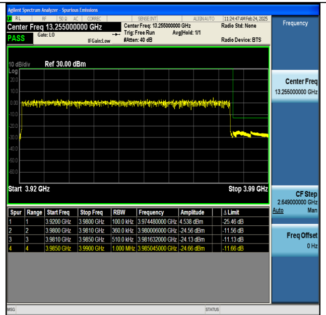
NTNV-n77(3700-3980)-PC2-30-60-H-DFT-BPSK- Outer_Full-PASS
