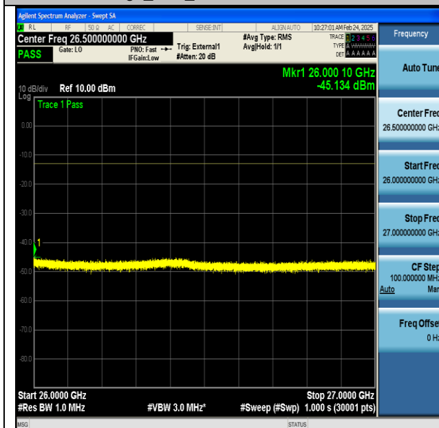
NTNV-n77(3700-3980)-PC2-30-100-M-DFT-BPSK- Edge_1RB_Left-26000-270000-PASS
