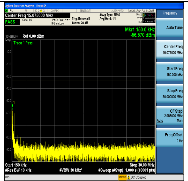
NTNV-n77(3700-3980)-PC2-30-100-H-DFT-BPSK- Edge_1RB_Left-0.15-30-PASS
