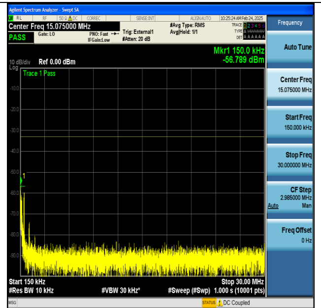
NTNV-n77(3700-3980)-PC2-30-100-M-DFT-BPSK- Edge_1RB_Left-0.15-30-PASS
