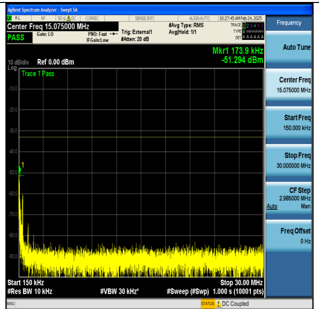
NTNV-n77(3700-3980)-PC2-30-100-M-CP-QPSK- Edge_1RB_Left-0.15-30-PASS
