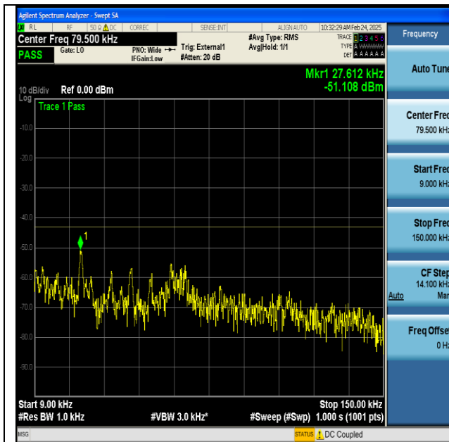
NTNV-n77(3700-3980)-PC2-30-100-H-CP-QPSK- Edge_1RB_Left-0.009-0.15-PASS
