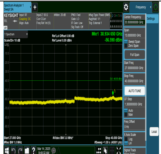
NTNV-n77(3700-3980)-PC2-30-100-H-CP-QPSK- Edge_1RB_Left-27000-40000-PASS
