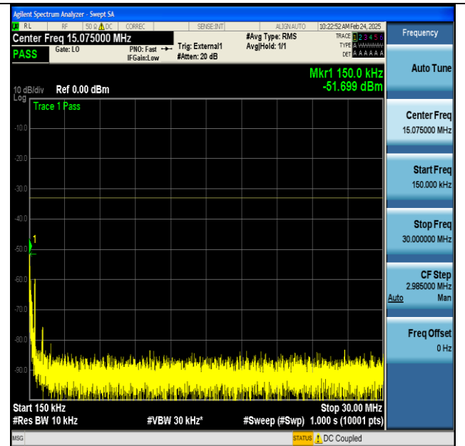
NTNV-n77(3700-3980)-PC2-30-100-L-CP-QPSK- Edge_1RB_Left-0.15-30-PASS
