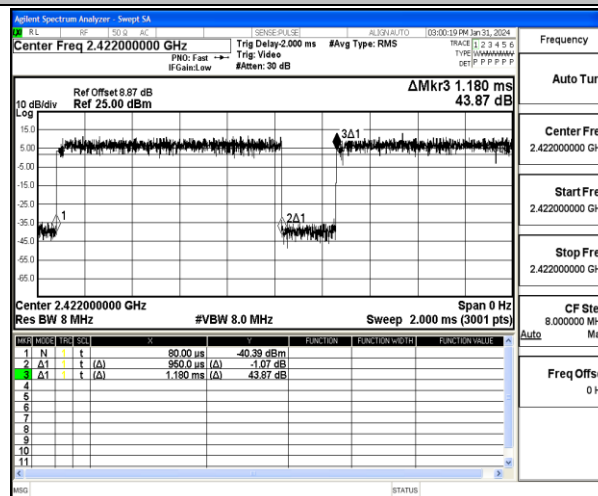
NTNV-11N40MIMO-Ant2-2422
