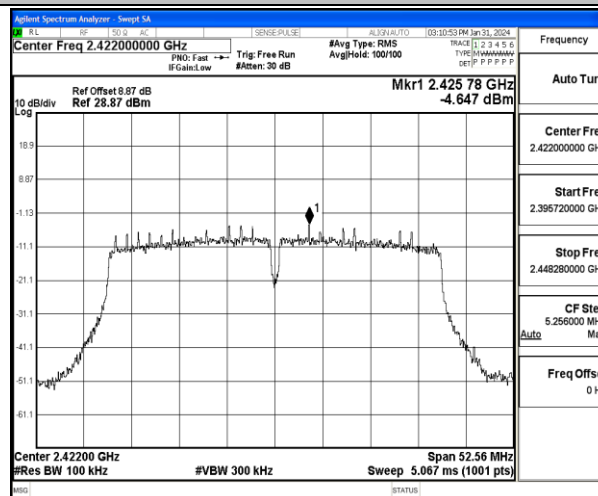
11N40MIMO-Ant2-2422-PASS
