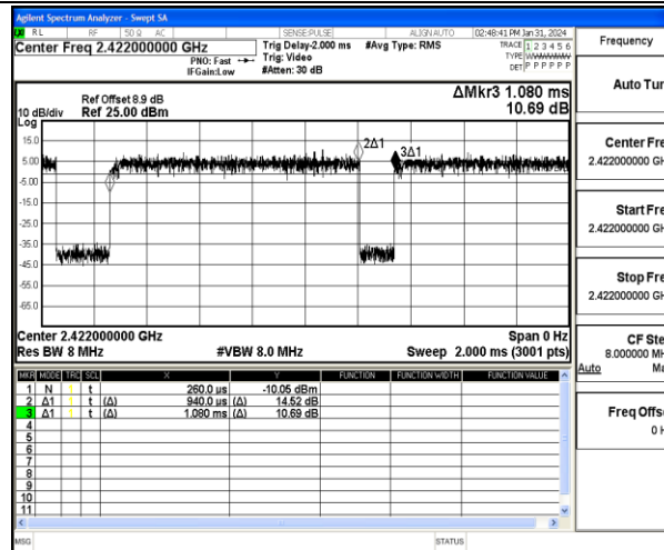
NTNV-11N40MIMO-Ant1-2422
