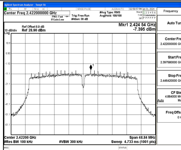
11N40MIMO-Ant1-2422-PASS
