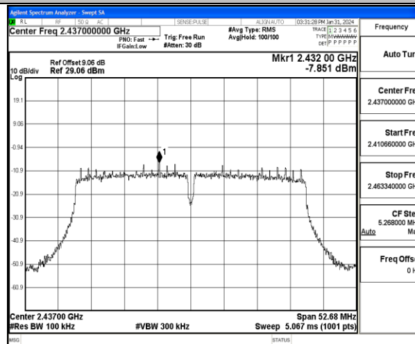
11N40MIMO-Ant1-2437-PASS
