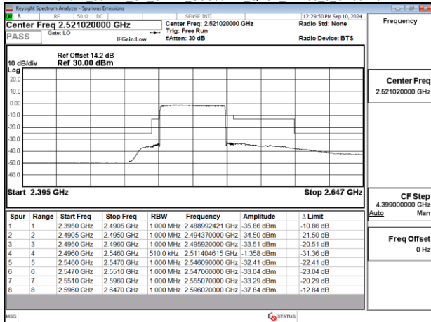
Band41_50MHz_CP_OFDM_SCS30kHz_QPSK_RB133_0_CH505002
