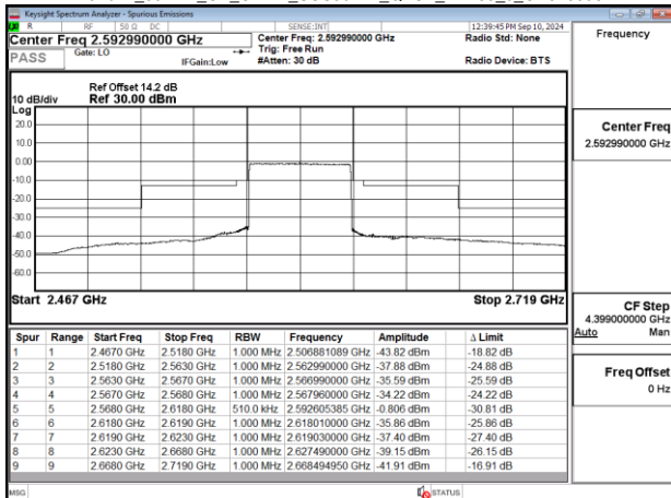
Band41_50MHz_CP_OFDM_SCS30kHz_QPSK_RB133_0_CH518598
