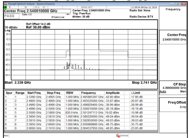
Band41_80MHz_DFT_s_OFDM_SCS30kHz_BPSK_RB1_0_CH508002
