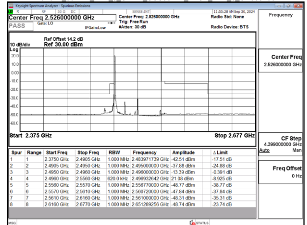
Band41_60MHz_DFT_s_OFDM_SCS30kHz_BPSK_RB1_0_CH506004
