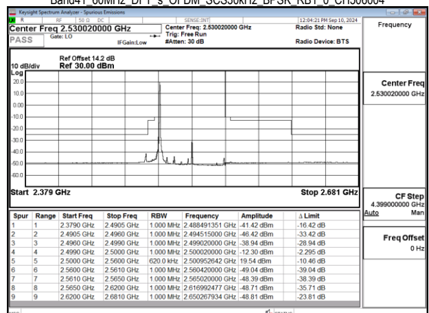
Band41_60MHz_DFT_s_OFDM_SCS30kHz_BPSK_RB1_0_CH506004
