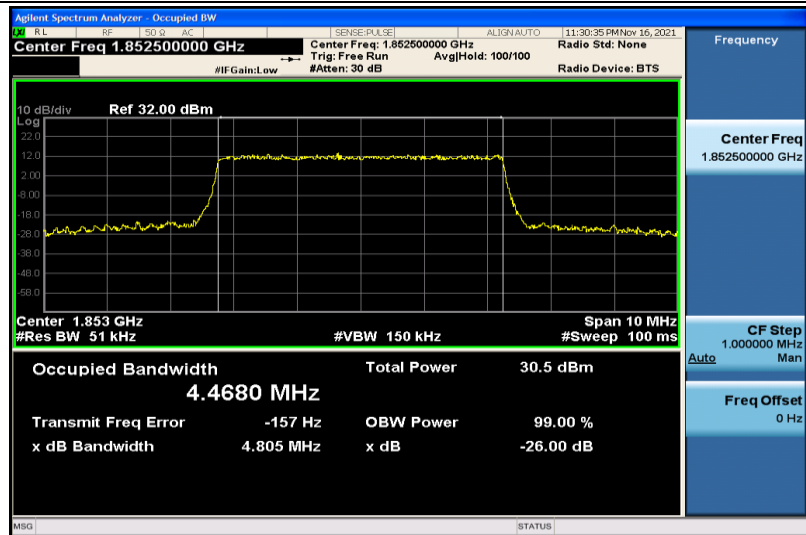
Band2-5MHz-QPSK-18625-25RB#0-4.4680
