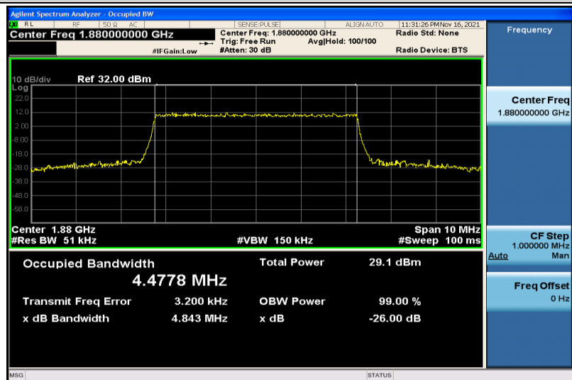
Band2-5MHz-16QAM-18900-25RB#0-4.4778
