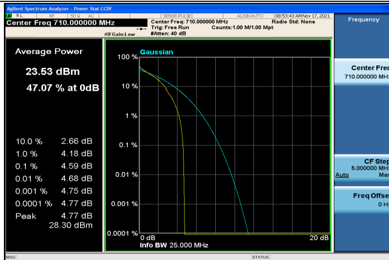
Band17-10MHz-QPSK-23790-1RB#0
