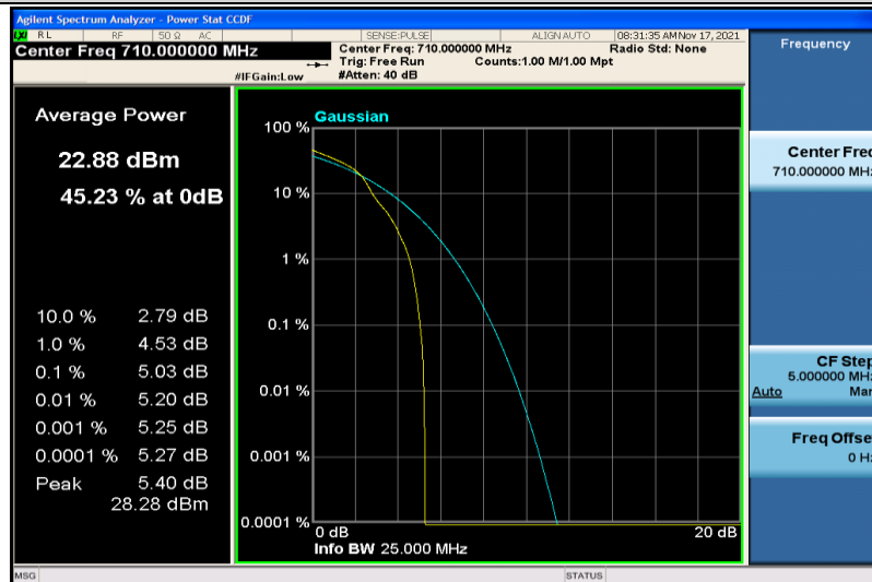
Band17-5MHz-16QAM-23790-1RB#0
