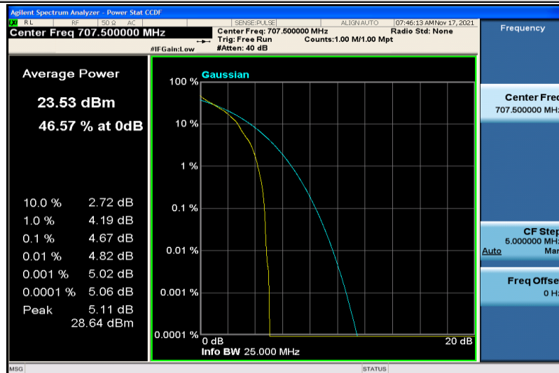
Band12-5MHz-QPSK-23095-1RB#0
