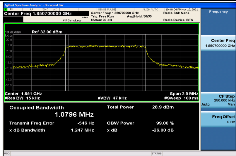
Band2-1.4MHz-16QAM-18607-6RB#0-1.0796
