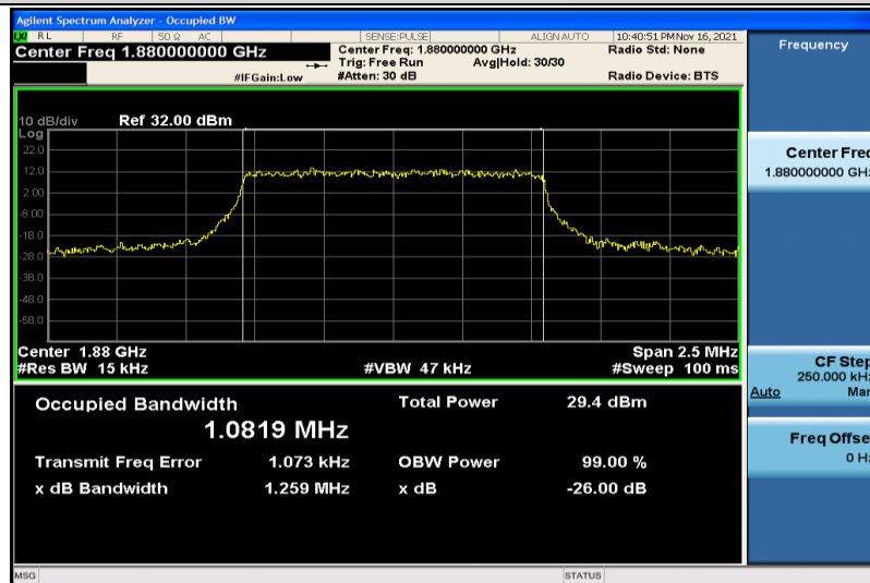
Band2-1.4MHz-QPSK-18900-6RB#0-1.0819
