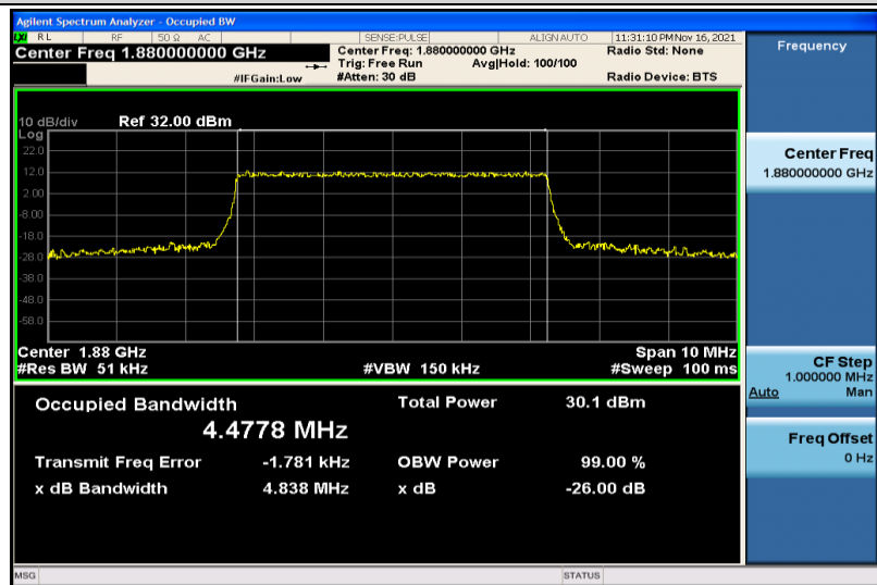
Band2-5MHz-QPSK-18900-25RB#0-4.4778
