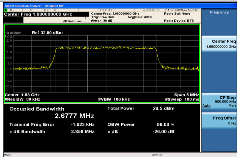
Band2-3MHz-16QAM-18900-15RB#0-2.6777
