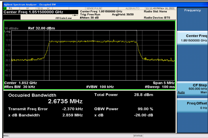
Band2-3MHz-16QAM-18615-15RB#0-2.6735
