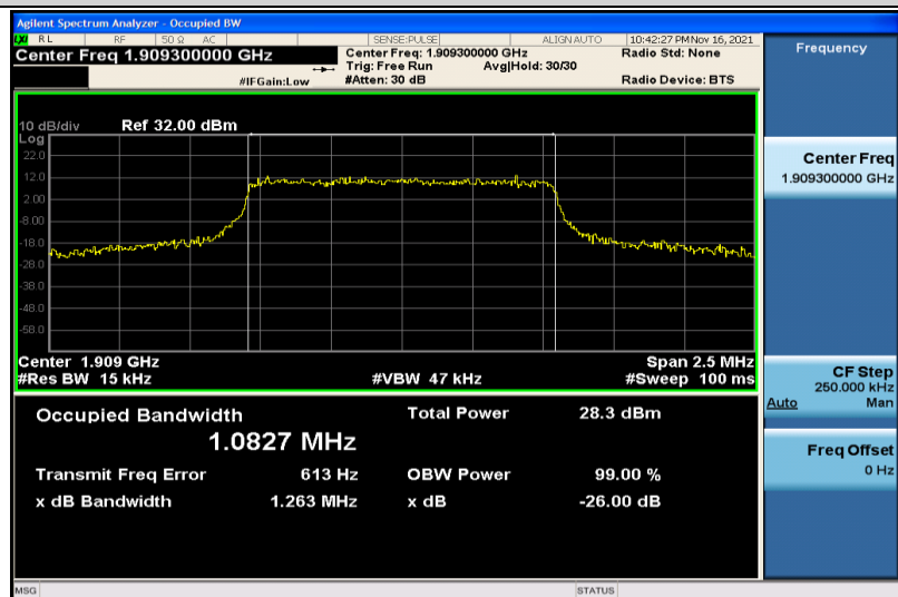
Band2-1.4MHz-16QAM-19193-6RB#0-1.0827
