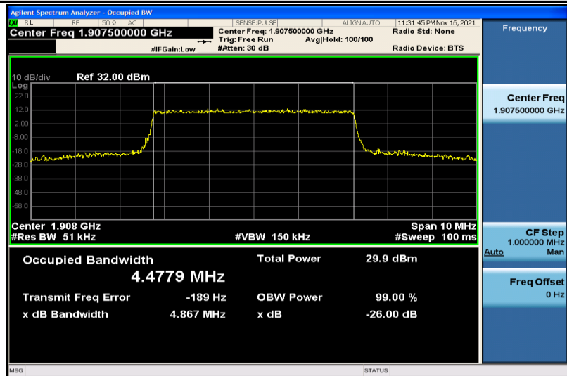
Band2-5MHz-QPSK-19175-25RB#0-4.4779
