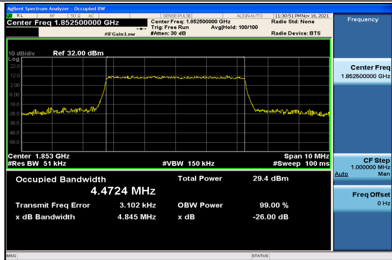
Band2-5MHz-16QAM-18625-25RB#0-4.4724
