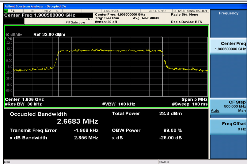
Band2-3MHz-16QAM-19185-15RB#0-2.6683
