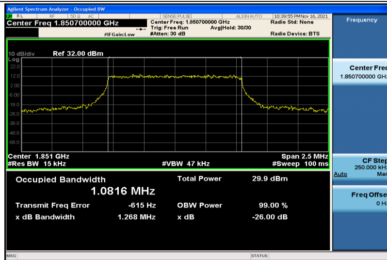
Band2-1.4MHz-QPSK-18607-6RB#0-1.0816
