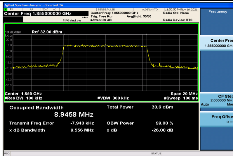
Band2-10MHz-QPSK-18650-50RB#0-8.9458
