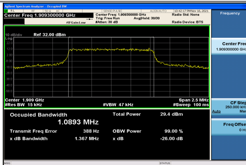
Band2-1.4MHz-QPSK-19193-6RB#0-1.0893
