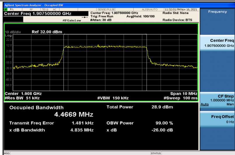
Band2-5MHz-16QAM-19175-25RB#0-4.4669
