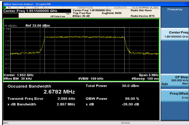
Band2-3MHz-QPSK-18615-15RB#0-2.6782
