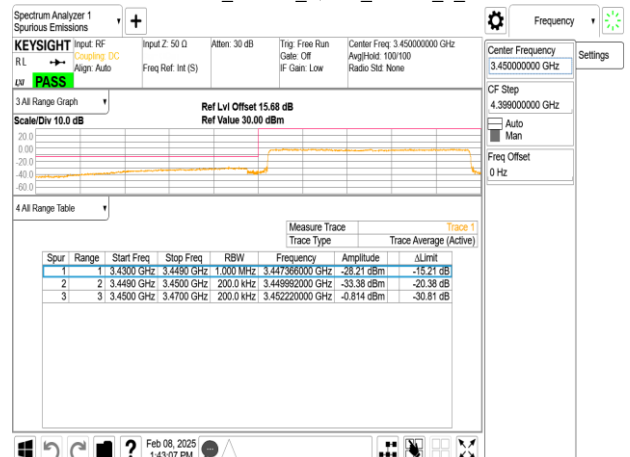
Band42-Part27_20MHz_QPSK_RB100_0_CH42190
