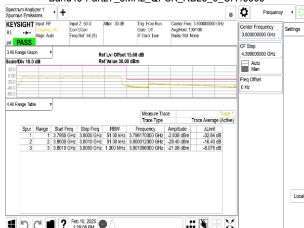
Band43-Part27_5MHz_QPSK_RB25_0_CH45565
