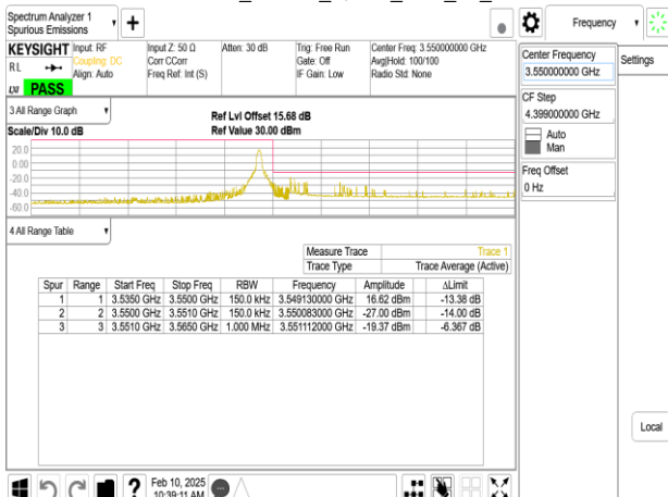
Band42-Part27_15MHz_QPSK_RB1_74_CH43015
