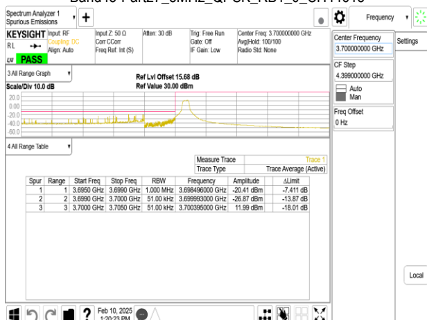
Band43-Part27_5MHz_QPSK_RB1_0_CH44615
