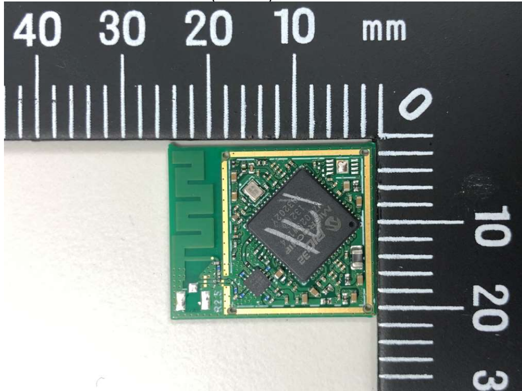
Internal Photo of WFI32E01PE (Module with PCB Antenna) (Reference)
