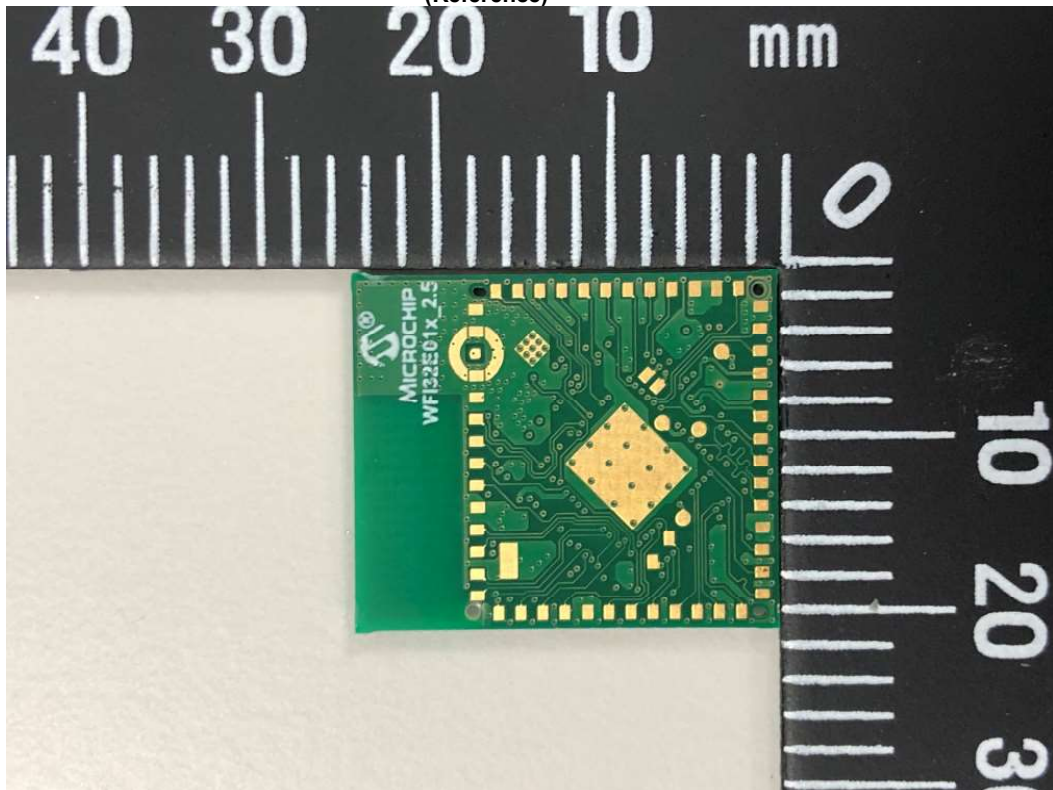
Internal Photo of WFI32E01PC (Module with PCB Antenna and Trust&GO) (Reference)
