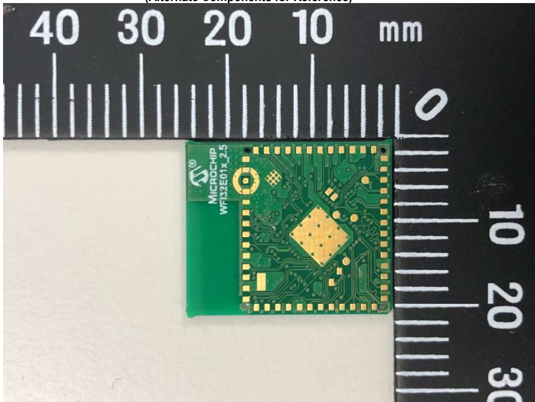
Internal Photo of WFI32E01PE (Module with PCB Antenna) (Alternate Components for Reference)
