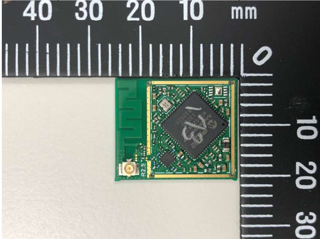
Internal Photo of WFI32E01UE (Module with u.FL Connector for External Antenna)
