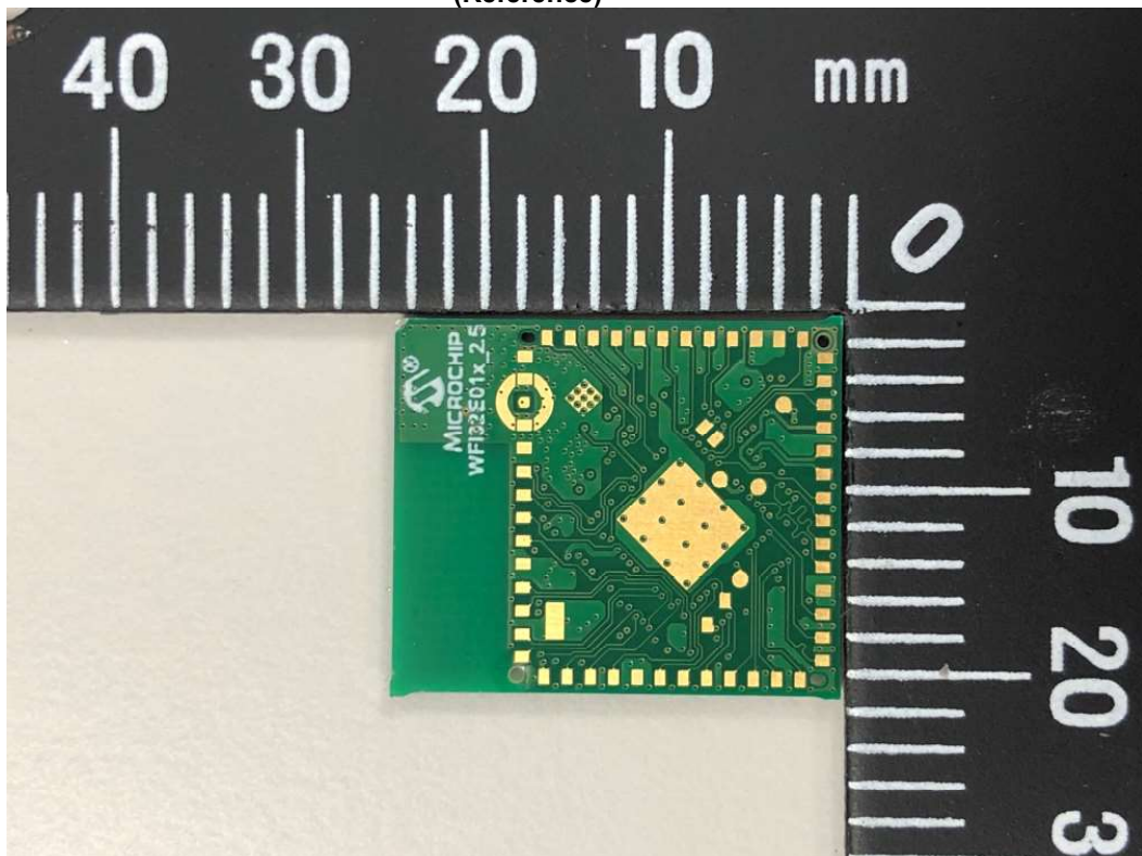
Internal Photo of WFI32E01PC (Module with PCB Antenna and Trust&GO) (Alternate Components) (Reference)
