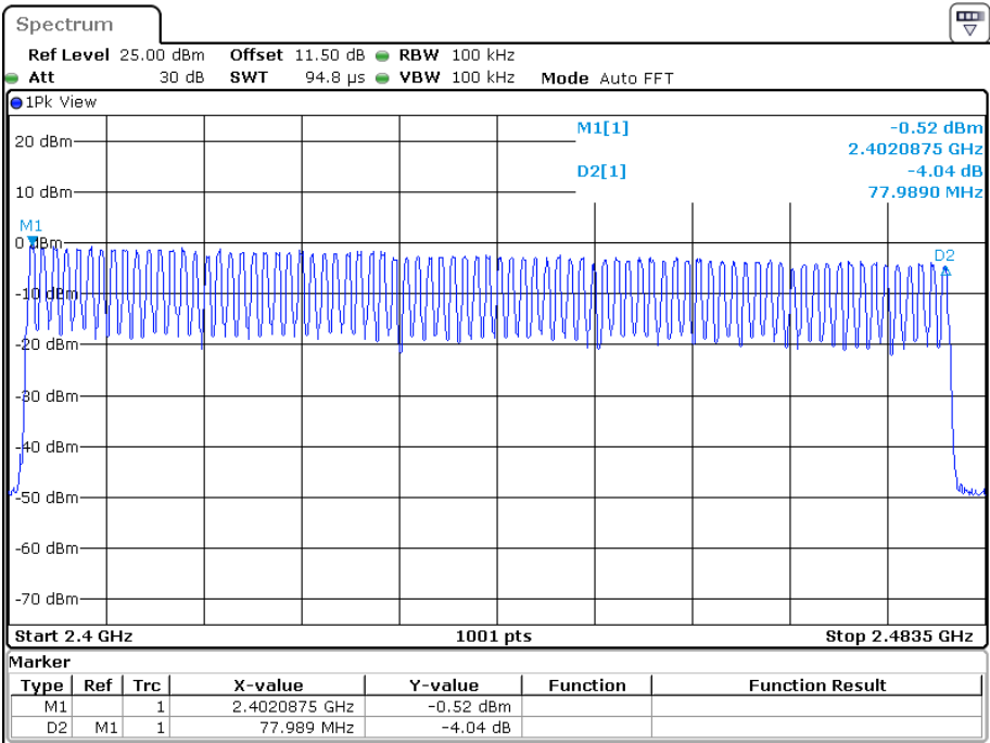
BDR (GFSK): Number of Hopping Channels
